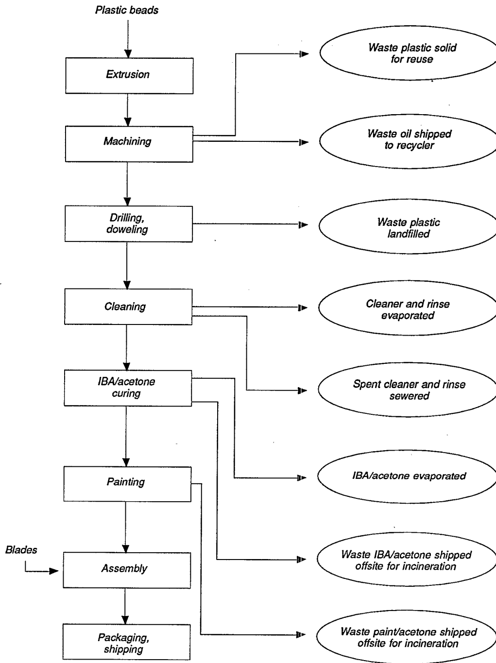
Figure 1. Abbreviated process flow diagram that describes the waste generation in this plant.
