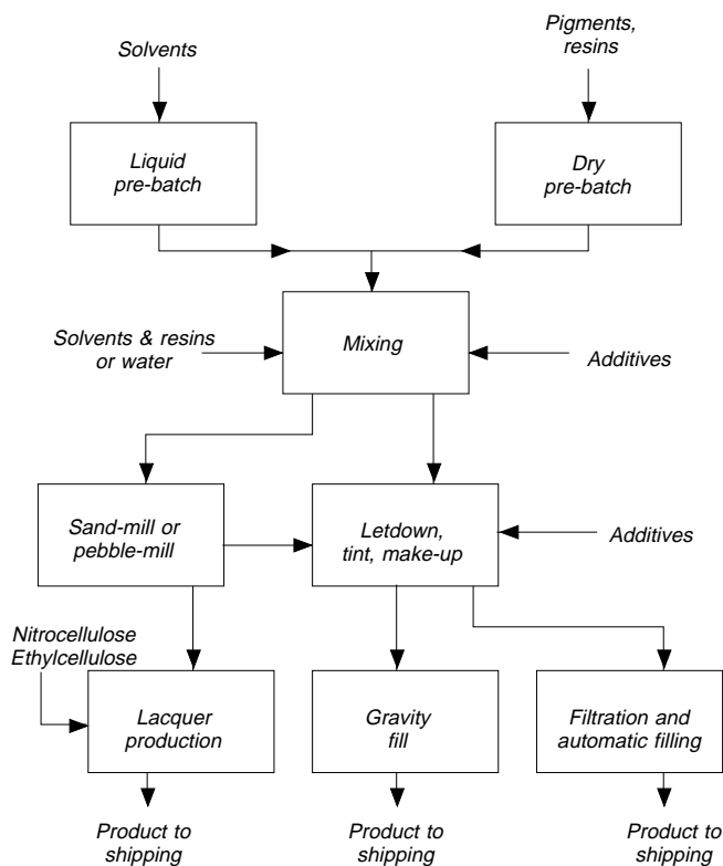
Figure 1. Abbreviated process flow diagram.
