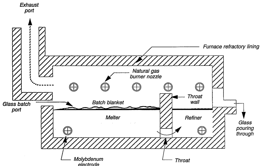
Figure 1. Ek Glassification™ test furnace for EAF dust.
