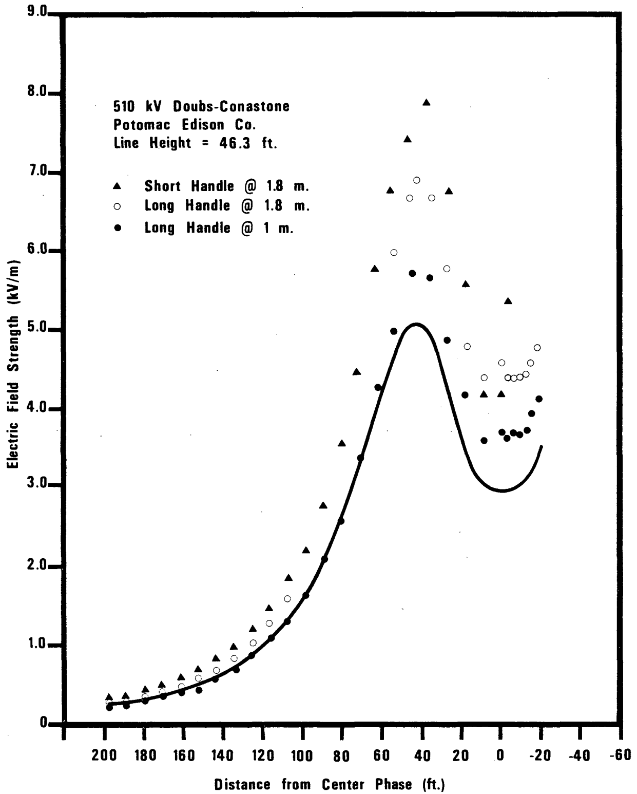
FIGURE 2. ELECTRIC FIELD STRENGTH PROFILES USING A MONROE ELECTRONICS MODEL 238A-1
