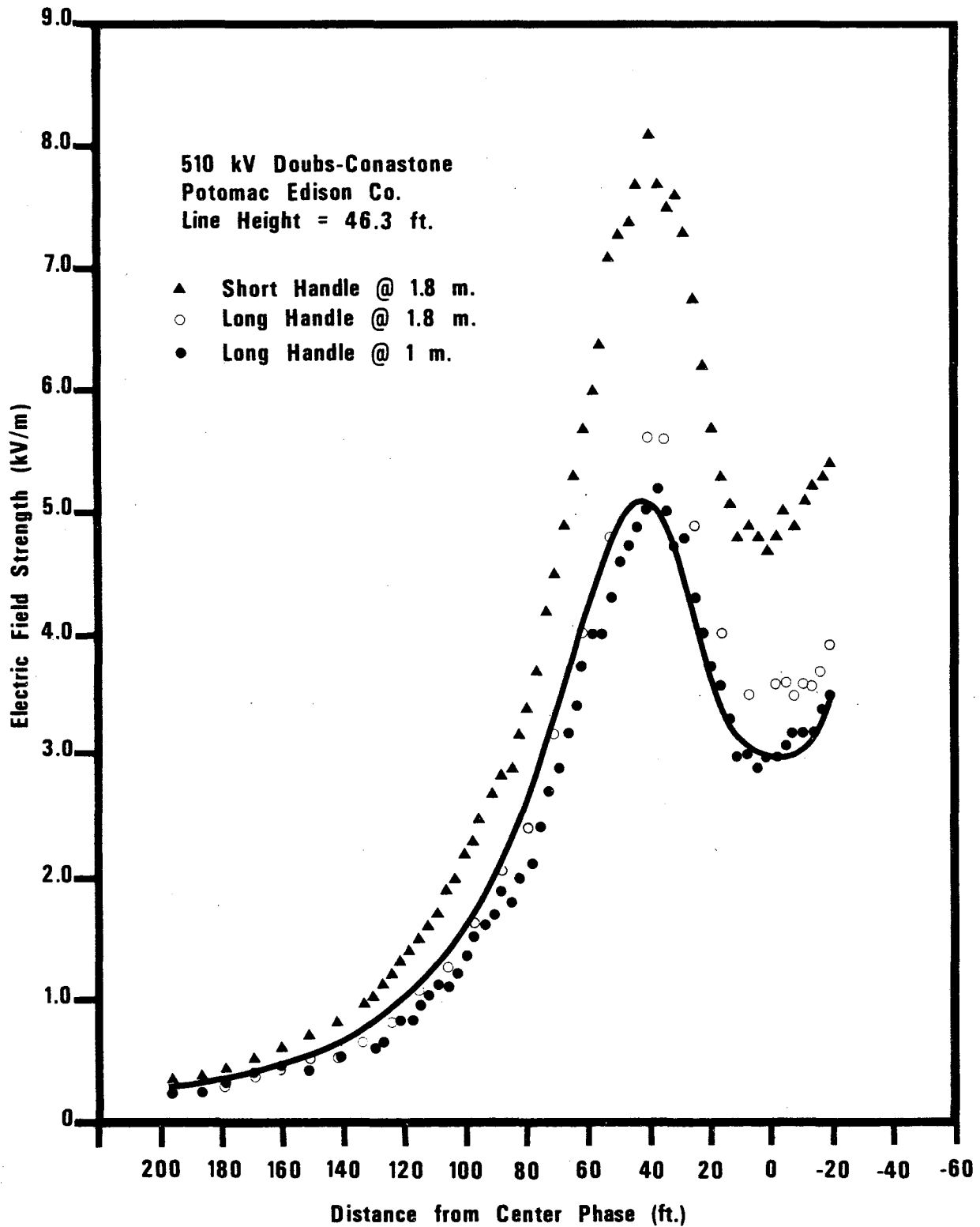
FIGURE 1. ELECTRIC FIELD STRENGTH PROFILES USING A POLYTECH FBM-100
