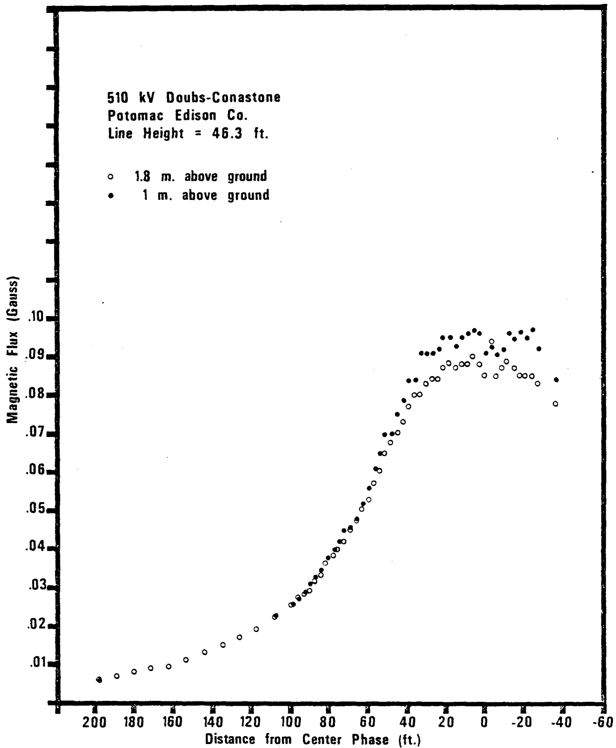
FIGURE 3. MAGNETIC FLUX PROFILE
