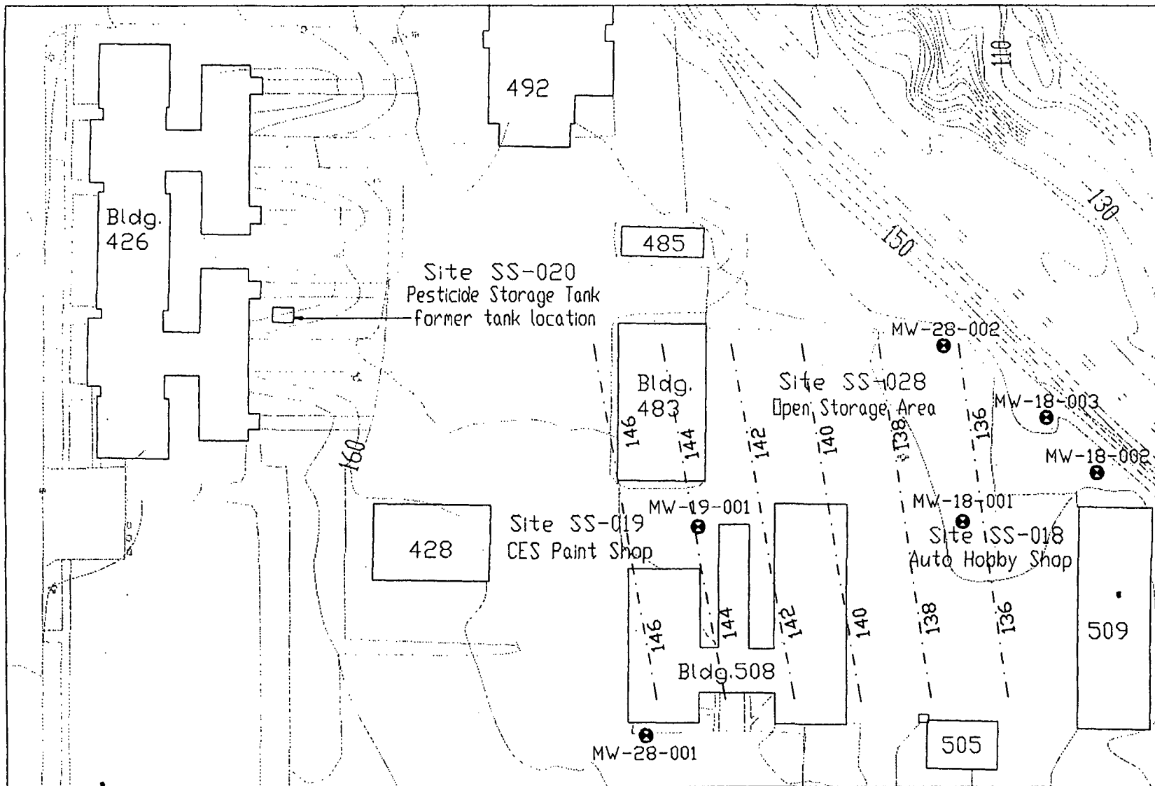
Figure 3 Groundwater Contours and Site Features --- Groundwater Contours From Malcolm Pinnie Site Investigation Jan 94
