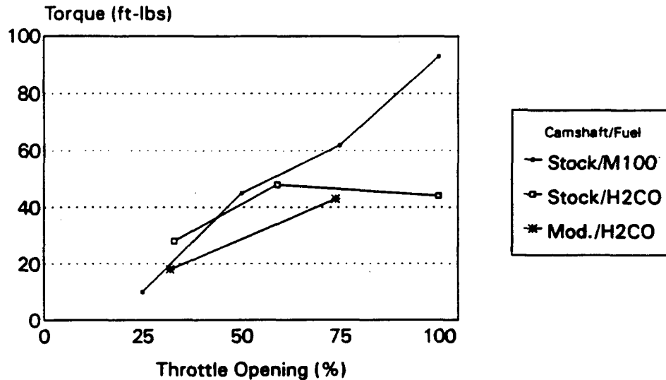
Figure 3 Brake Specific Torque Values Lambda = 0.7*, 1500 rpm Operating Conditions
