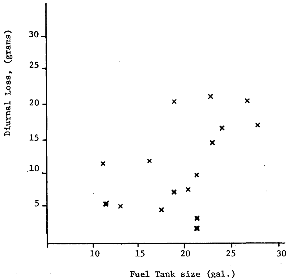
Figure 14 Diurnal Loss vs. Fuel tank volume for the L.A. FY 72 surveillance program.
