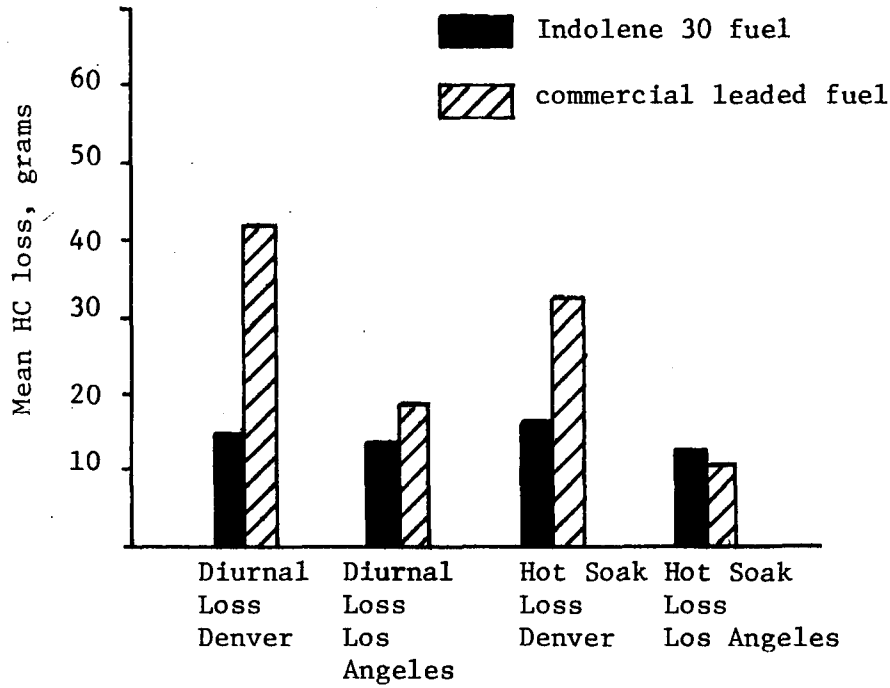
Figure 3 Mean HC loss for Indolene or Commercial Leded Fuels for Denver and Los Angeles.
