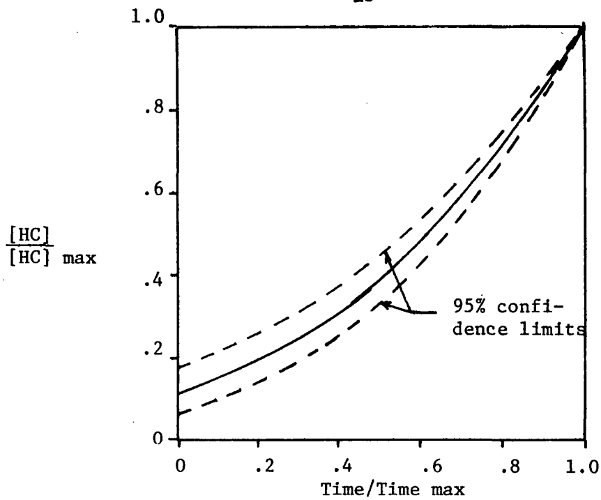
Figure 10 \frac{[HC]}{[HC] \text{ max}} vs. \frac{\text{Time}}{\text{Time max}} for diurnal tests conducted during the Denver FY 73 surveillance program.
