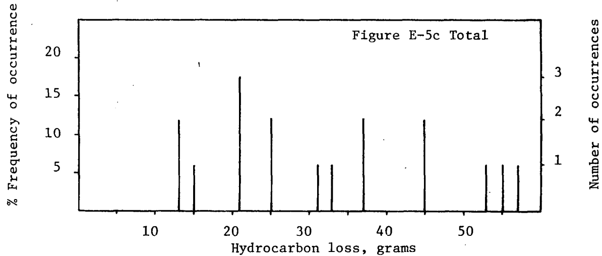
Figure E-5 Histograms of Diurnal, Hot Soak, and Total loss data for Denver FY 73 program.
