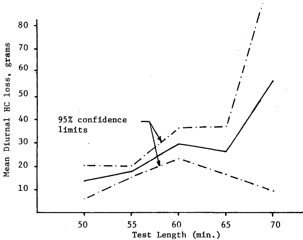
Figure 11 Mean diurnal HC loss vs. length of test for Denver FY 71 data only. (All tests ended at 84^{\circ}\text{F} \pm .5^{\circ}\text{F} )
