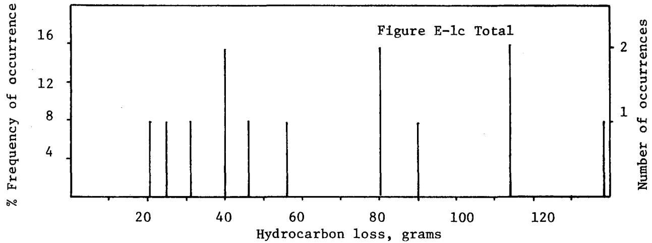
Figure E-1 Histograms of Diurnal, Hot Soak, and Total loss data for Denver FY71 program.
