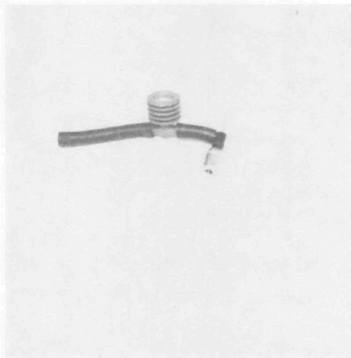
New PCV valve, device, and PCV hose unit used to replace the original PCV valve and hose.
