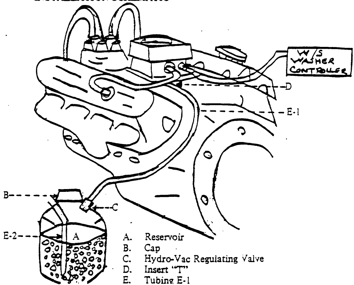
HYDRO VAC SYSTEM INSTALLATION SCHEMATIC
