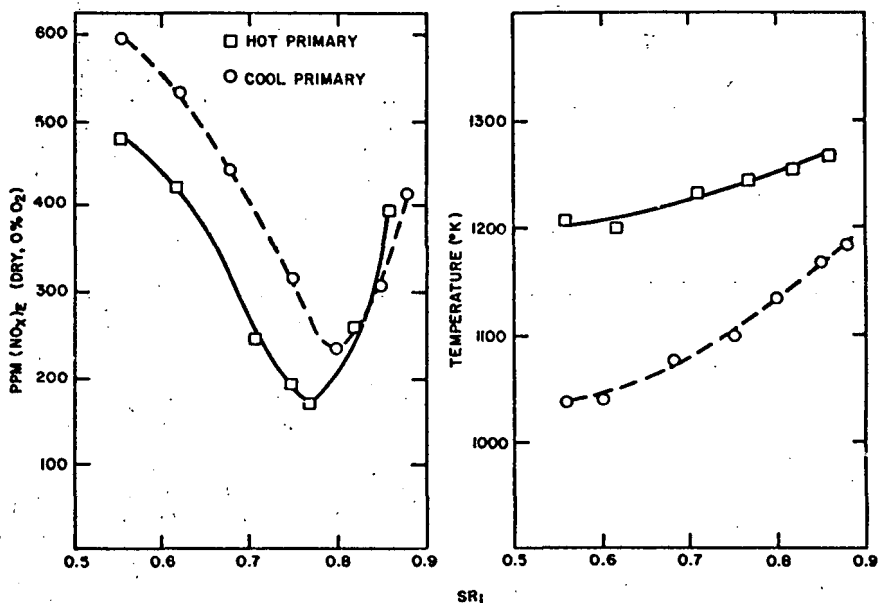
FIG. 8. The influence of fuel-rich hold-up zone temperature profile on exhaust NO x .
