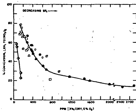
FIG. 7. Conversion of TFN to exhaust \text{NO}_x ( 0.5 \leq \text{SR}_1 \leq 0.8 ).
