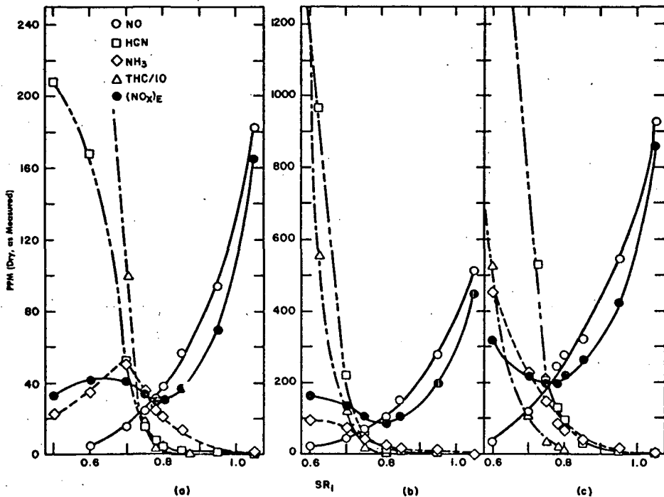
FIG. 3. NO, HCN, and \text{NH}_3 production in the fuel-rich hold-up zone for (a) D1-Alaskan diesel oil, (b) R9-Alaskan bunker C oil, and (c) A9-SRC-II heavy distillate oil (3% overall excess oxygen).
