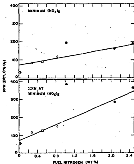
FIG. 6. The effect of fuel-bound nitrogen content on exhaust \text{NO}_x and TFN in the primary zone ( \Sigma\text{XN}_1 ) ( \text{SR}_1 = 0.78 , 3% overall excess \text{O}_2 ).
