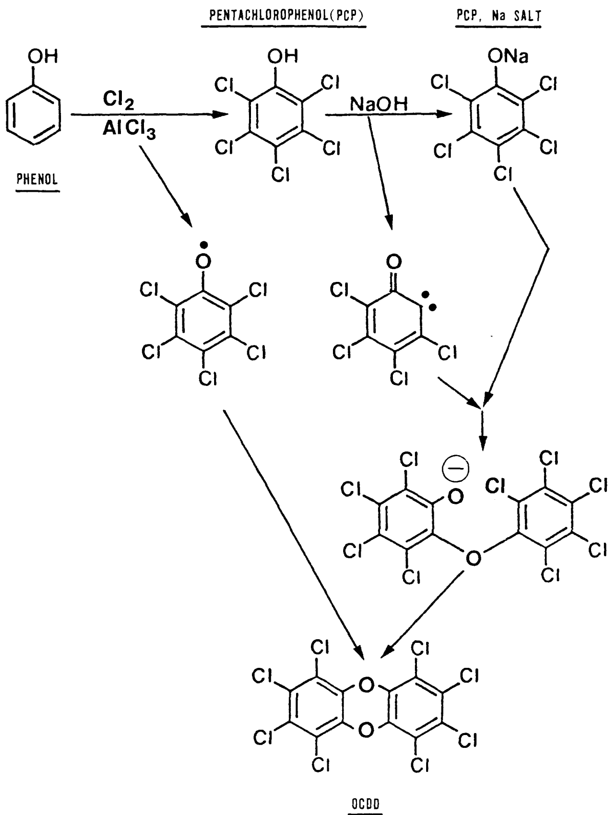
Figure 23. Pentachlorophenol (PCP) via phenol.
