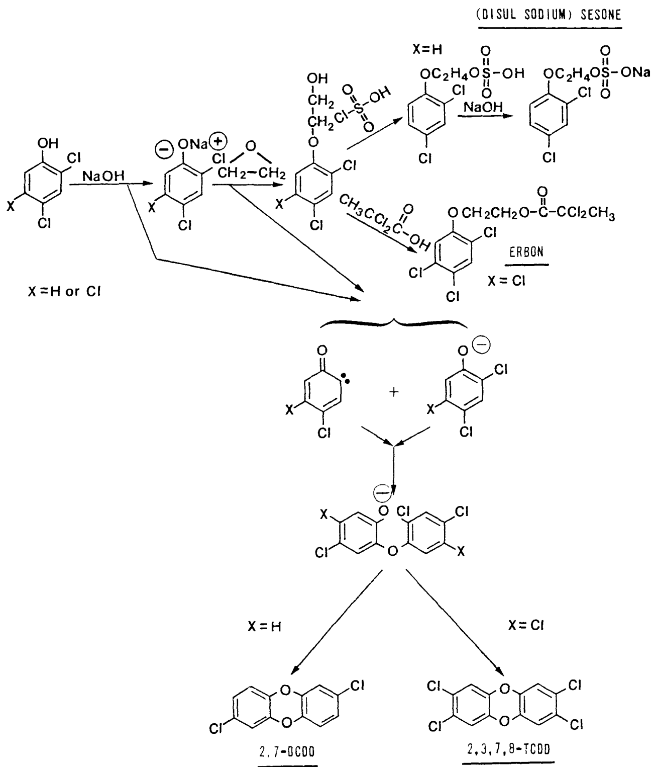
Figure 15. Erbon and Sesone.
