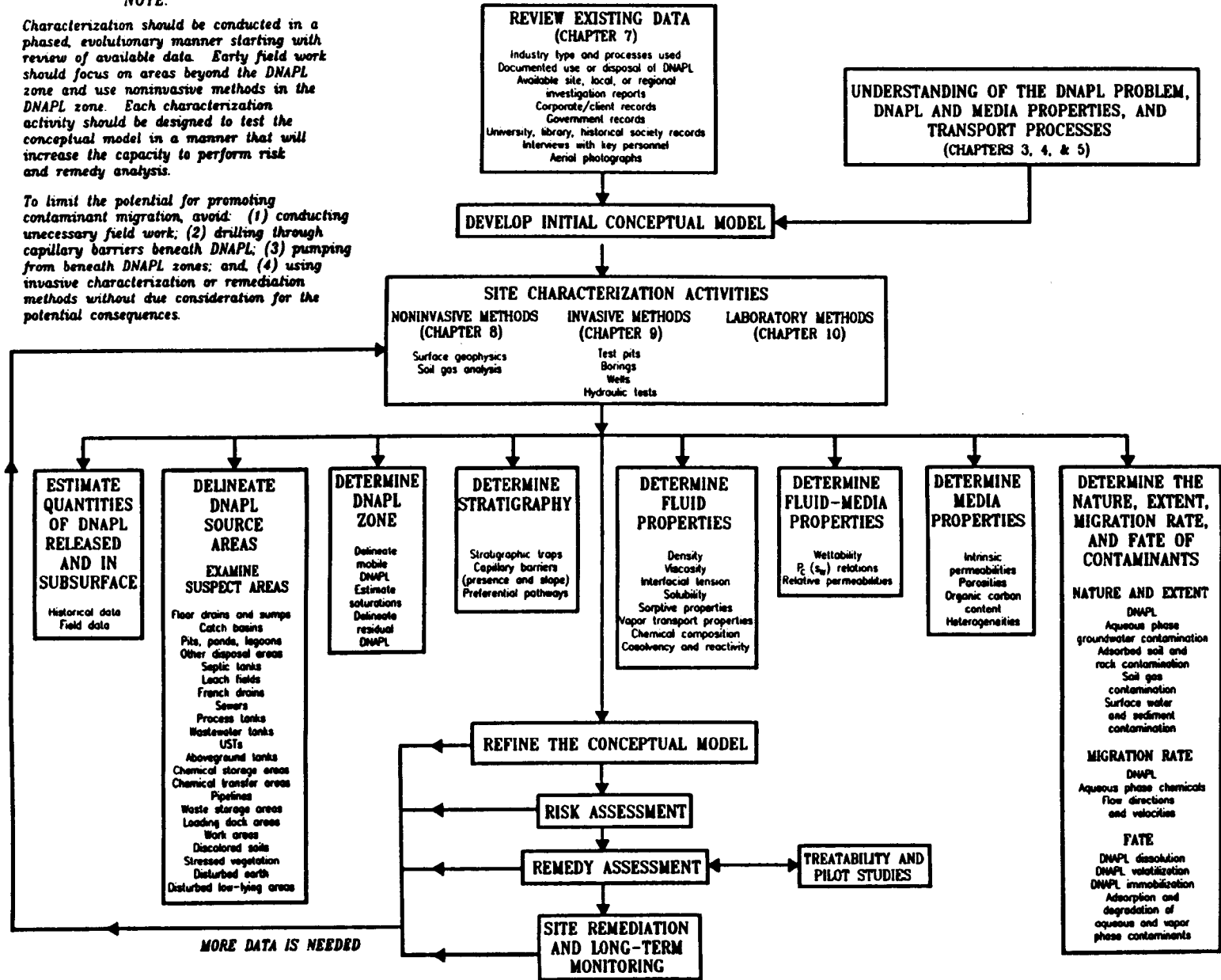
Figure 1. DNAPL site characterization flowchart (modified from Cohen and Mercer, 1993).
