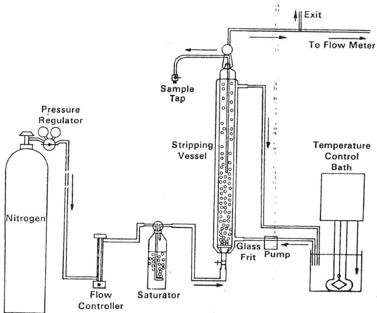
Figure 1. Stripping apparatus diagram
