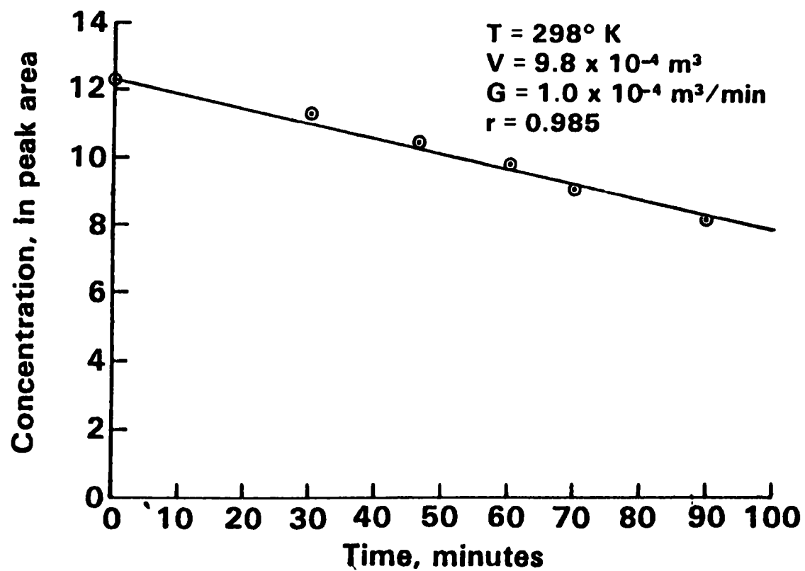
Figure 3. Typical plot for volatilization of trichloroethylene
