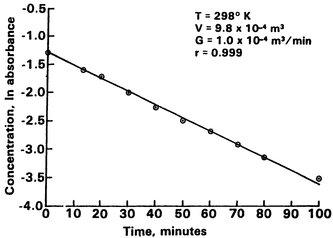
Figure 4. Typical plot for volatilization of benzene
