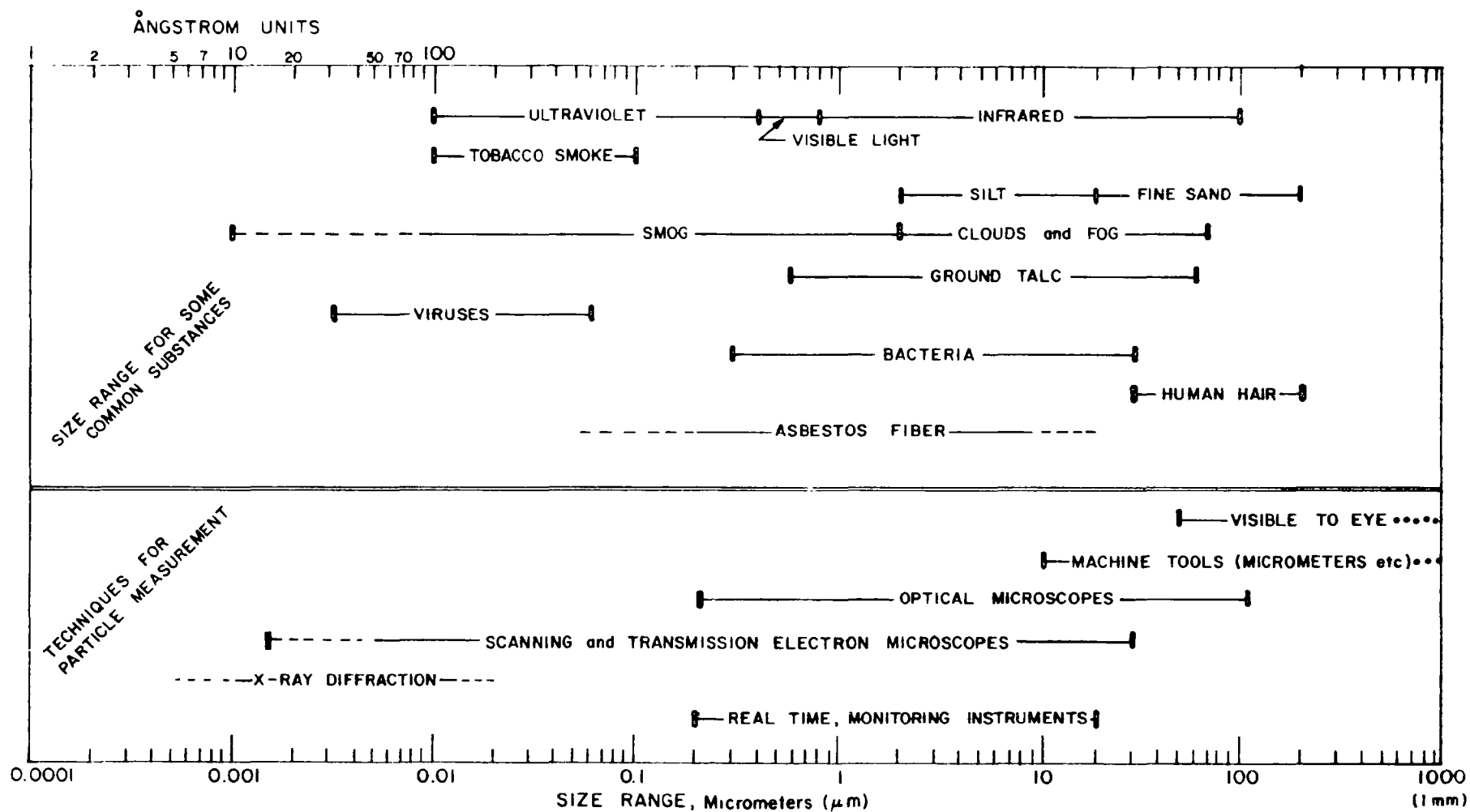
Figure I-2-1. Asbestos size comparison with other particles and measurement techniques.
