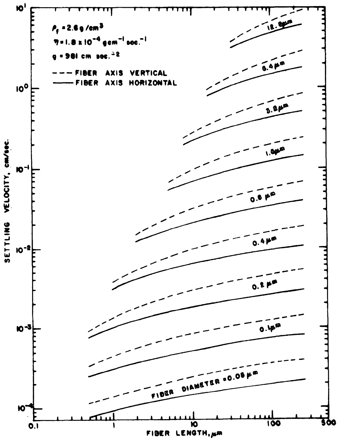
Figure I-2-2. Theoretical settling velocities of fibers.
