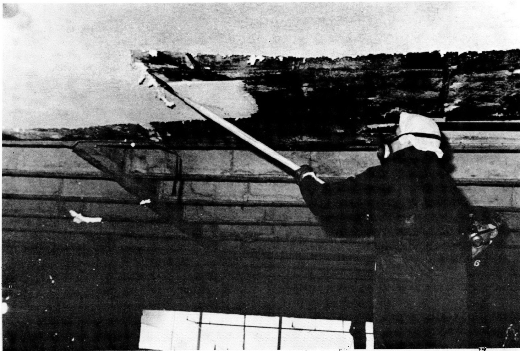
Figure E-1. Removal of asbestos-containing ceiling material. Note use of headgear, coveralls and respiratory protection.
