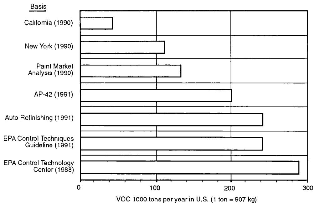
Figure 1. National VOC estimations by different methods.
