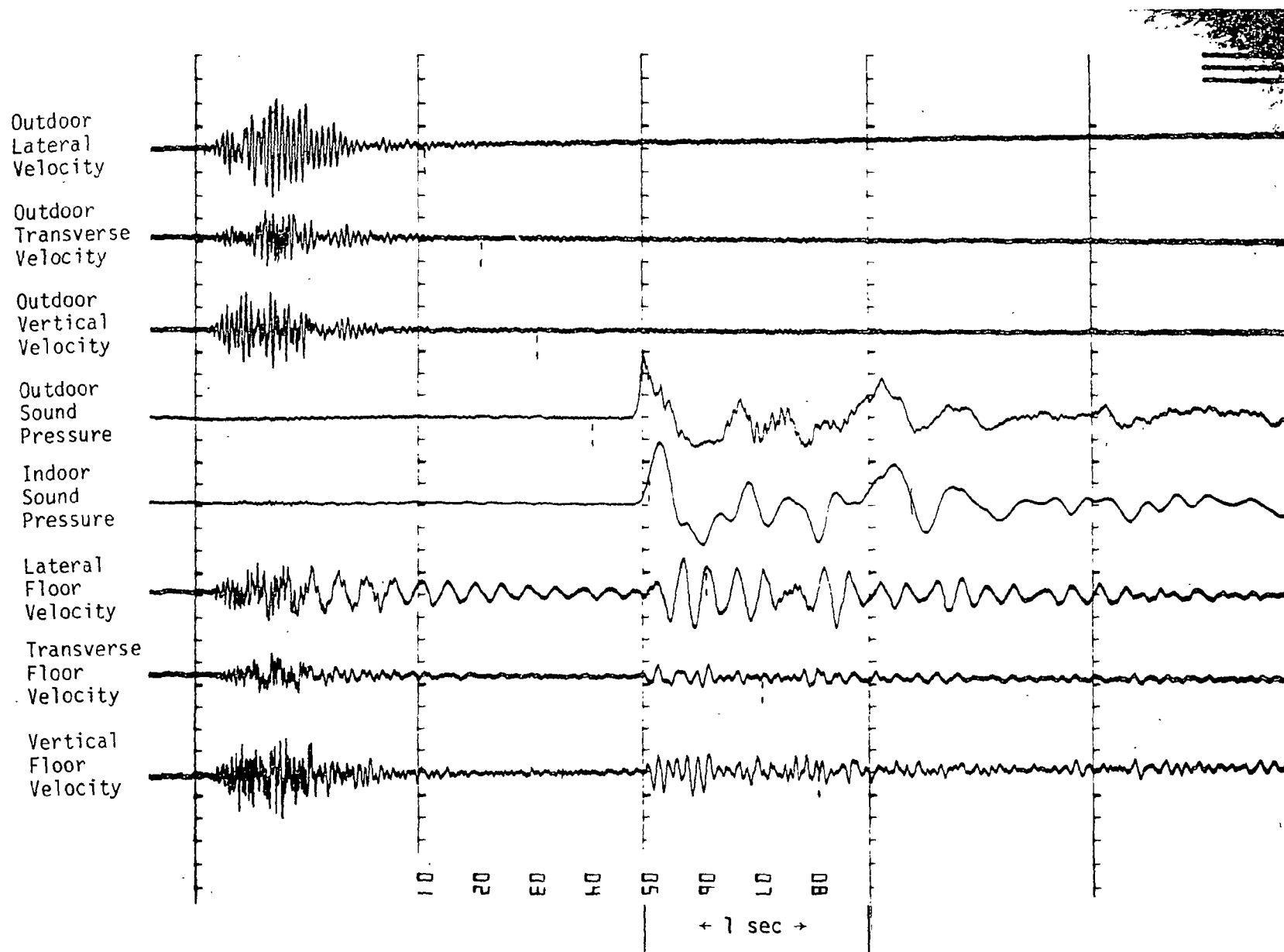
Fig. B-11. Oscillograph Record of Blast No. 11
