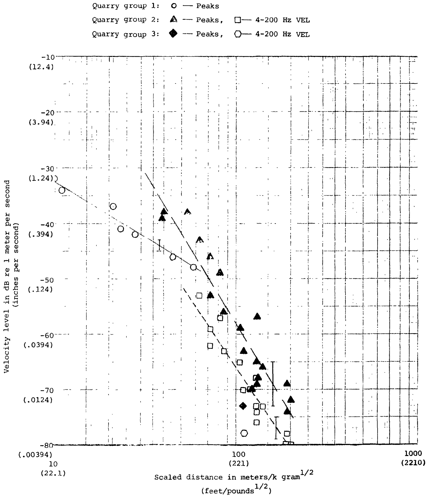
Fig. 3.7-1. Velocity Levels versus Scaled Distance
