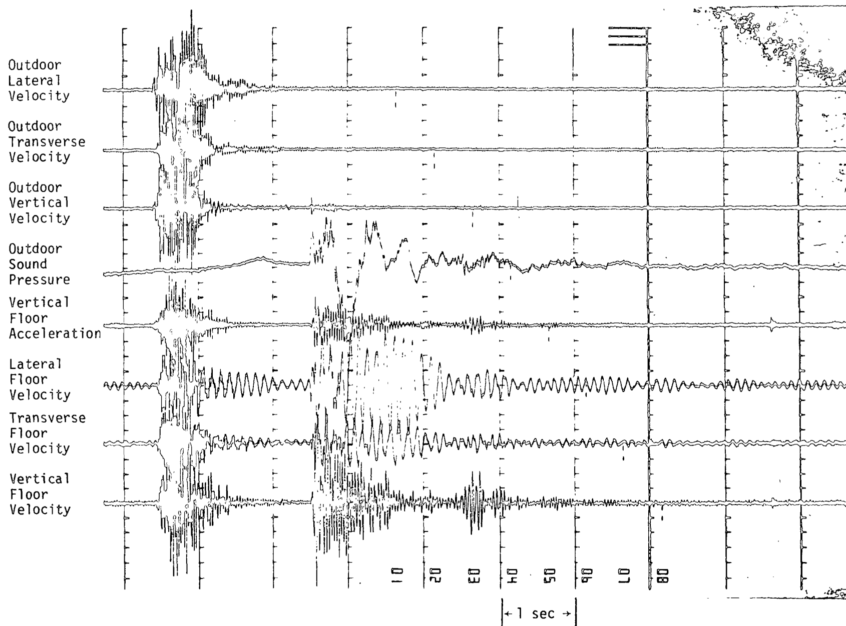
Fig. B-15. Oscillograph Record of Blast No. 15
