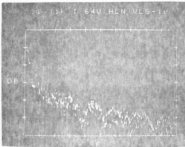
Fig. 4.2.2-4. Frequency spectrum of blast, including hole blowout. Full scale 120 dB, frequency range 0 to 1000 Hz.
