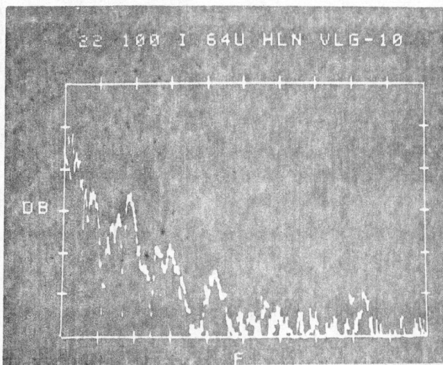
Fig. A.3.3-3 Air blast frequency spectrum with rectangular "window."
