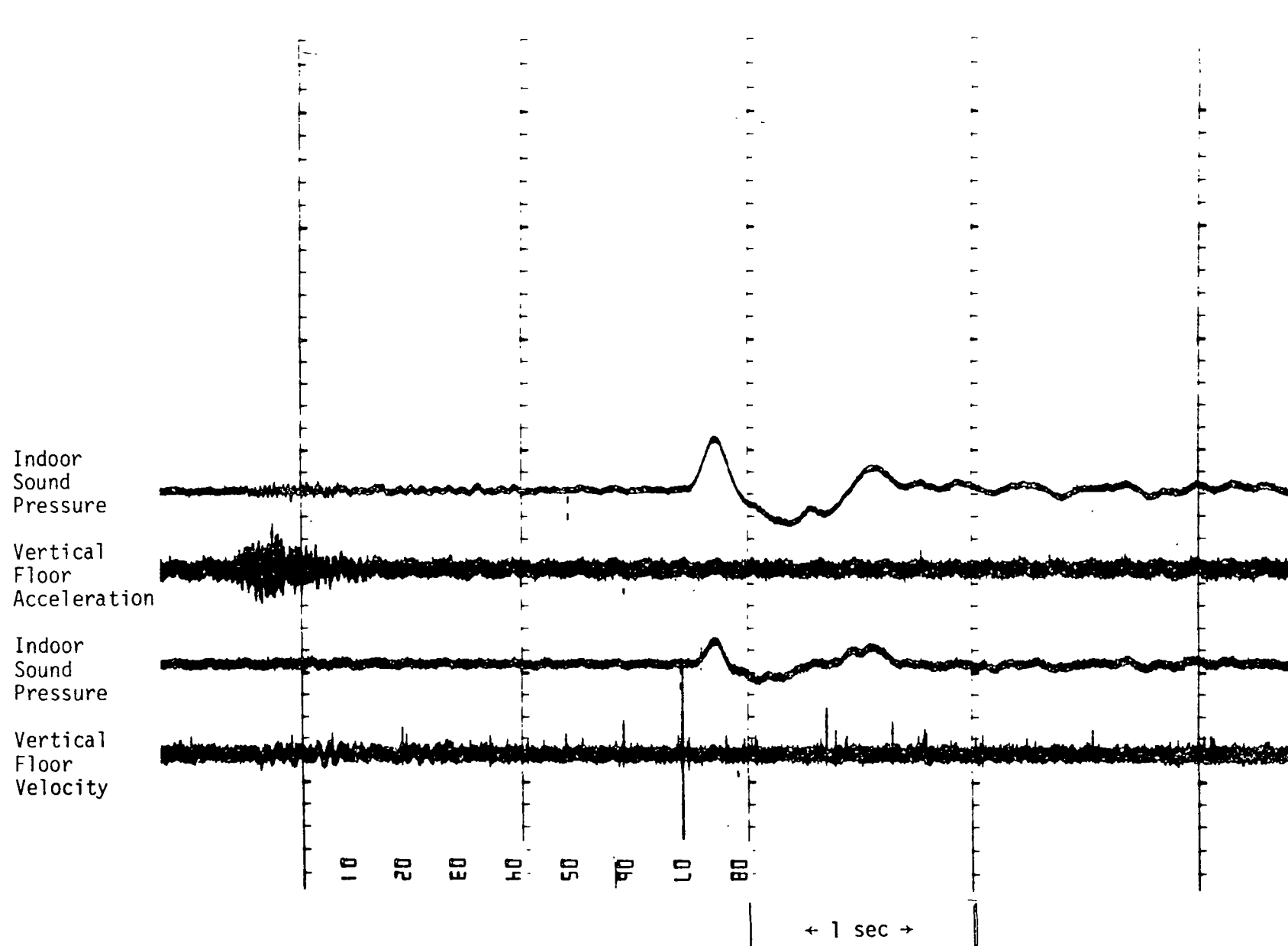
Fig. B-1. Oscillograph Record of Blast No. 1
