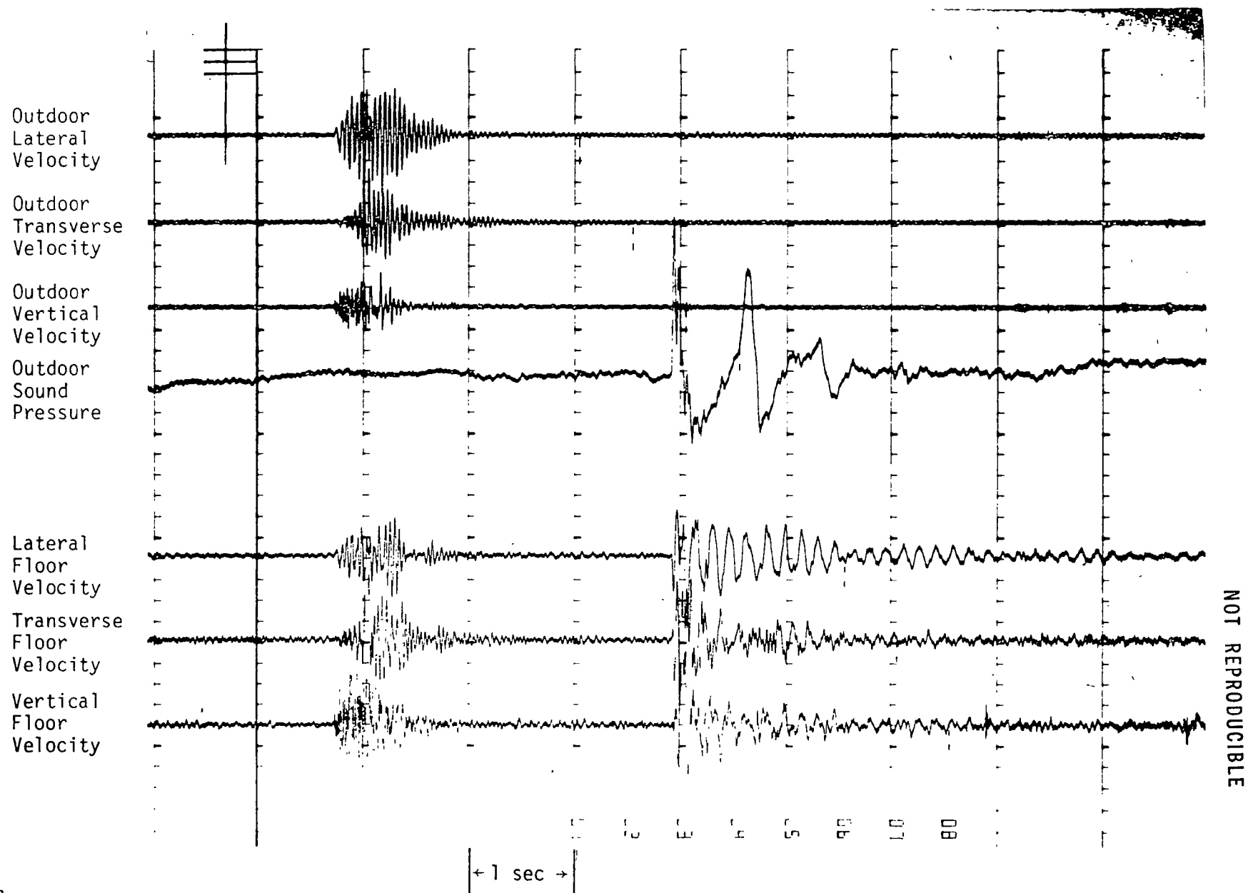
Fig. B-18. Oscillograph Record of Blast No. 18
