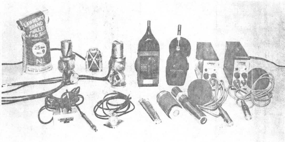
Fig. A.1.4-1 Blast noise and vibration-measurement transducers.
