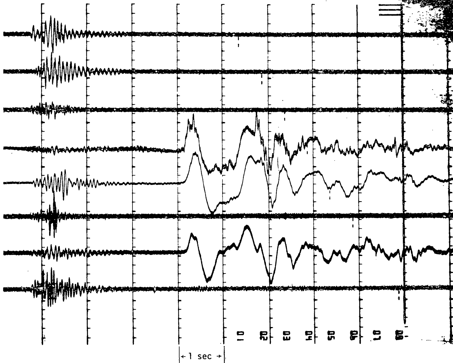
Fig. B-3. Oscillograph Record of Blast No. 3
