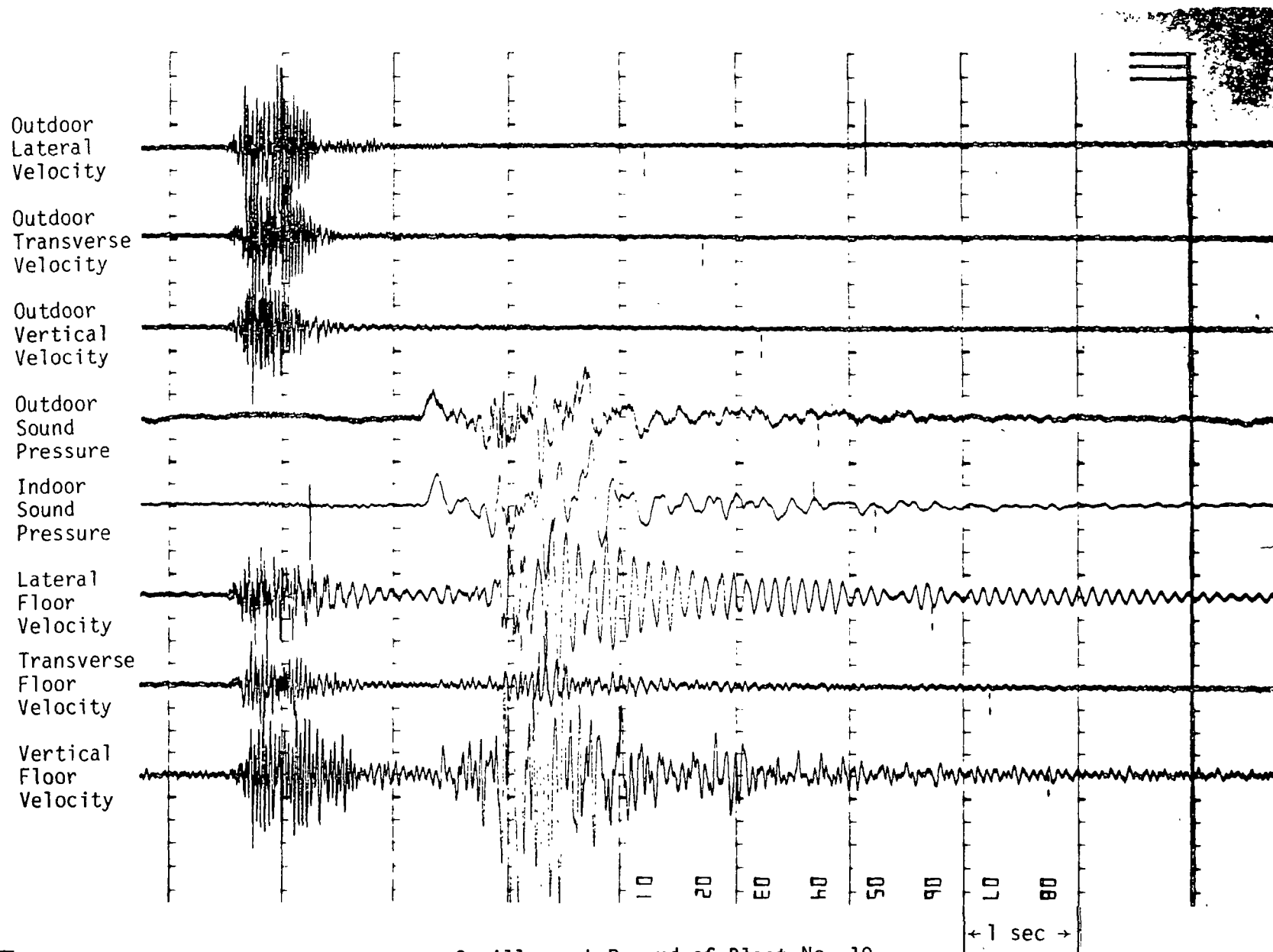
Fig. B-10. Oscillograph Record of Blast No. 10
