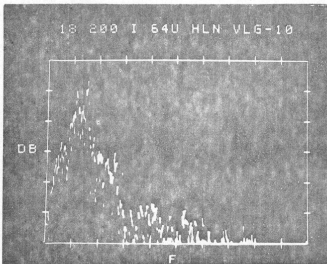
Fig. A.4.2-7 Indoor vertical floor velocity due to the air wave.
