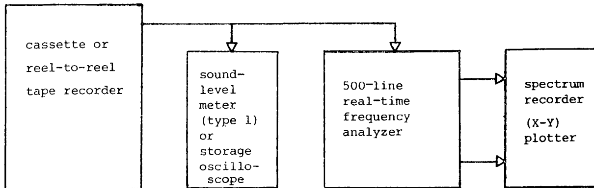
Laboratory Blast Noise Analysis System
