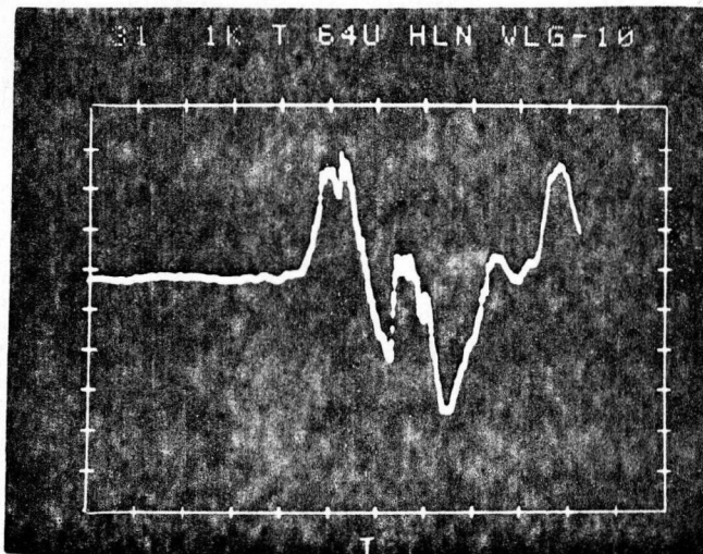
Fig. 4.2.2-1. Time history of blast prior to blowout (.2 sec time elapsed).
