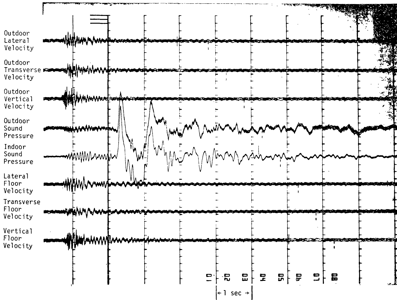
Fig. B-6. Oscillograph Record of Blast No. 6
