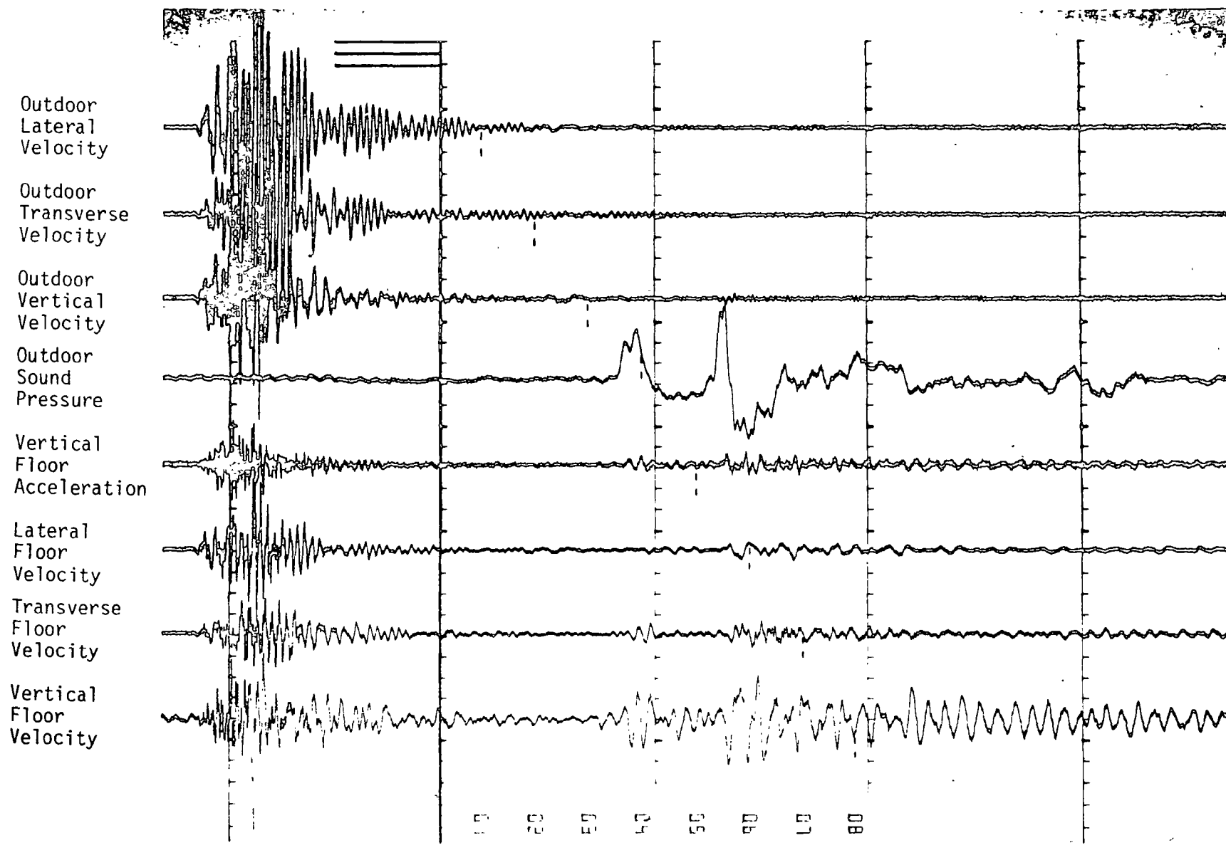
Fig. B-16. Oscillograph Record of Blast No. 16
