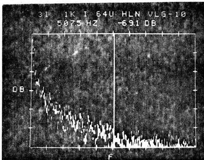
Fig. 4.2.2-2. Frequency spectrum of blast prior to hole blowout. Full scale 120 dB, frequency range 0 to 1000 Hz.
