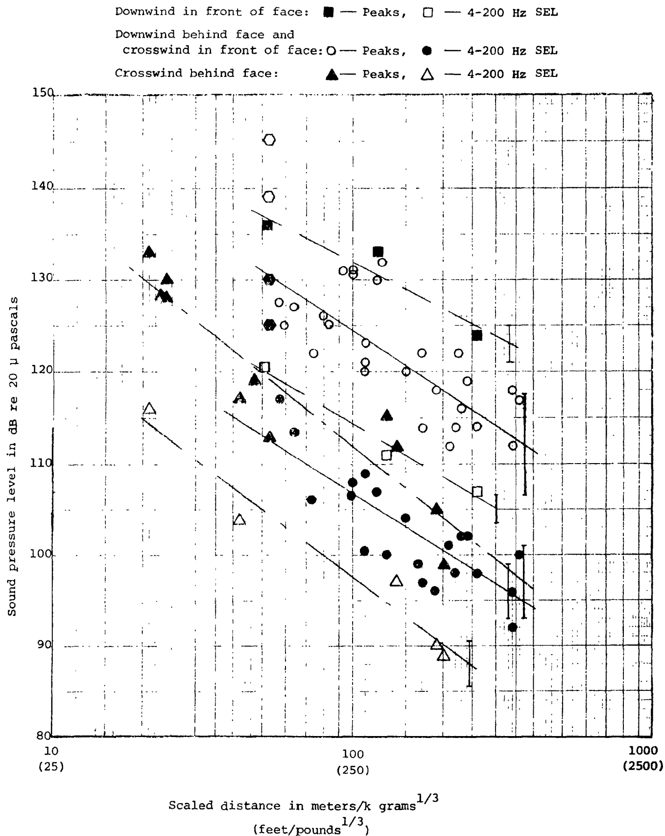
Fig. 3.7-2. Sound Levels versus Scaled Distance
