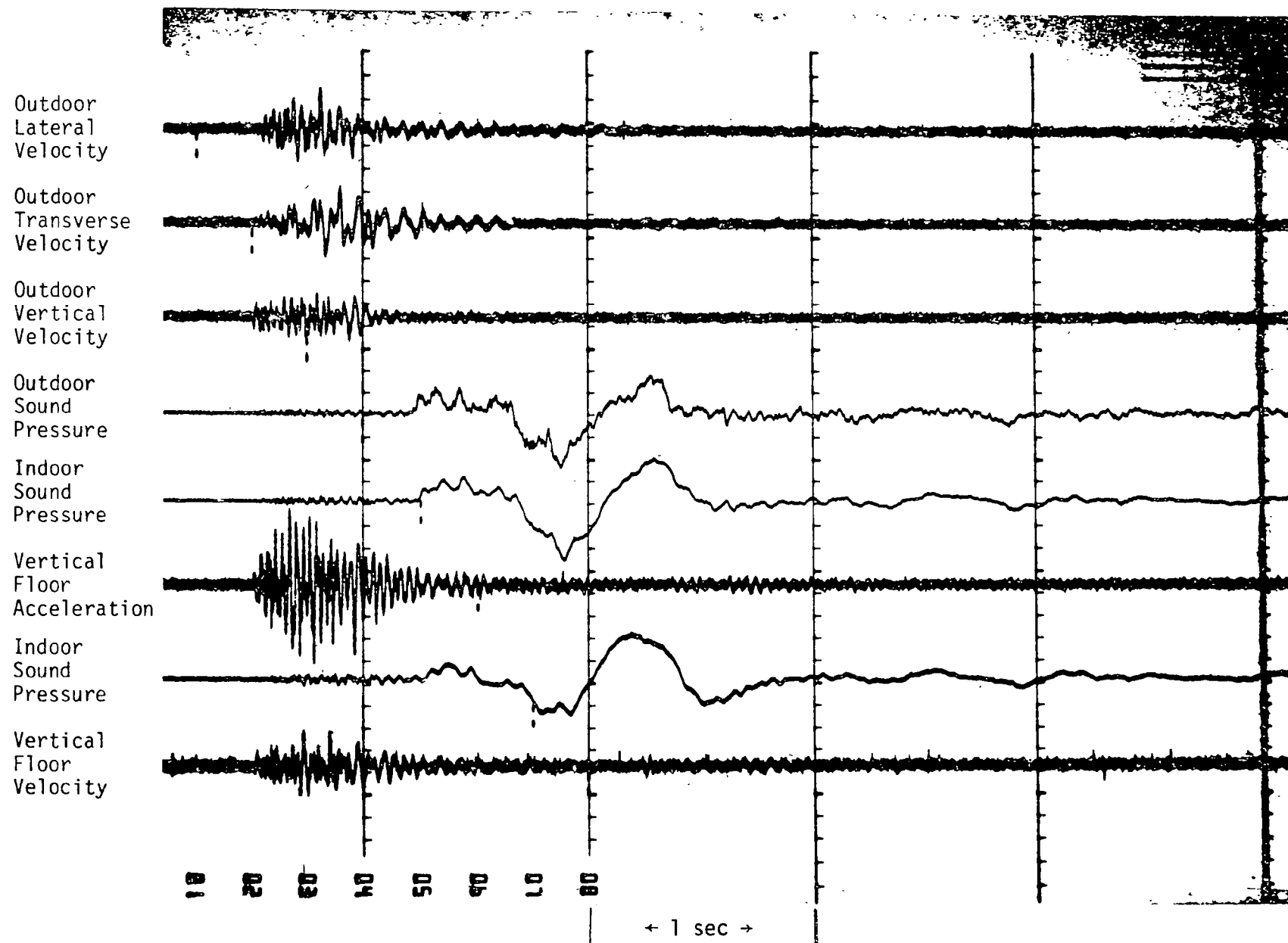
Fig. B-2. Oscillograph Record of Blast No. 2
