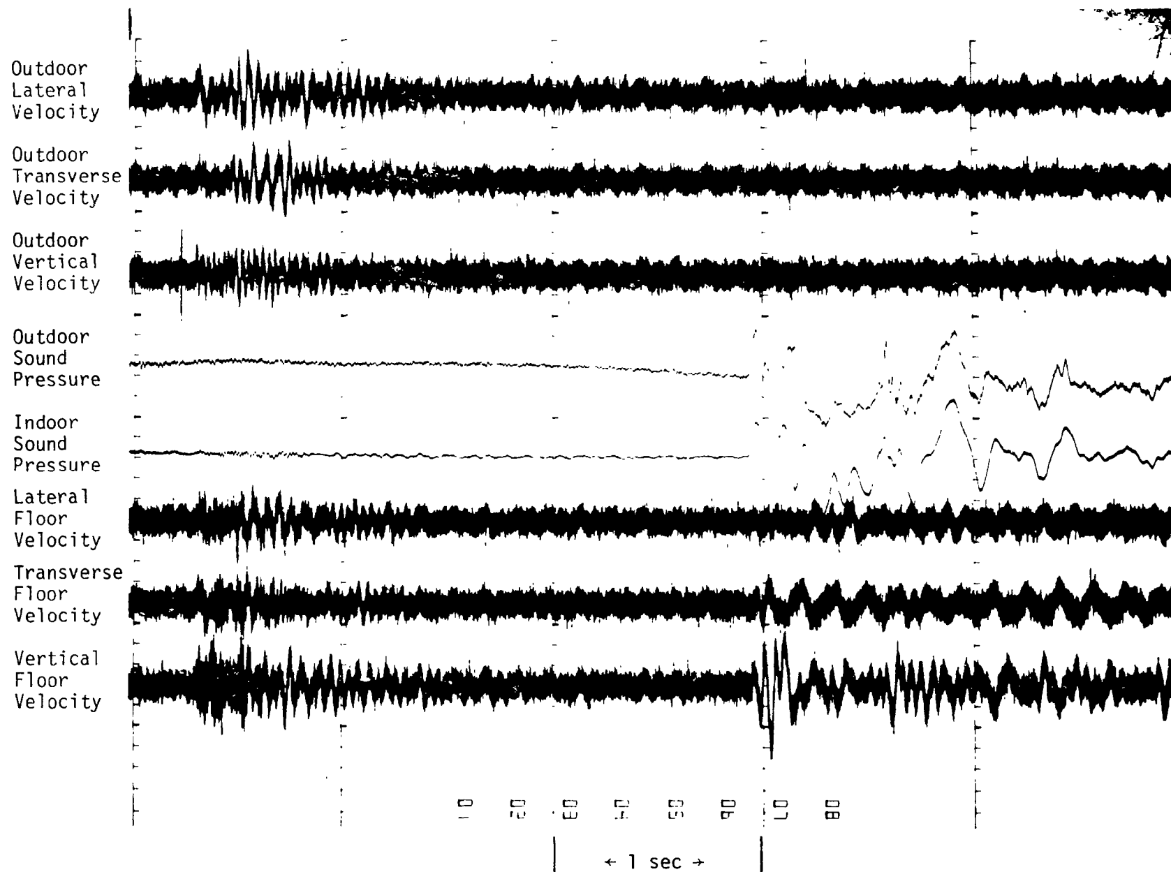
Fig. B-9. Oscillograph Record of Blast No. 9
