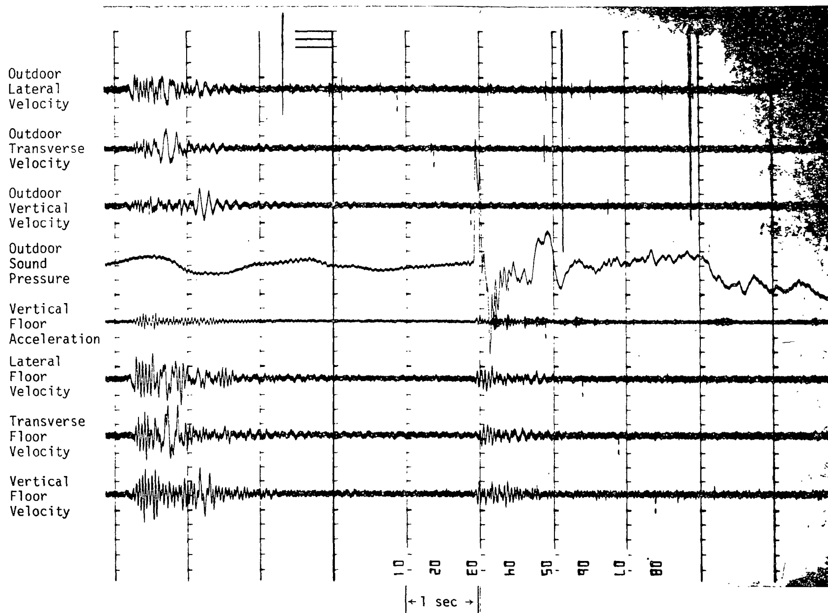
Fig. B-14. Oscillograph Record of Blast No. 14
