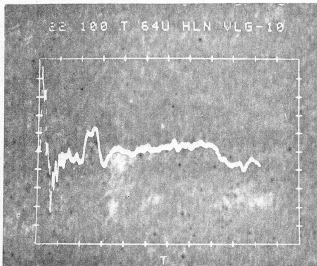
Fig. A.3.3-2 Amplitude-time history of an air blast.
