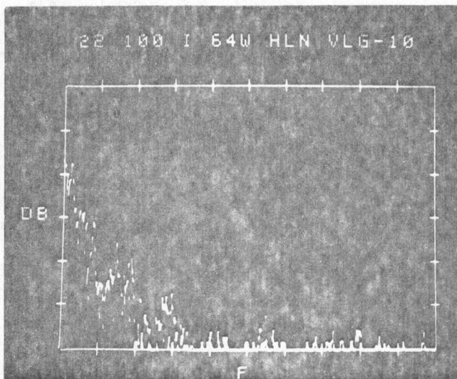
Fig. A.3.3-4 Air blast frequency spectrum with Hanning "window."
