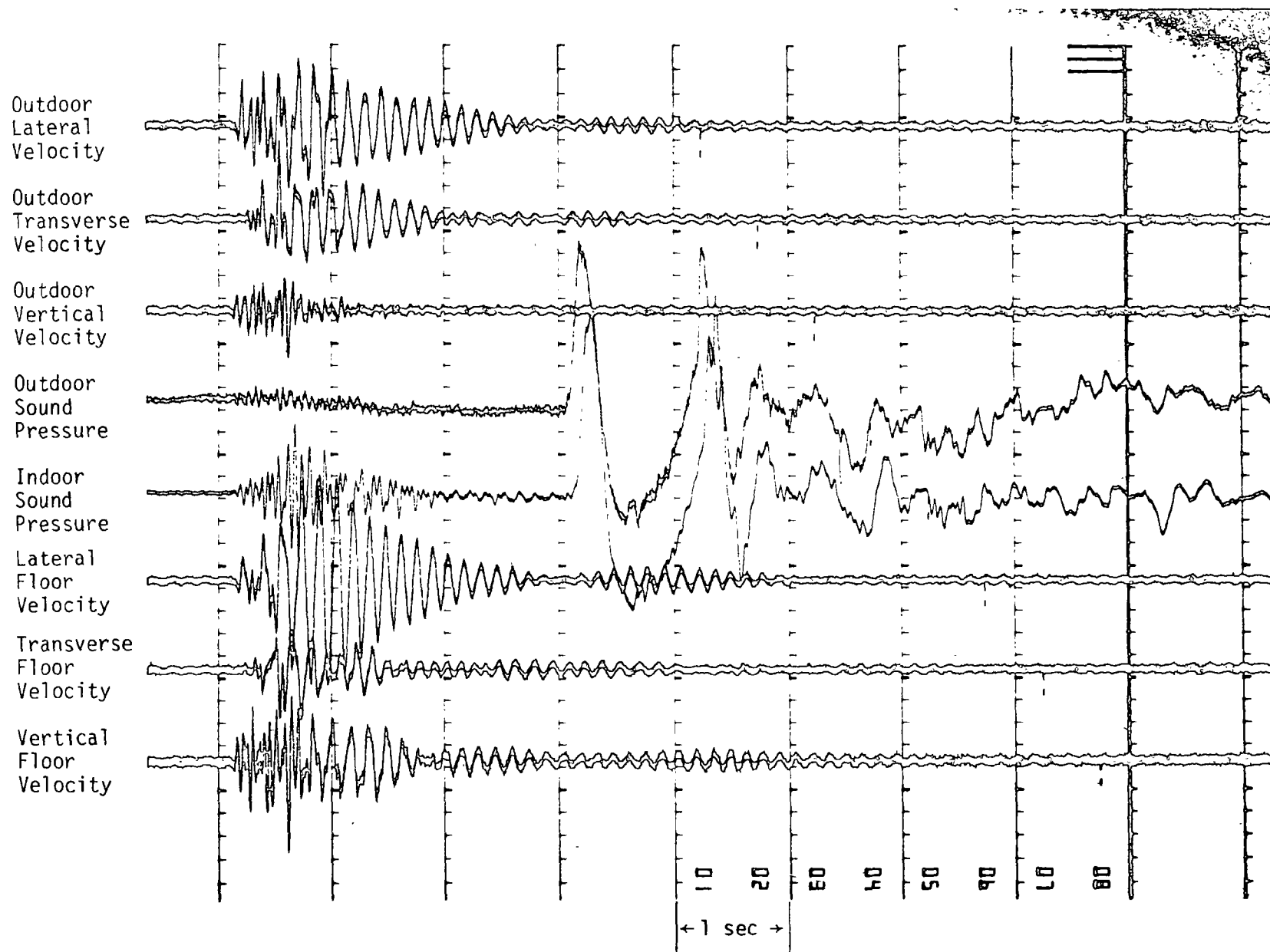
Fig. B-7. Oscillograph Record of Blast No. 7
