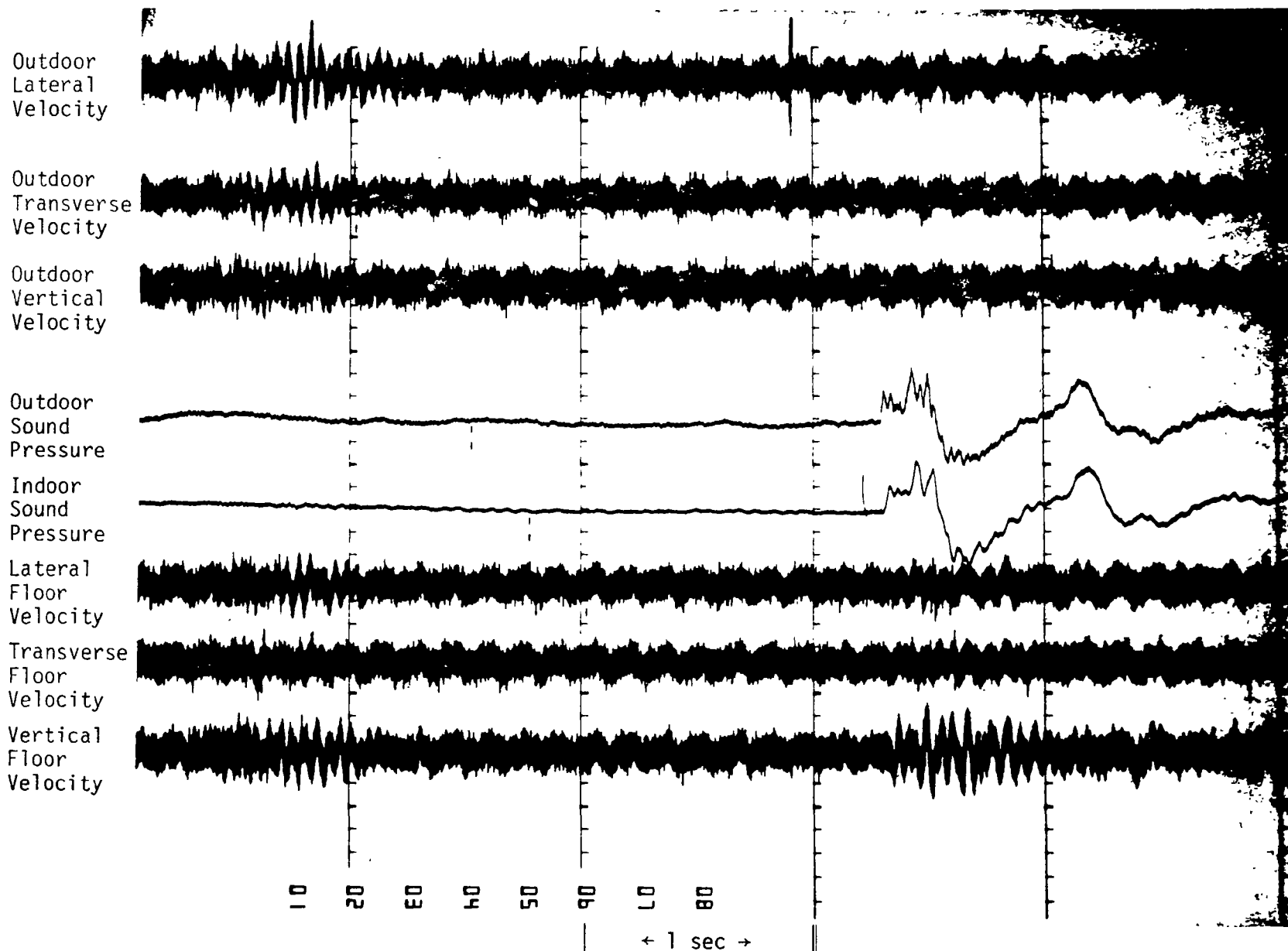
Fig. B-8. Oscillograph Record of Blast No. 8
