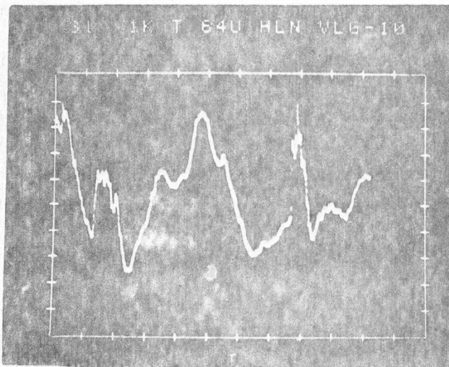
Fig. 4.2.2-3. Time history of blast, including hole blowout (0.2 seconds total time elapsed).
