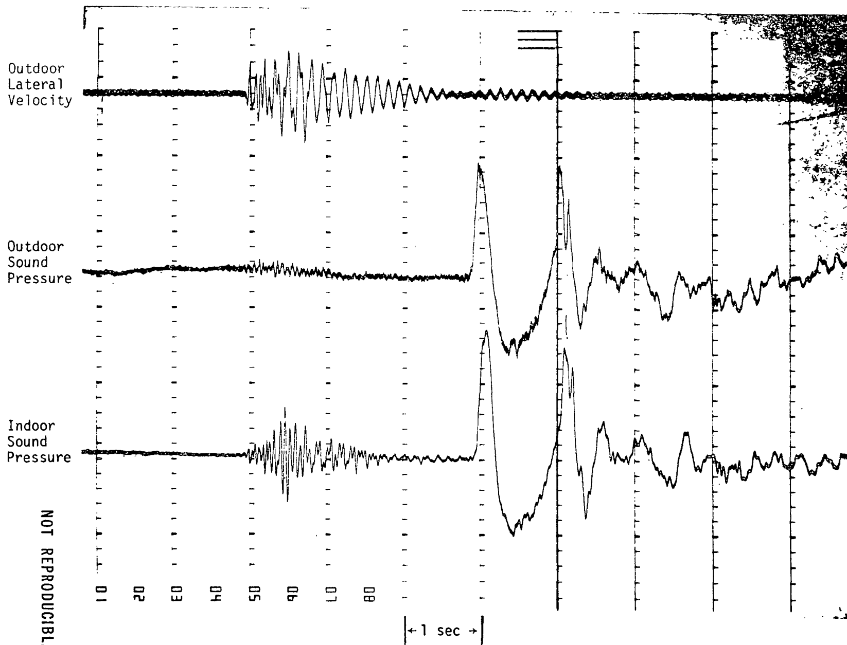
Fig. A.4.1-2. Oscillograph Record of Blast No. 7
