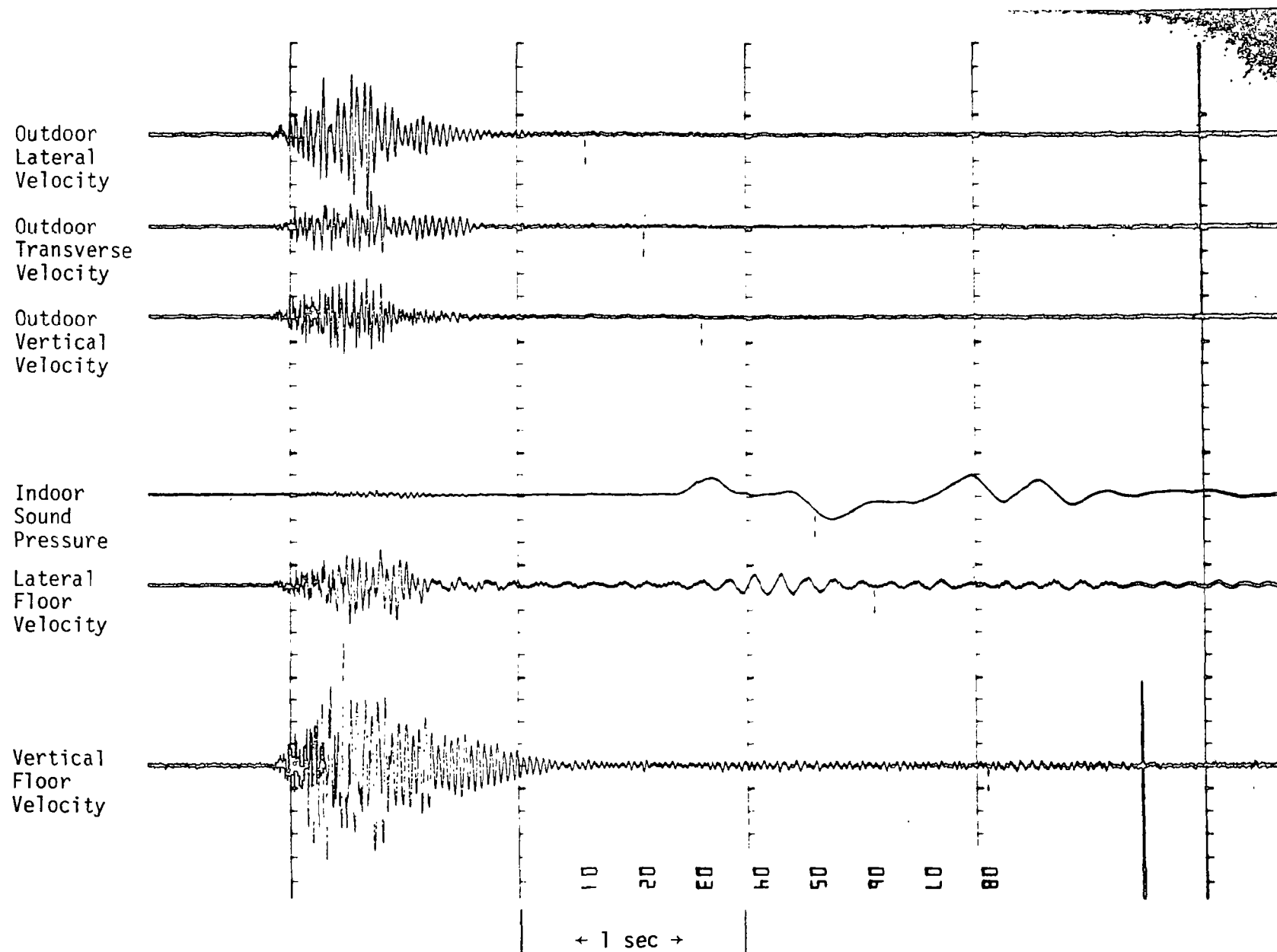
Fig. B-12. Oscillograph Record of Blast No. 12
