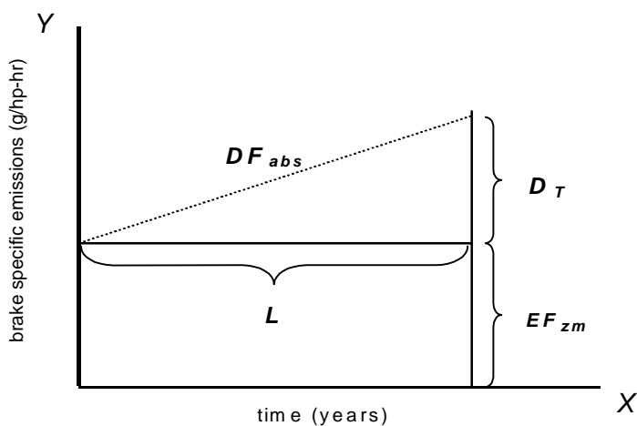
Figure 1. Conceptual representation of absolute linear emissions deterioration over the useful life of a diesel engine.
