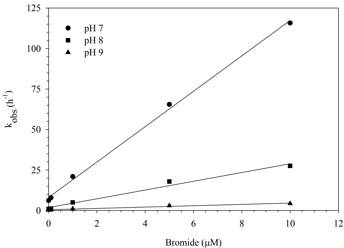
Figure 8 Observed first order rate coefficients for CP loss in the presence of increasing bromide concentrations at [\text{HOCl}]_{\text{T}} = 10 \mu\text{M} over the pH range of 7-9. [\text{CP}]_{\text{o}} = 0.5 \mu\text{M} , [\text{Buffer}]_{\text{T}} = 10 \text{mM} , and Temperature = 25 \text{ }^{\circ}\text{C} .
