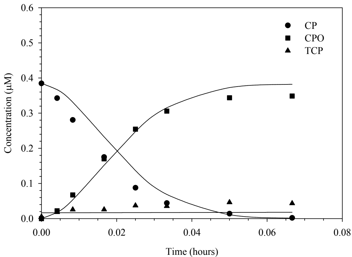
Figure 20 CP degradation in the presence of free chlorine and bromide at pH 8.0. [CP]_o = 0.39 \mu\text{M} , [\text{HOCl}]_T = 50 \mu\text{M} , [\text{Br}^-] = 10 \mu\text{M} , [\text{PO}_4]_T = 10 \text{mM} , and Temperature = 25^\circ\text{C} . Lines represent model results.
