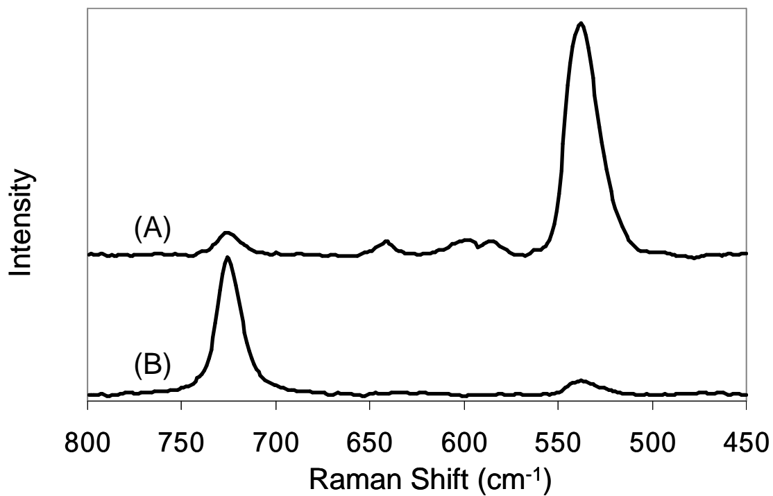
Figure 5 Raman spectra comparing 13.1 mM free chlorine solutions with (A) equimolar chloride ion at pH 0.75 (ECS) and (B) free chlorine solution with reduced chloride ion at pH 0.80 (LCS). The spectrum of the solution containing equimolar chloride ion has a much larger band at 538 cm -1 (due to aqueous Cl 2 ) than the solution with greatly reduced chloride concentration.
