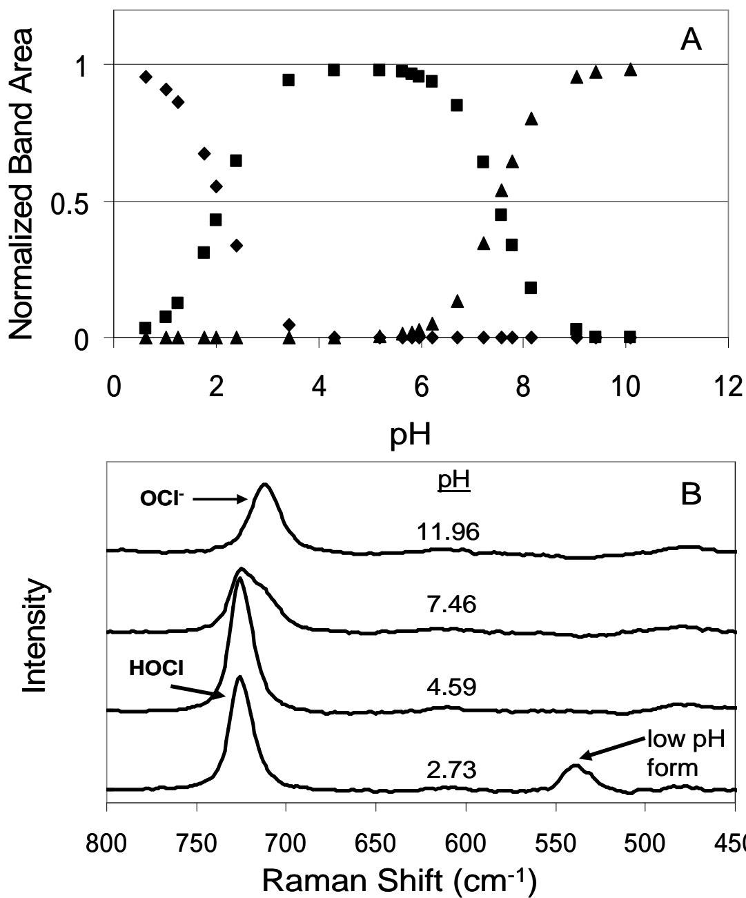
Figure 2 (A.) Speciation plot of the 26.2 mM commercial free chlorine solution (the ECS solution) generated by monitoring the normalized areas of the Raman bands from OCl - at 711 cm -1 (▲), HOCl at 725 cm -1 (■) and the low pH species at 538 cm -1 (◆). (B.) Background-subtracted Raman spectra of ECS solutions. The OCl - band is observed in the top two spectra and the HOCl band is observed in the bottom three spectra. An additional band for the low pH form appears as the pH is lowered below 5.
