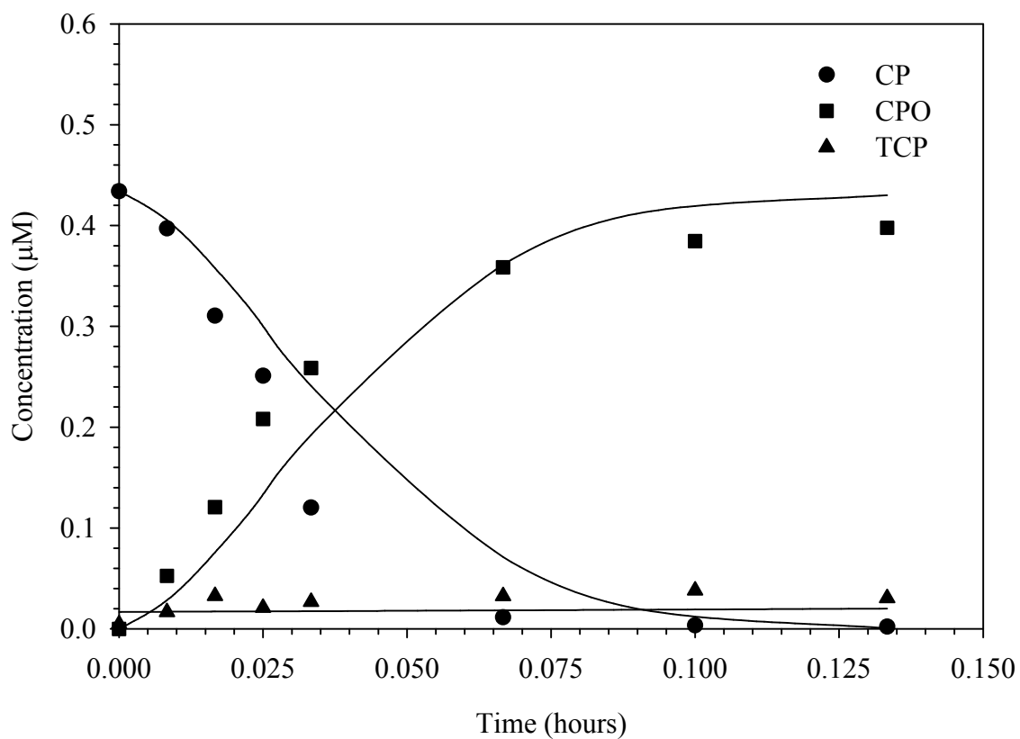
Figure 19 CP degradation in the presence of free chlorine and bromide at pH 8.0. [CP]_o = 0.43 \mu\text{M} , [\text{HOCl}]_T = 50 \mu\text{M} , [\text{Br}^-] = 5 \mu\text{M} , [\text{PO}_4]_T = 10 \text{mM} , and Temperature = 25 °C. Lines represent model results.
