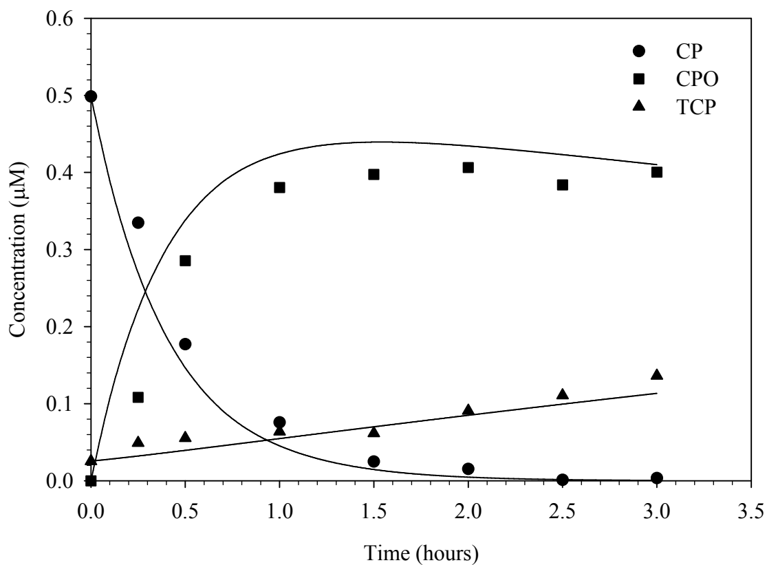
Figure 27 CP degradation in the presence of free chlorine and ACC water at pH 9.0. [CP]_0 = 0.5 \mu\text{M} , [\text{HOCl}]_T = 50 \mu\text{M} , [\text{DOC}] = 1.1 \text{ mg-C/L} , [\text{Buffer}]_T = 10 \text{ mM} , and Temperature = 25 °C. Lines represent model results.
