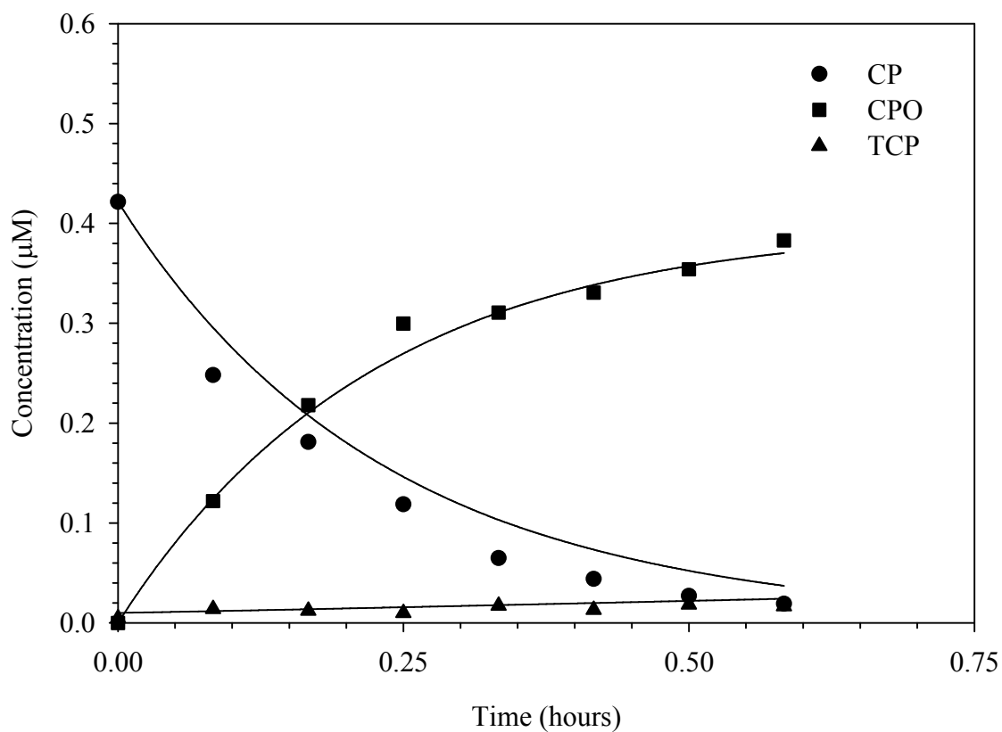
Figure 14 CP degradation in the presence of free chlorine at pH 8.0 in the absence of bromide. [CP]_o = 0.42 \mu\text{M} , [\text{HOCl}]_T = 50 \mu\text{M} , [\text{PO}_4]_T = 10 \text{ mM} , and Temperature = 25 °C. Lines represent model results.
