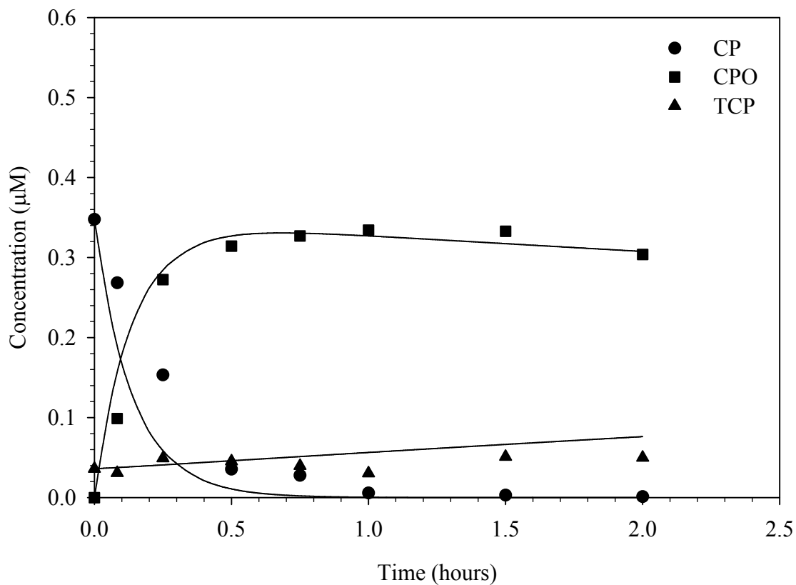
Figure 26 CP degradation in the presence of free chlorine and ACC water at pH 8.5. [CP]_0 = 0.35 \mu\text{M} , [\text{HOCl}]_T = 50 \mu\text{M} , [\text{DOC}] = 1.1 \text{ mg-C/L} , [\text{Buffer}]_T = 10 \text{ mM} , and Temperature = 25 °C. Lines represent model results.
