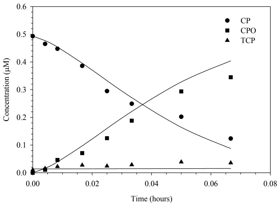
Figure 17 CP degradation in the presence of free chlorine and bromide at pH 8.0. [CP]_o = 0.49 \mu\text{M} , [\text{HOCl}]_T = 50 \mu\text{M} , [\text{Br}^-] = 1 \mu\text{M} , [\text{PO}_4]_T = 10 \text{mM} , and Temperature = 25 °C. Lines represent model results.
