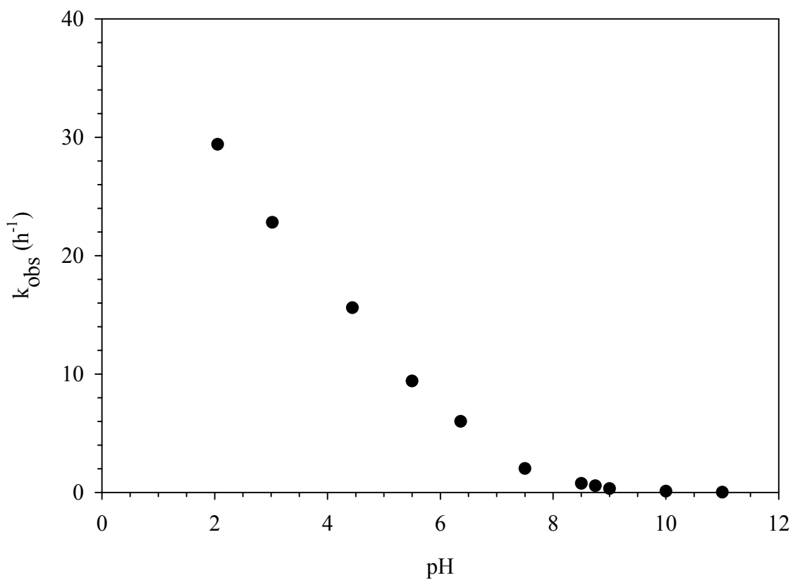
Figure 7 Observed first order loss rate coefficients for chlorpyrifos over the pH range of 2-11 in the presence of LCS. [CP]_o = 0.5 \mu\text{M} , [\text{Buffer}]_T = 10 \text{ mM} , Temperature = 25 \pm 1^\circ\text{C} , and [\text{HOCl}]_T = 10 \mu\text{M} .
