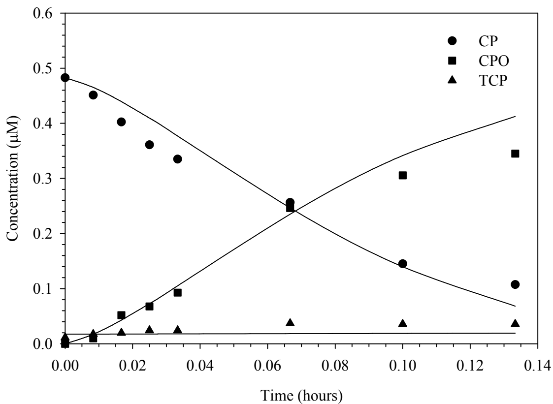
Figure 16 CP degradation in the presence of free chlorine and bromide at pH 8.0. [CP]_o = 0.48 \mu\text{M} , [\text{HOCl}]_T = 25 \mu\text{M} , [\text{Br}^-] = 1 \mu\text{M} , [\text{PO}_4]_T = 10 \text{mM} , and Temperature = 25 °C. Lines represent model results.
