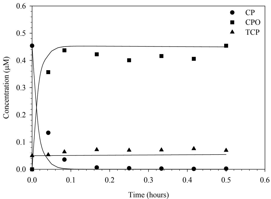
Figure 23 CP degradation in the presence of free chlorine and ACC water at pH 7. [CP]_o = 0.46 \mu\text{M} , [\text{HOCl}]_T = 50 \mu\text{M} , [\text{DOC}] = 1.1 \text{ mg-C/L} , [\text{Buffer}]_T = 10 \text{ mM} , and Temperature = 25 °C. Lines represent model results.
