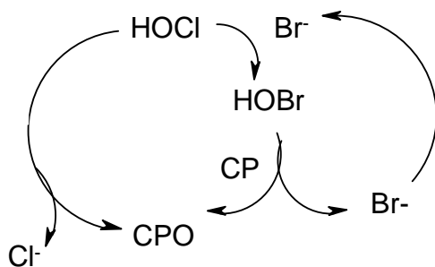
Figure 10 Two possible oxidation pathways for CP at high and low [\text{HOCl}]:[\text{Br}^-] ratios. The pathway on the left shows the predominant pathway when [\text{HOCl}] \gg [\text{Br}^-] and the pathway on the right shows the predominant pathway when [\text{HOCl}]:[\text{Br}^-] approaches 1.
