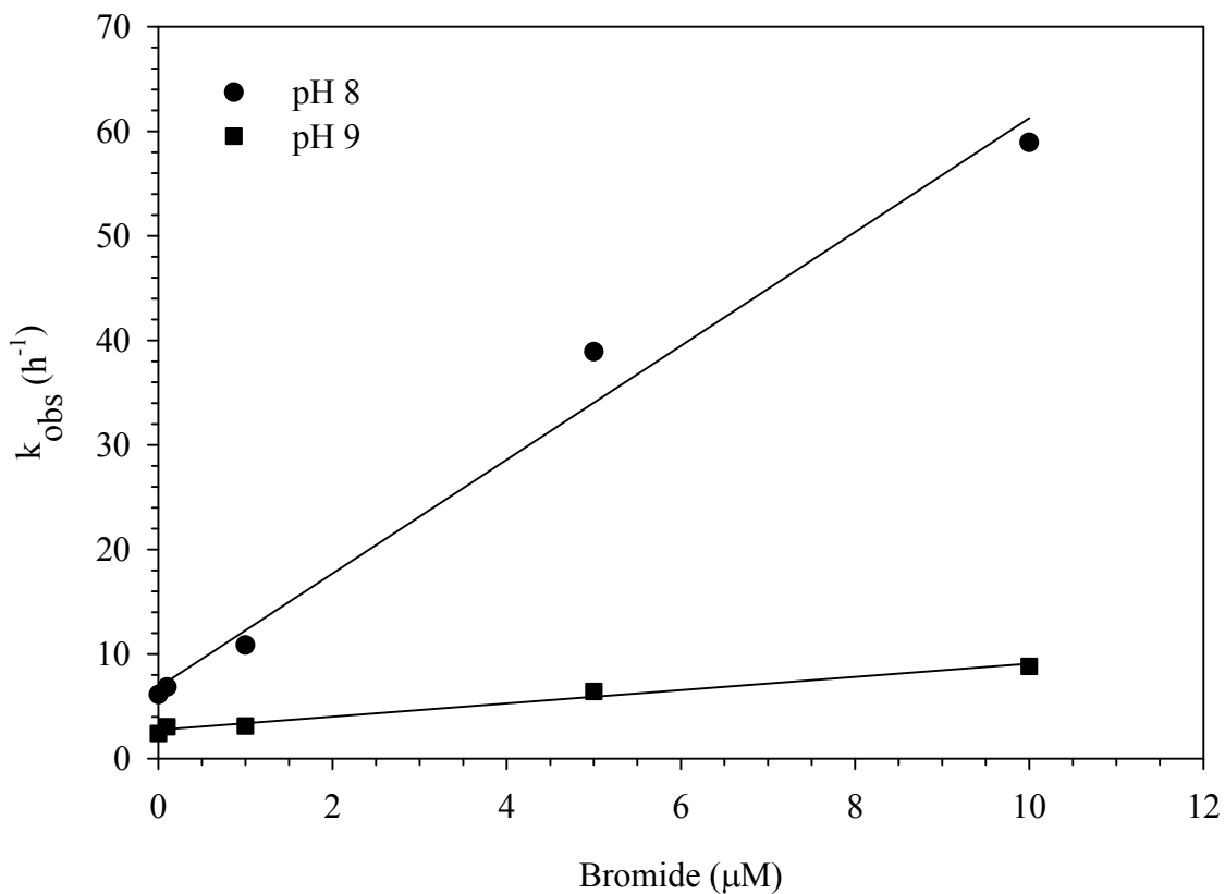
Figure 9 Observed first order rate coefficients for CP loss in the presence of increasing bromide concentrations at [\text{HOCl}]_{\text{T}} = 50 \mu\text{M} at pH 8 and 9. [\text{CP}]_{\text{o}} = 0.5 \mu\text{M} , [\text{Buffer}]_{\text{T}} = 10 \text{ mM} , and Temperature = 25 \text{ }^{\circ}\text{C} .
