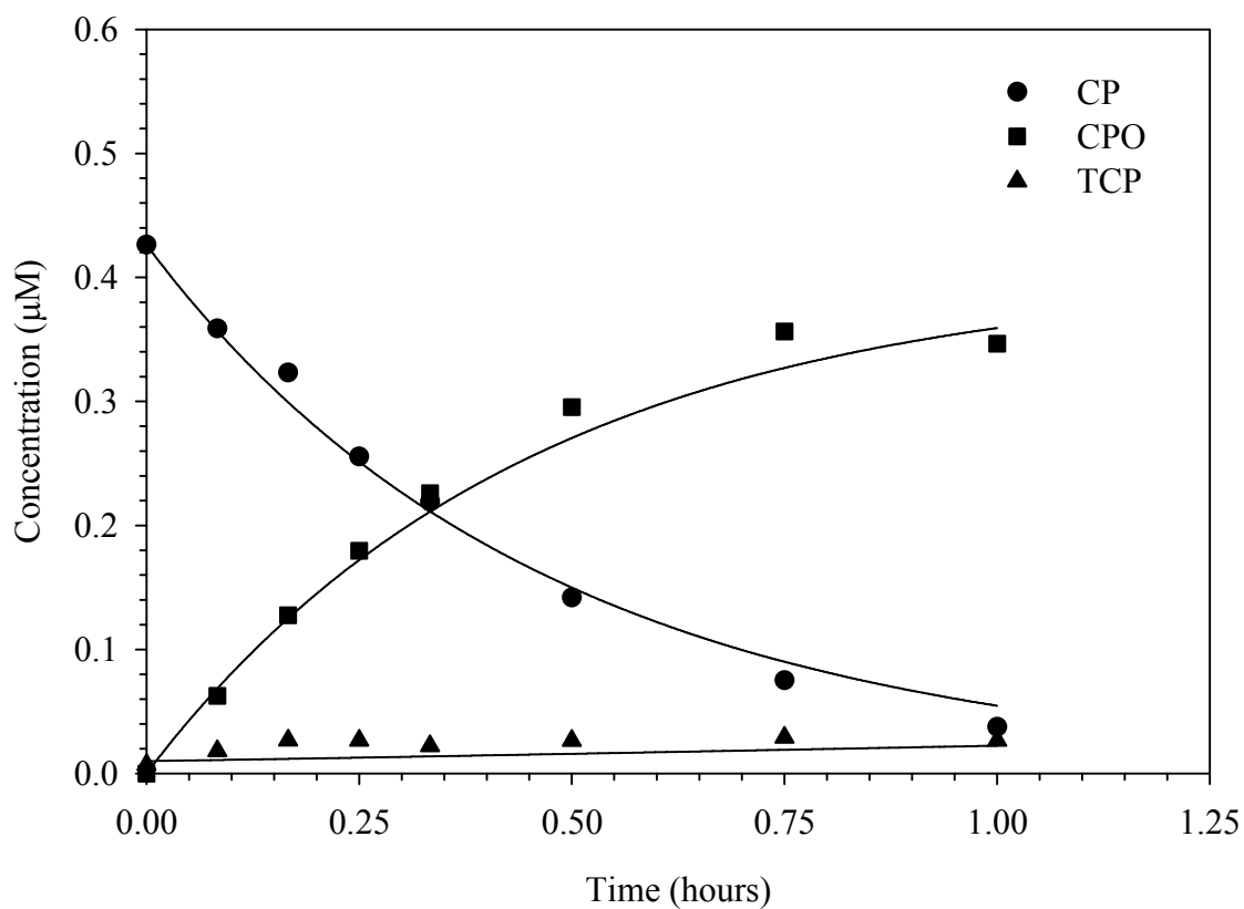
Figure 13 CP degradation in the presence of free chlorine at pH 8.0 in the absence of bromide. [CP]_0 = 0.42 \mu\text{M} , [\text{HOCl}]_T = 25 \mu\text{M} , [\text{PO}_4]_T = 10 \text{ mM} , and Temperature = 25 °C. Lines represent model results.
