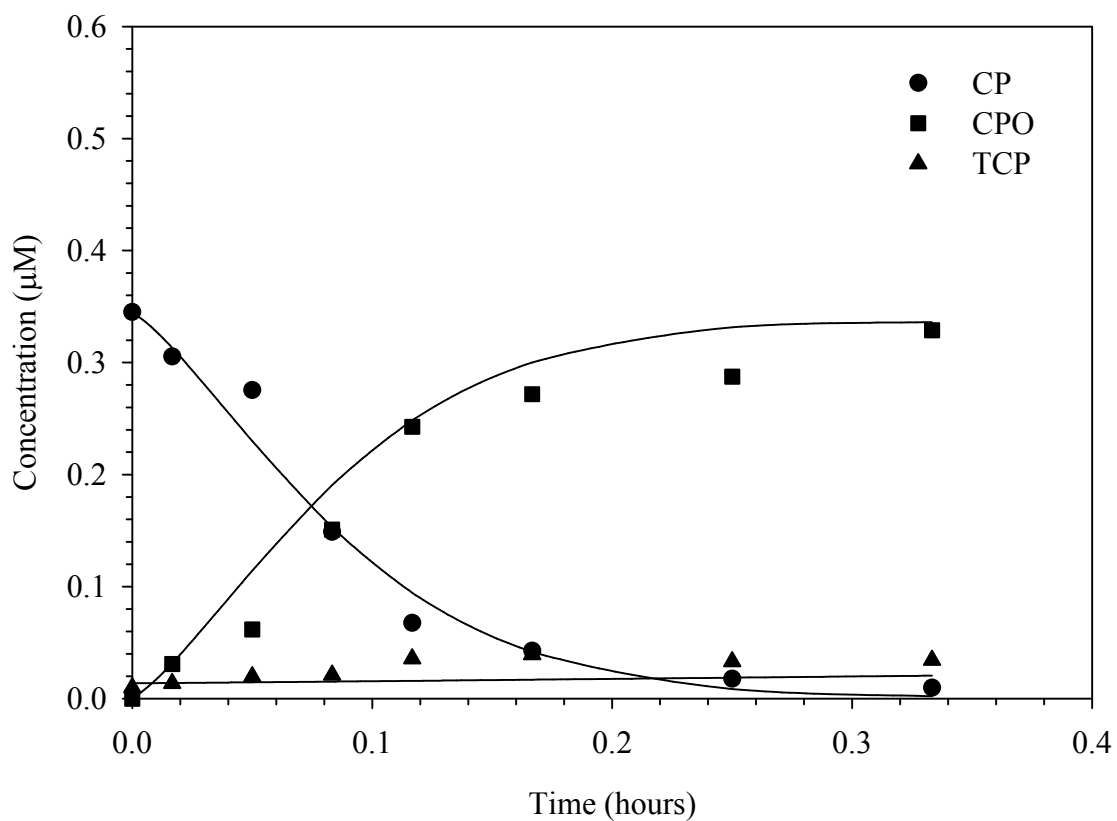
Figure 18 CP degradation in the presence of free chlorine and bromide at pH 8.0. [CP]_o = 0.35 \mu\text{M} , [\text{HOCl}]_T = 50 \mu\text{M} , [\text{Br}^-] = 1 \mu\text{M} , [\text{PO}_4]_T = 10 \text{mM} , and Temperature = 25 °C. Lines represent model results.
