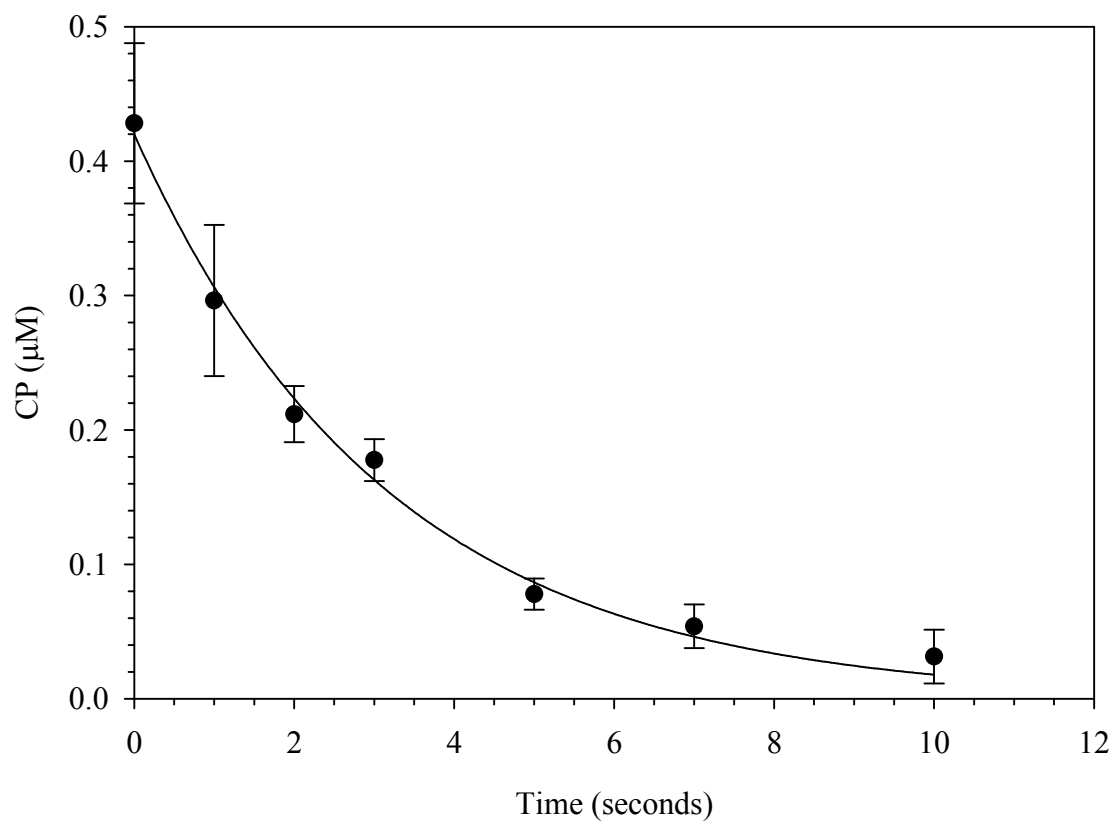
Figure 11 Loss of CP in the presence of hypobromous acid at pH 6.5. [\text{CP}]_0 = 0.42 \mu\text{M} , [\text{HOBr}]_T = 10 \mu\text{M} , [\text{Buffer}]_T = 10 \text{mM} , and Temperature = 25 \text{ }^\circ\text{C} .
