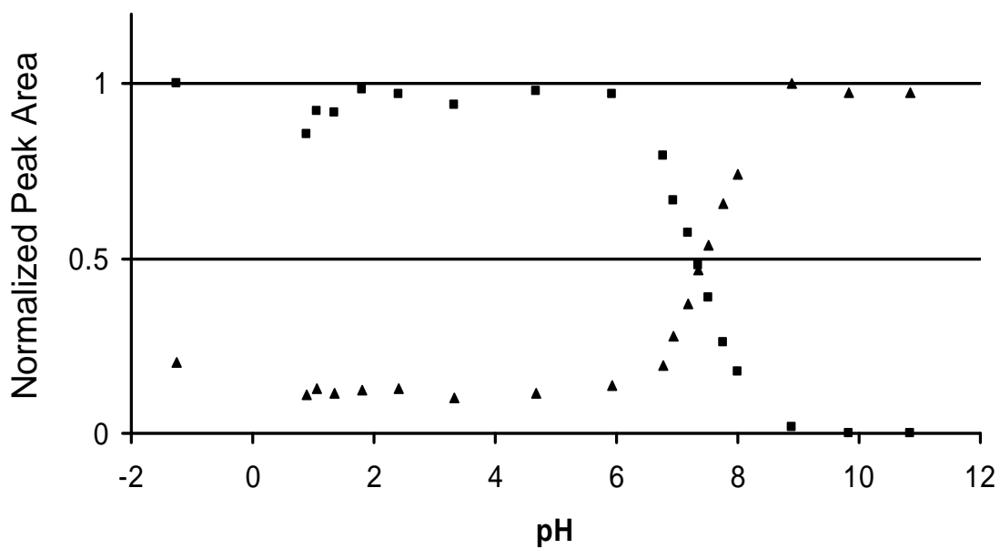
Figure 6 Speciation profile of the LCS free chlorine solution with reduced chloride ion concentration generated by monitoring the normalized areas of the Raman bands from HOCl at 725 cm -1 (■) and OCl - at 711 cm -1 (▲). The predominant species in solution at low pH remains HOCl throughout, and a significant drop in its total area is not observed as pH decreases.
