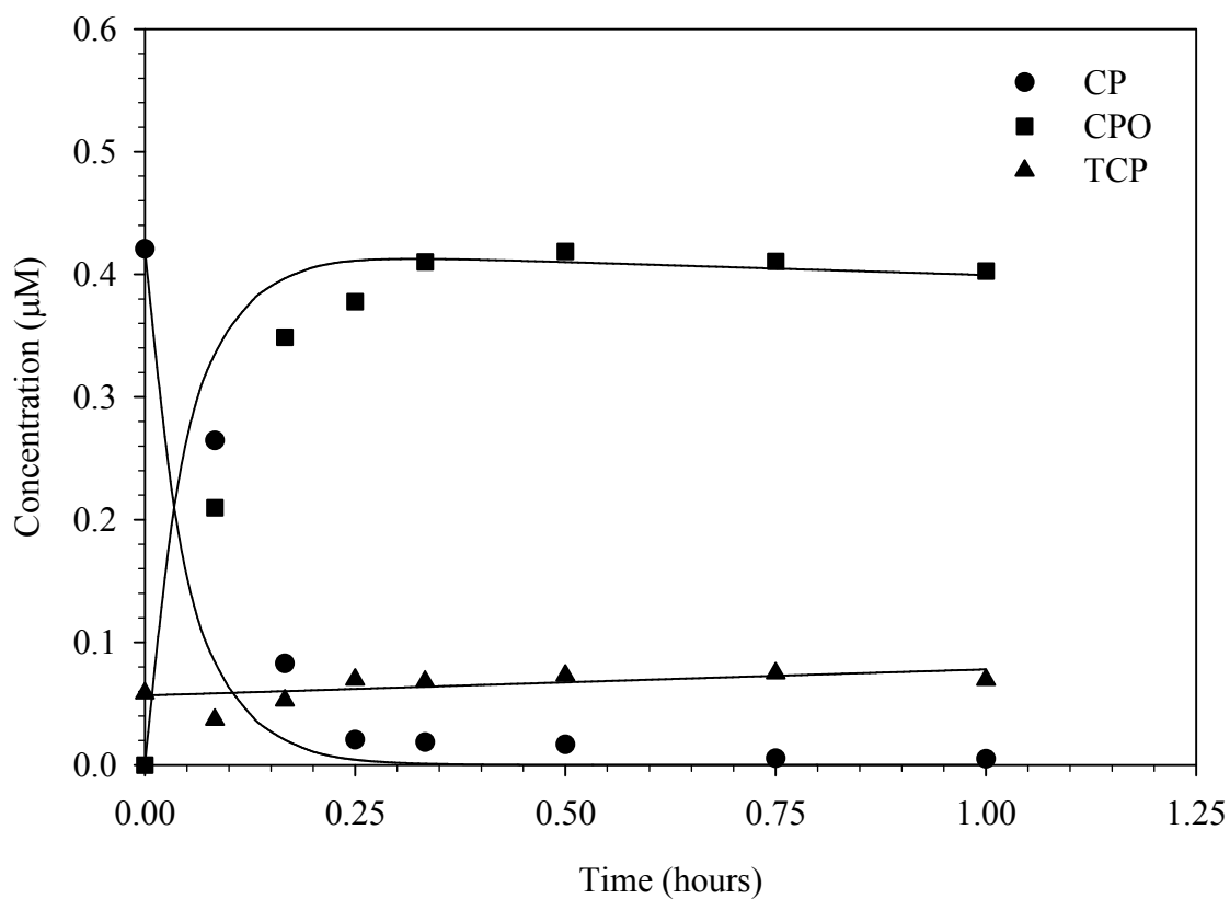
Figure 25 CP degradation in the presence of free chlorine and ACC water at pH 8.0. [CP]_0 = 0.42 \mu\text{M} , [\text{HOCl}]_T = 50 \mu\text{M} , [\text{DOC}] = 1.1 \text{ mg-C/L} , [\text{Buffer}]_T = 10 \text{ mM} , and Temperature = 25 °C. Lines represent model results.
