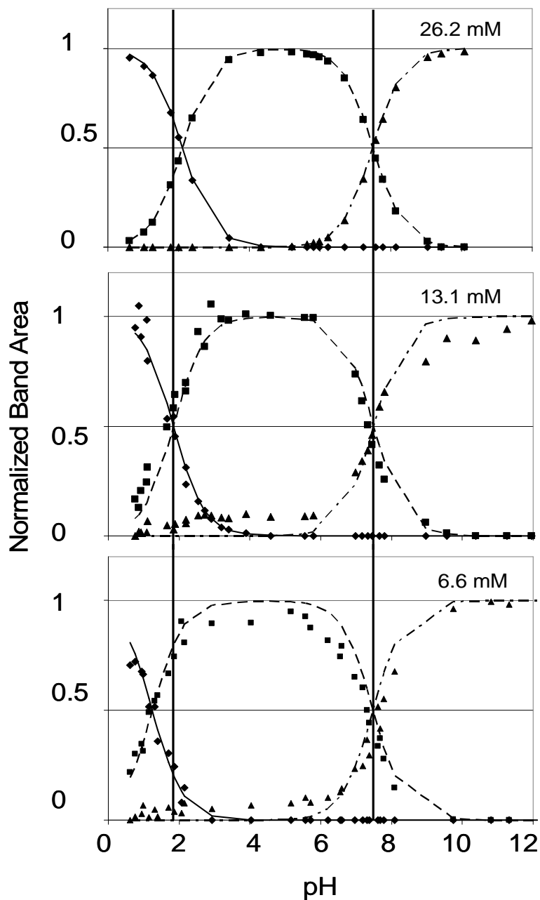
Figure 3 Speciation plots of commercial free chlorine solutions (ECS solutions) generated by monitoring the normalized areas of the Raman bands from OCl - at 711 cm -1 (▲, dash-dot model line), HOCl at 725 cm -1 (■, dashed model line) and the low pH species at 538 cm -1 (◆, solid model line). Vertical lines indicate the apparent pK a s at 13.1 mM. The pK a for the protonation of OCl - to HOCl occurs at 7.50 for all three concentrations. The apparent pK at lower pH varies from (from top to bottom): 2.11, 1.84, and 1.25.
