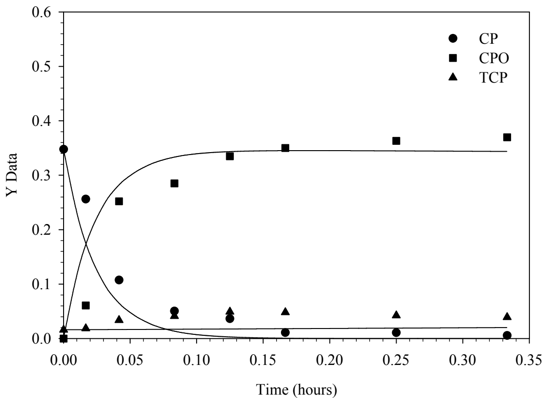
Figure 24 CP degradation in the presence of free chlorine and ACC water at pH 7.5. [CP]_0 = 0.35 \mu\text{M} , [\text{HOCl}]_T = 50 \mu\text{M} , [\text{DOC}] = 1.1 \text{ mg-C/L} , [\text{Buffer}]_T = 10 \text{ mM} , and Temperature = 25^\circ\text{C} . Lines represent model results.
