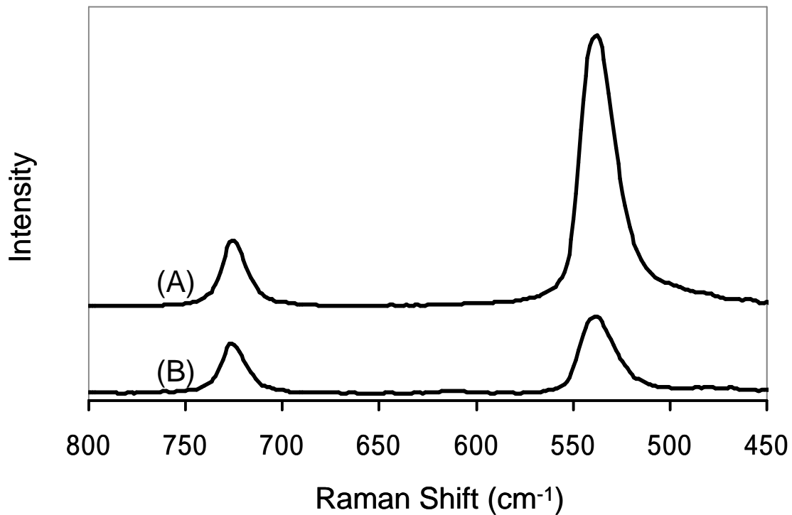
Figure 4 Raman spectrum acquired from (A) a buffered aqueous solution at pH 1.45 through which chlorine gas was bubbled (BCS) and (B) a pH 1.63 solution containing 13.1 mM commercial free chlorine (ECS). The band at 538 cm -1 is due to the presence of Cl 2 (aq) in each solution.
