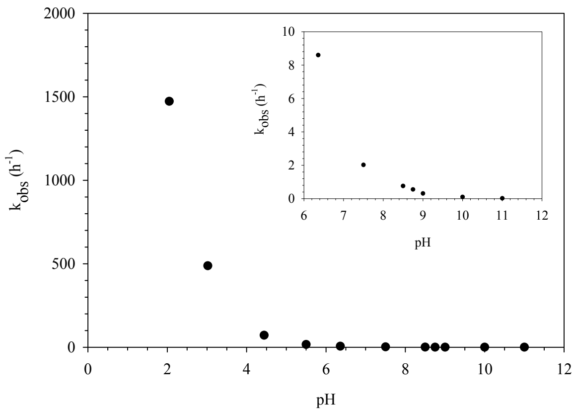
Figure 1 Observed first order loss rate coefficients for chlorpyrifos over the pH range of 2-11 in the presence of ECS. [\text{CP}]_0 = 0.5 \mu\text{M} , [\text{Buffer}]_T = 10 \text{ mM} , Temperature = 25 \pm 1^\circ\text{C} , and [\text{HOCl}]_T = 10 \mu\text{M} .
