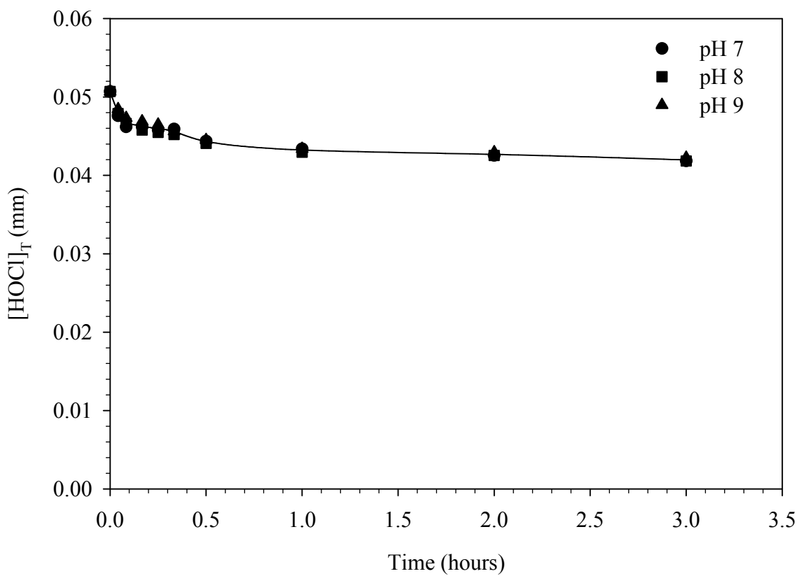
Figure 21 Chlorine demand of ACC water over the pH range of 7-9. [\text{HOCl}]_T = 50 \mu\text{M} , [\text{Buffer}]_T = 10 \text{ mM} , [\text{DOC}] = 1.1 \text{ mg-C/L} , and Temperature = 25 \text{ }^\circ\text{C} .
