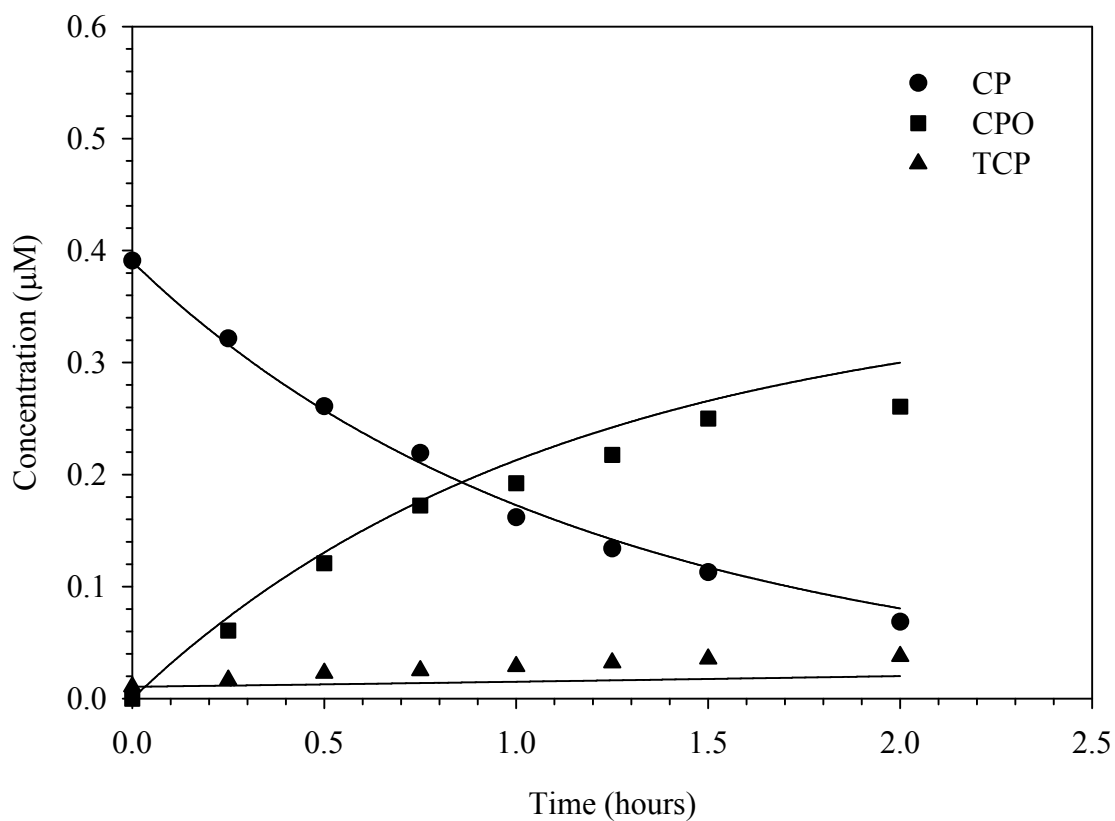
Figure 12 CP degradation in the presence of free chlorine at pH 8.0 in the absence of bromide. [CP]_0 = 0.39 \mu\text{M} , [\text{HOCl}]_T = 10 \mu\text{M} , [\text{PO}_4]_T = 10 \text{mM} , and Temperature = 25 °C. Lines represent model results.
