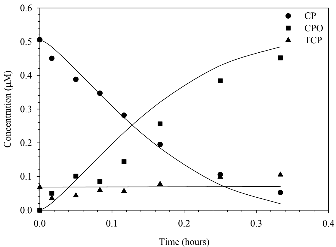
Figure 15 CP degradation in the presence of free chlorine and bromide at pH 8.0. [CP]_o = 0.51 \mu\text{M} , [\text{HOCl}]_T = 10 \mu\text{M} , [\text{Br}^-] = 1 \mu\text{M} , [\text{PO}_4]_T = 10 \text{mM} , and Temperature = 25 °C. Lines represent model results.
