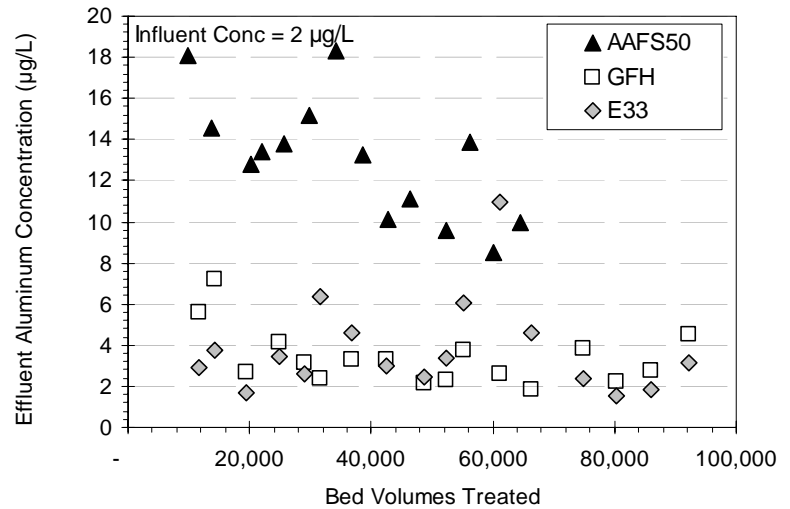
Figure 4-7. Breakthrough of V, P, Si, and Al from Rimrock, AZ Laboratory RSSCT Columns
