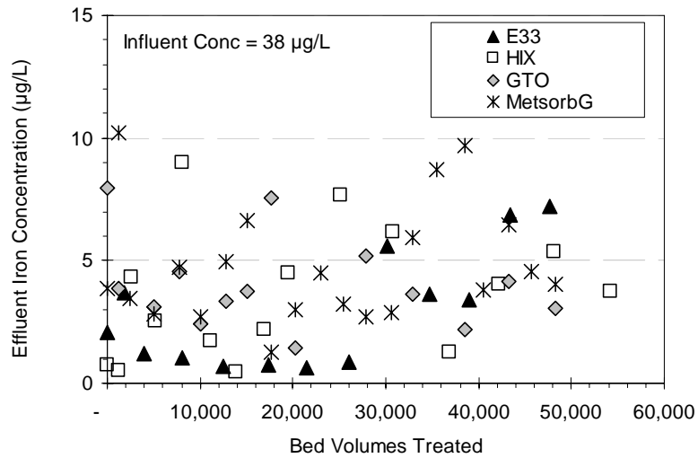
Figure 4-12. Breakthrough of U, V, Fe, and Mn from Lyman, NE Laboratory RSSCT Columns
