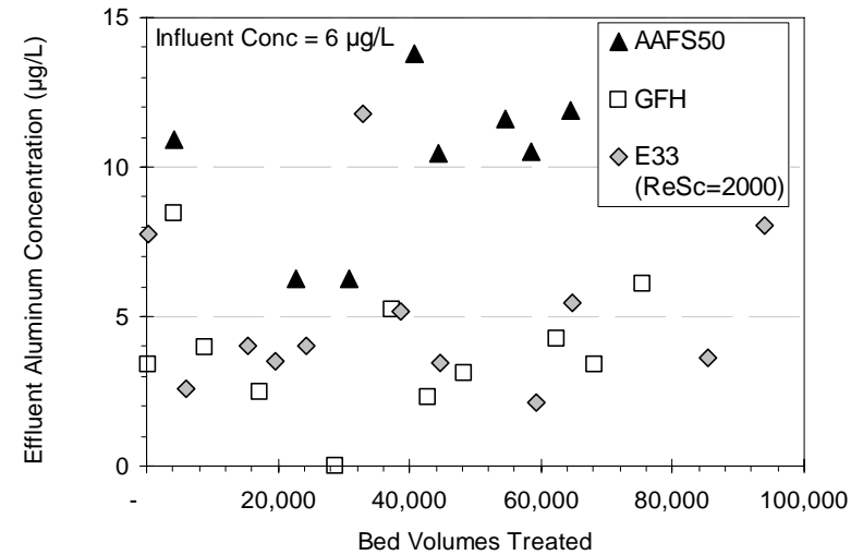
Figure 4-2. Breakthrough of V, P, Si, and Al from Field RSSCT Columns at Valley Vista, AZ
