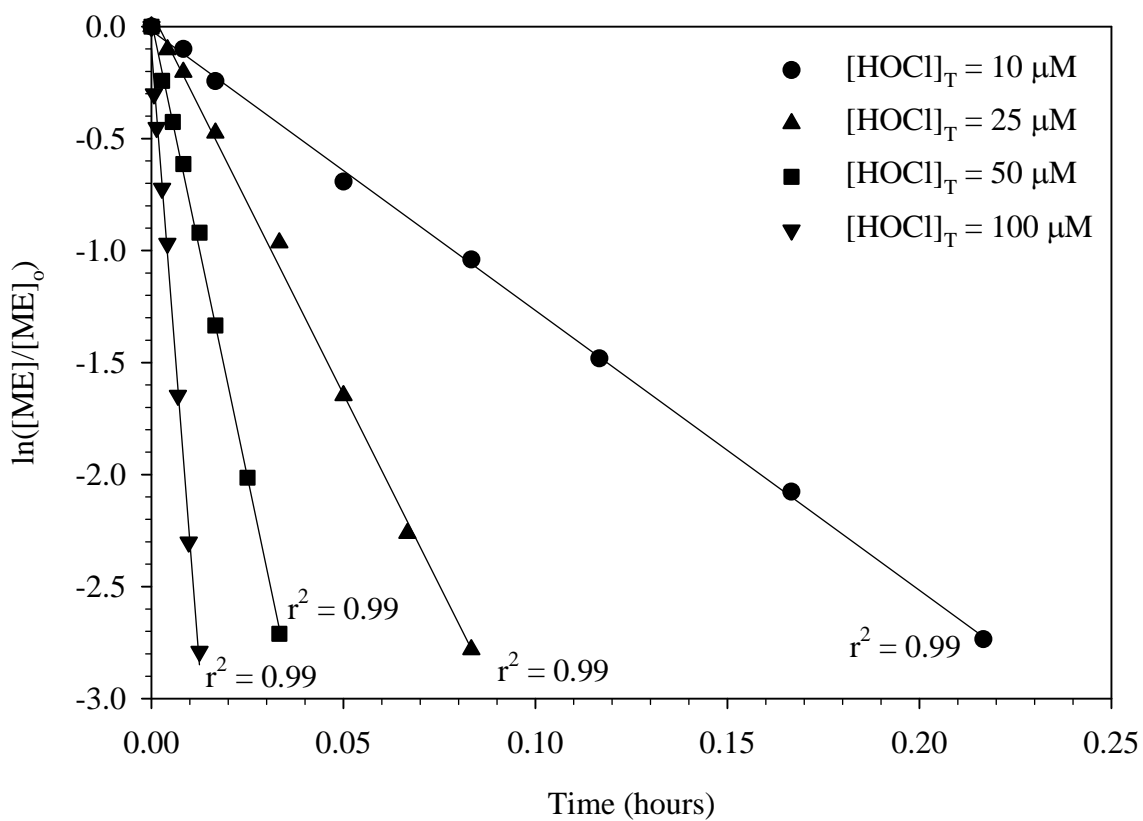
Figure 8 Observed first-order rate of ME loss in the presence of aqueous chlorine at pH 6.5. [\text{ME}]_0 = 0.5 \mu\text{M} , [\text{HOCl}]_0 = 10\text{-}100 \mu\text{M} , [\text{PO}_4]_T = 10 \text{ mM} , and Temperature = 25 \pm 1^\circ\text{C} . Experiments performed in triplicate.
