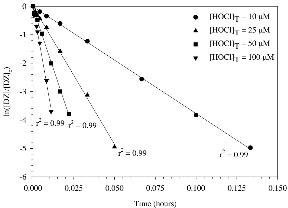
Figure 6 Observed first-order rate of DZ loss in the presence of aqueous chlorine at pH 6.5. [DZ]_0 = 0.5 \mu M , [HOCl]_0 = 10-100 \mu M , [PO_4]_T = 10 \text{ mM} , and Temperature = 25 \pm 1^\circ C . Experiments performed in triplicate.
