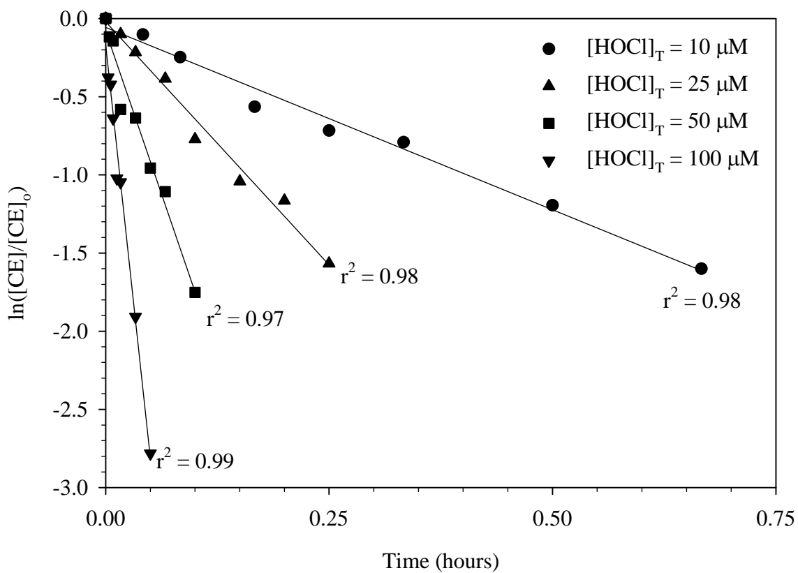
Figure 5 Observed first-order rate of CE loss in the presence of aqueous chlorine at pH 6.5. [CE]_0 = 0.5 \mu M , [HOCl]_0 = 10-100 \mu M , [PO_4]_T = 10 mM , and Temperature = 25 \pm 1^\circ C . Experiments performed in triplicate.
