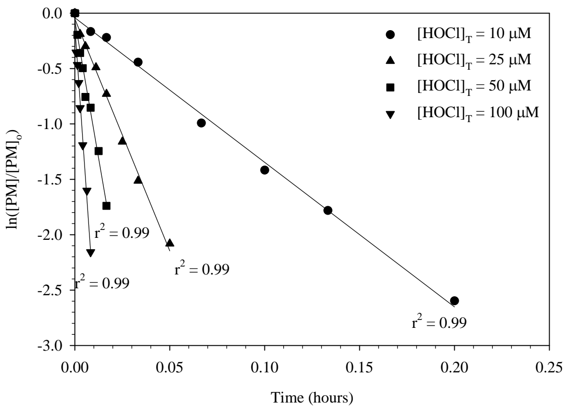
Figure 10 Observed first-order rate of PM loss in the presence of aqueous chlorine at pH 6.5. [\text{PM}]_0 = 0.5 \mu\text{M} , [\text{HOCl}]_0 = 10\text{-}100 \mu\text{M} , [\text{PO}_4]_{\text{T}} = 10 \text{mM} , and Temperature = 25 \pm 1^\circ\text{C} . Experiments performed in triplicate.
