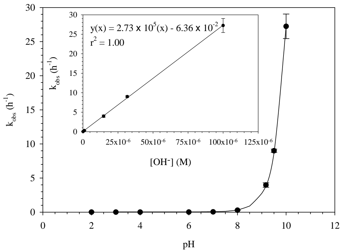
Figure 4 Hydrolytic behavior of phosmet (PM) over the pH range of 2-10. Insert: slope represents the alkaline hydrolysis rate coefficient. [PM]_0 = 0.5 \mu\text{M} , [\text{Buffer}]_T = 10 \text{ mM} , and Temperature = 25 \pm 1^\circ\text{C} . Error bars represent 95% confidence intervals.
