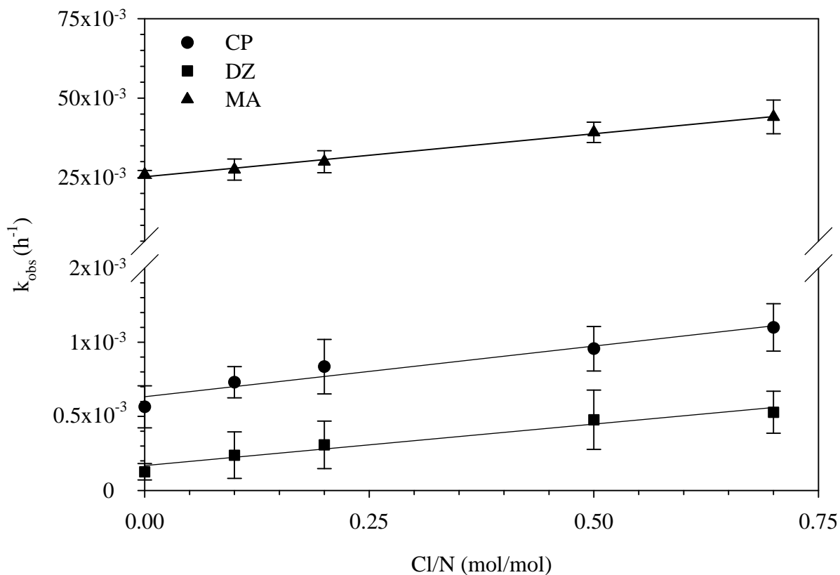
Figure 23 Observed first-order observed loss of three OP pesticides in the presence of monochloramine at pH 8.5. [NH_2Cl] = 50 \mu M , [OP]_o = 0.5 \mu M , Cl/N = 0-0.7 mol/mol, [H_3BO_3]_T = 10 mM, and Temperature = 25 \pm 1^\circ C . Error bars represent 95% confidence intervals.
