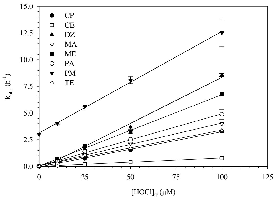
Figure 15 Second-order apparent rate coefficient for the OP pesticides at pH 9. [OP]_o = 0.5 \mu\text{M} , [\text{CO}_3]_T = 10 \text{ mM} , Temperature = 25 \pm 1^\circ\text{C} , and [\text{HOCl}]_T = 0\text{-}100 \mu\text{M} . Error bars represent 95% confidence intervals.
