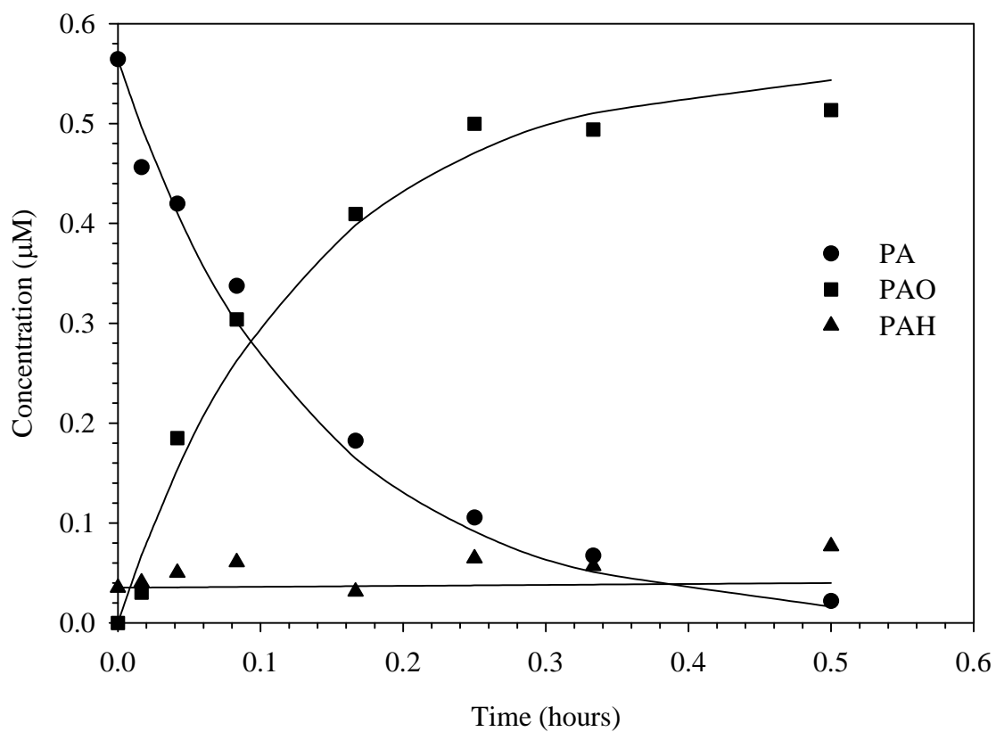
Figure 20 Experimental and model results for PA loss in the presence of chlorine at pH 8.0. [PA]_o = 0.57 \mu\text{M} , [HOCl]_T = 25 \mu\text{M} , [PO_4]_T = 10 \text{mM} , and Temperature = 25 \pm 1^\circ\text{C} . Lines represent model results.
