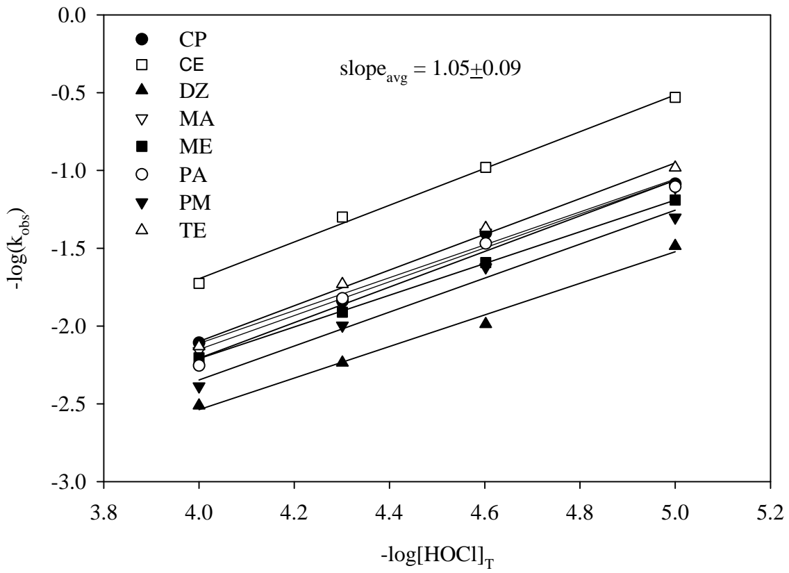
Figure 12 The reaction order of chlorine with 8 OP pesticides at pH 6.5. [\text{OP}]_0 = 0.5 \mu\text{M} , [\text{PO}_4]_T = 10 \text{ mM} , Temperature = 25 \pm 1^\circ\text{C} , and [\text{HOCl}]_T = 10\text{-}100 \mu\text{M} .
