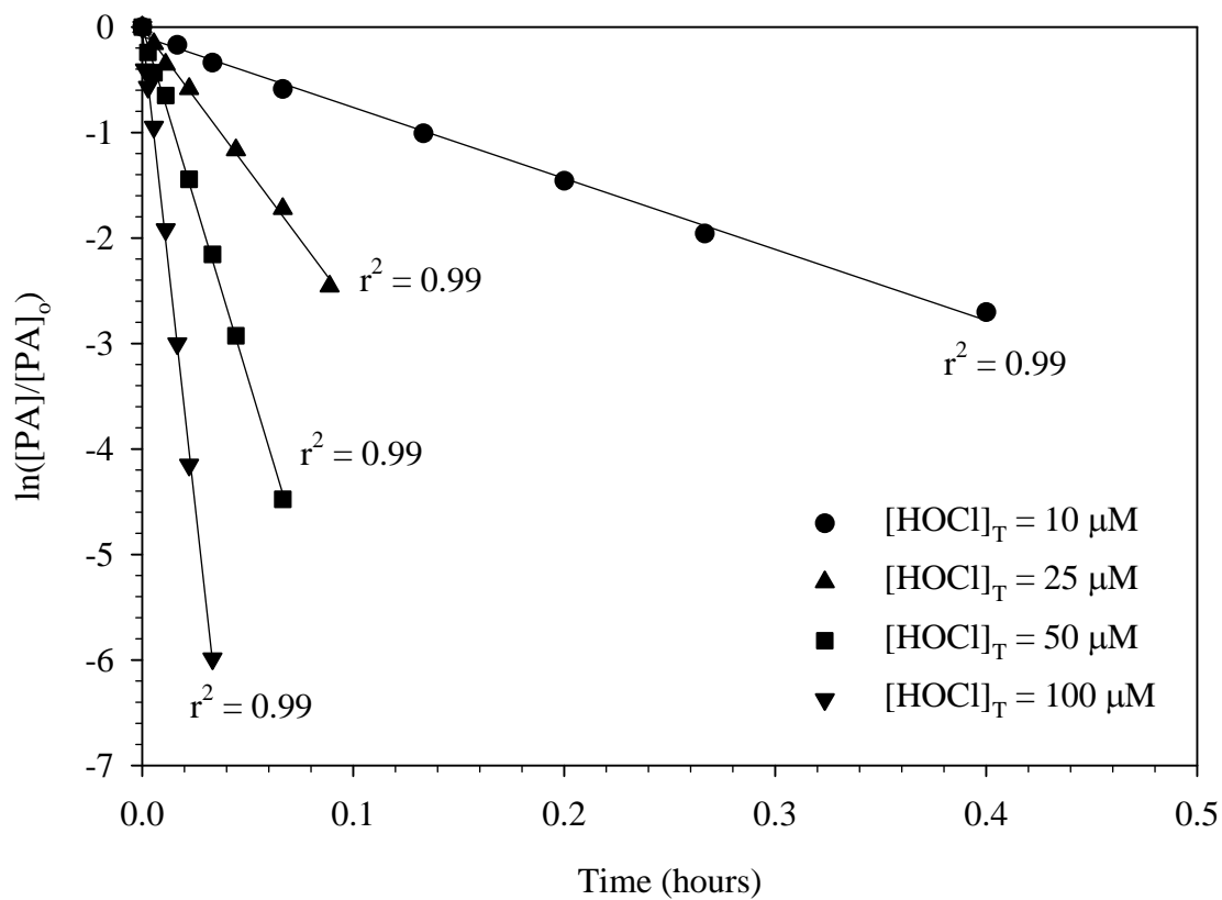
Figure 9 Observed first-order rate of PA loss in the presence of aqueous chlorine at pH 6.5. [PA]_0 = 0.5 \mu M , [HOCl]_0 = 10\text{-}100 \mu M , [PO_4]_T = 10 \text{ mM} , and Temperature = 25 \pm 1^\circ C . Experiments performed in triplicate.
