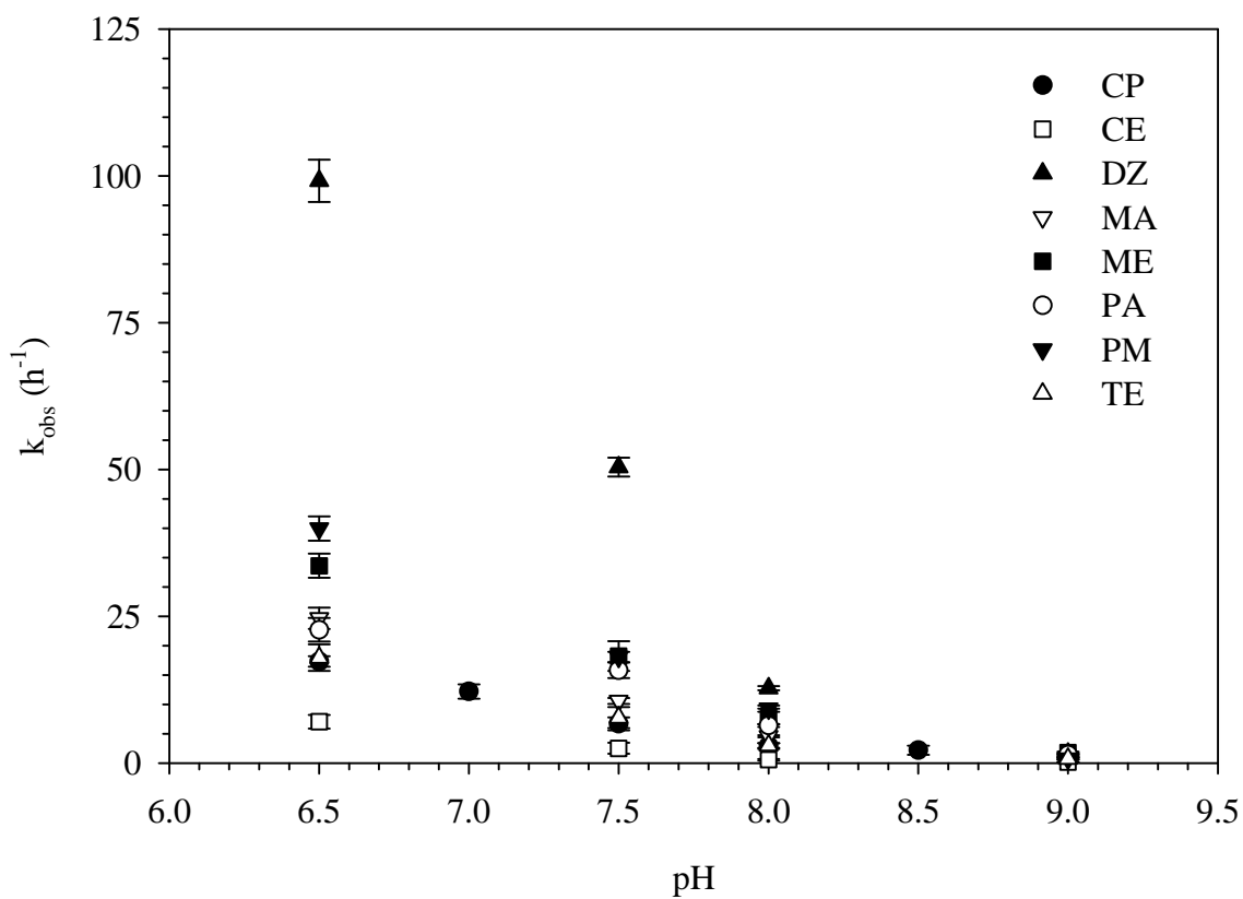
Figure 14 The pH dependency of the first-order observed rate coefficients for the OP pesticides. [\text{OP}]_0 = 0.5 \mu\text{M} , [\text{HOCl}]_T = 25 \mu\text{M} , [\text{Buffer}]_T = 10 \text{mM} , and Temperature = 25 °C. Error bars represent 95% confidence intervals.
