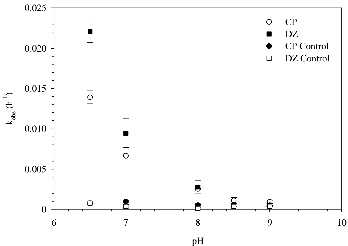
Figure 21 First-order observed loss of CP and DZ in the presence of monochloramine as a function of pH. [\text{NH}_2\text{Cl}] = 50 \mu\text{M} , [\text{OP}]_0 = 0.5 \mu\text{M} , \text{Cl/N} = 0.7 \text{ mol/mol} , [\text{Buffer}]_T = 10 \text{ mM} , Temperature = 25 \pm 1^\circ\text{C} , and pH 6.5-9.0. Error bars represent 95% confidence intervals.
