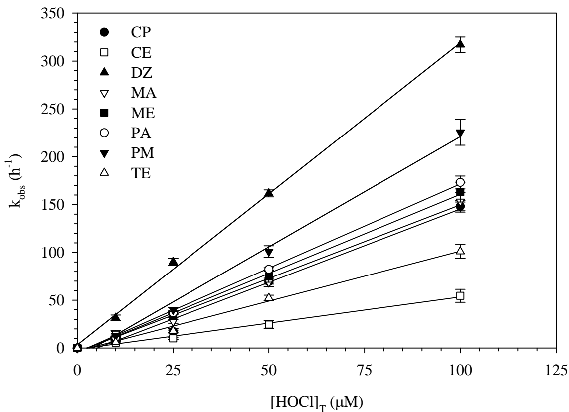
Figure 13 Second-order apparent rate coefficient for the OP pesticides at pH 6.5. [OP]_0 = 0.5 \mu\text{M} , [PO_4]_T = 10 \text{ mM} , Temperature = 25 \pm 1^\circ\text{C} , and [HOCl]_T = 0\text{-}100 \mu\text{M} . Error bars represent 95% confidence intervals.
