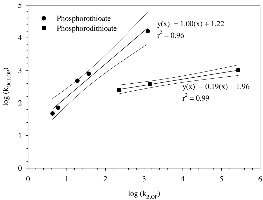
Figure 17 Relationship between the k_{OCl,OP} with alkaline hydrolysis rate coefficient as a function of OP pesticide subgroup. Error bars about the regression line represent 95% confidence intervals.
