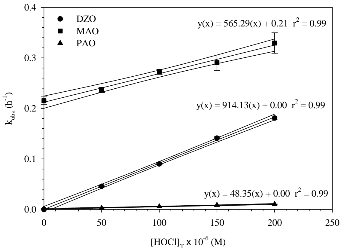
Figure 18 Second-order apparent rate coefficient of 3 OP pesticide oxons at pH 9. [OP]_o = 0.5 \mu\text{M} , [\text{CO}_3]_T = 10 \text{ mM} , Temperature = 25 \pm 1^\circ\text{C} , and [\text{HOCl}]_T = 0\text{-}200 \mu\text{M} . Error bars represent 95% confidence intervals for both data points and regression lines.
