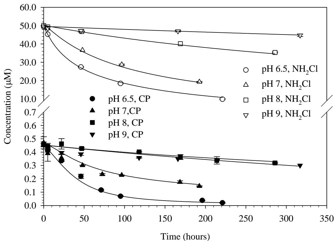
Figure 24 Experimental and model results for CP loss in the presence of monochloramine. [CP]_0 = 0.5 \mu\text{M} , [\text{NH}_2\text{Cl}]_0 = 50 \mu\text{M} , \text{Cl}/\text{N} = 0.7 \text{ mol/mol} , [\text{Buffer}]_T = 10 \text{ mM} , pH 6.5-9, and Temperature = 25 \pm 1^\circ\text{C} . Error bars represent 95% confidence intervals. Lines represent model results.
