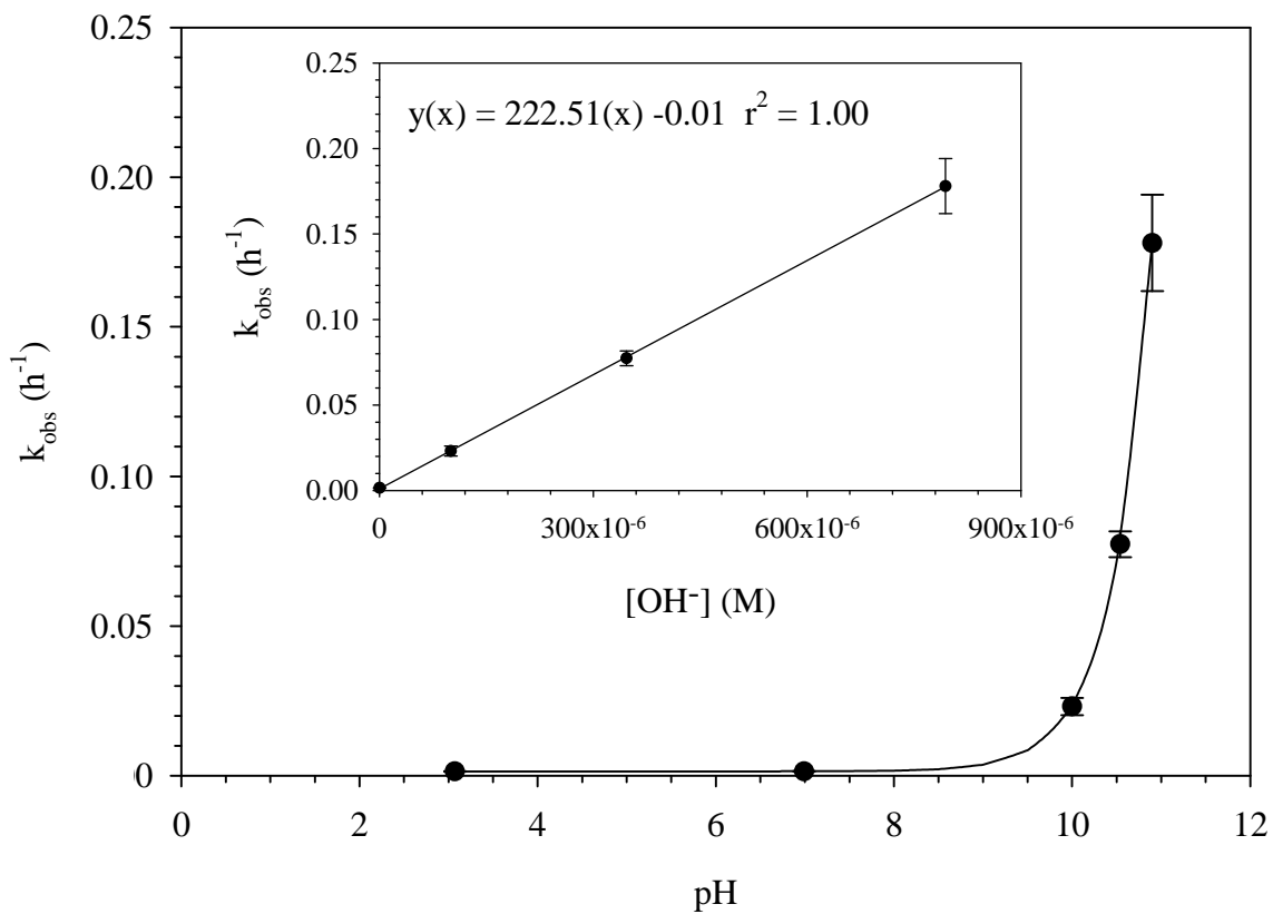
Figure 3 Hydrolytic behavior of methidathion (ME) over the pH range of 3-11. Insert: slope represents the alkaline hydrolysis rate coefficient. [ME]_o = 0.5 \mu\text{M} , [\text{Buffer}]_T = 10 \text{ mM} , and Temperature = 25 \pm 1^\circ\text{C} . Error bars represent 95% confidence intervals.
