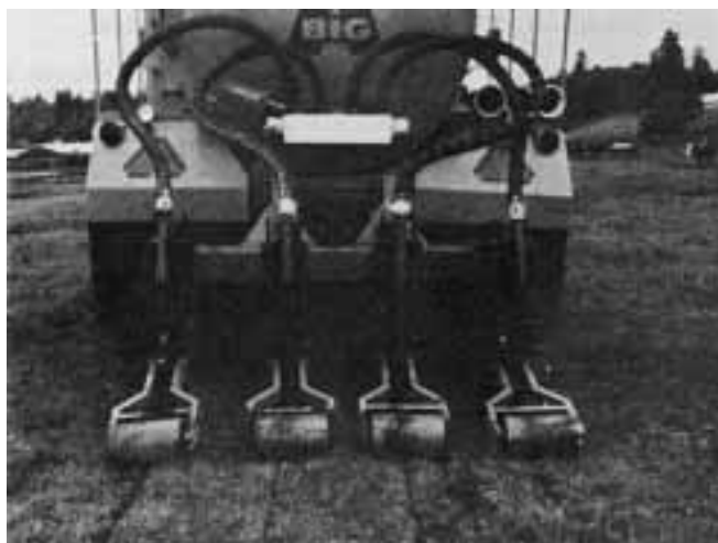
Figure 14-10. Tank truck with liquid sludge grassland injectors (courtesy of Rickel Manufacturing Company).
