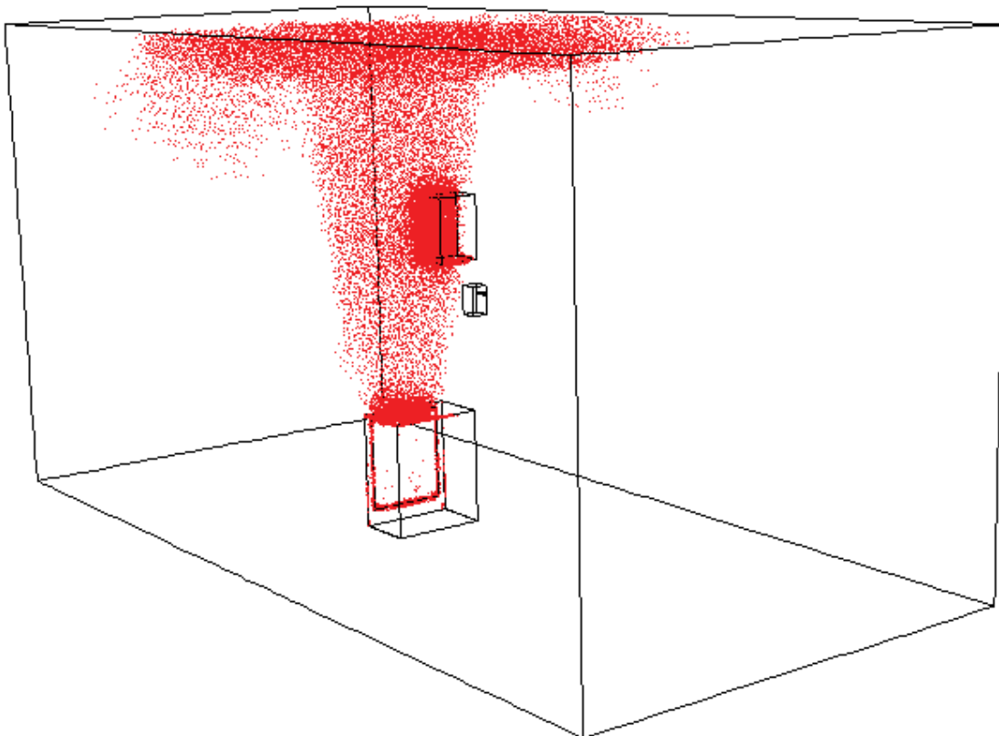
Figure B-4. Cells From the Base Mesh Marked for Adaptive Refinement
