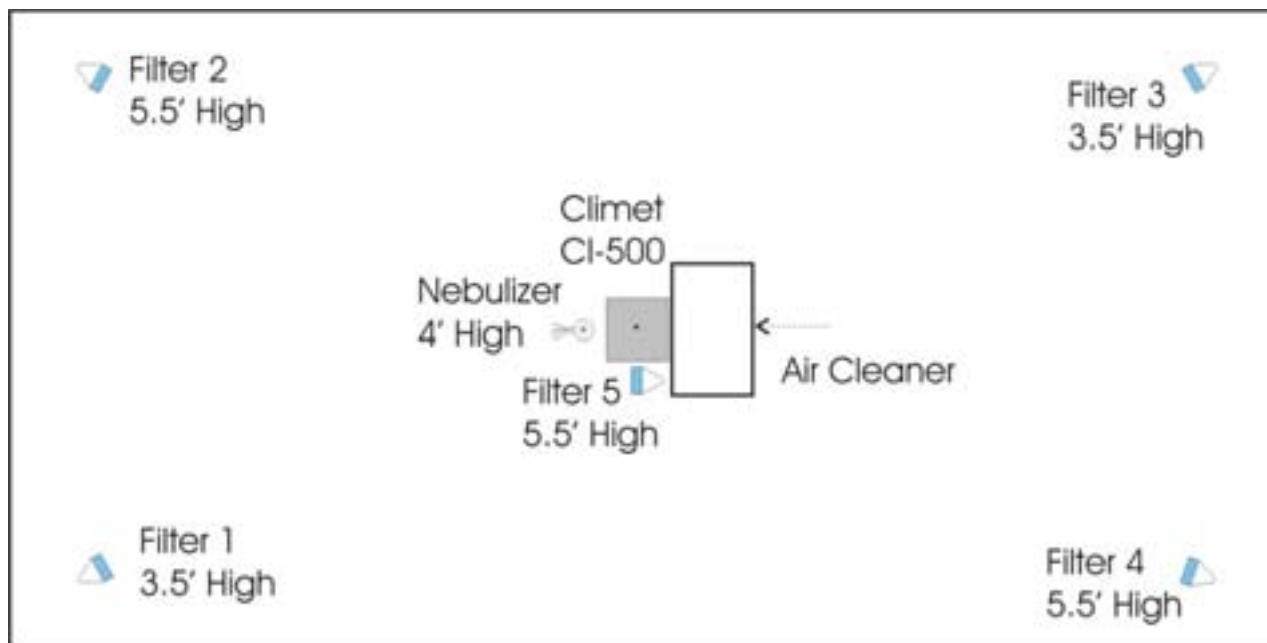
Figure 16. In-Room Test Configuration A
