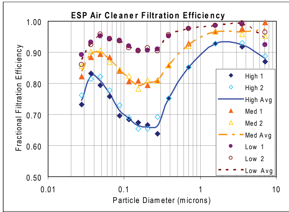
Figure 9. Filtration Efficiency for the ESP Air Cleaner
