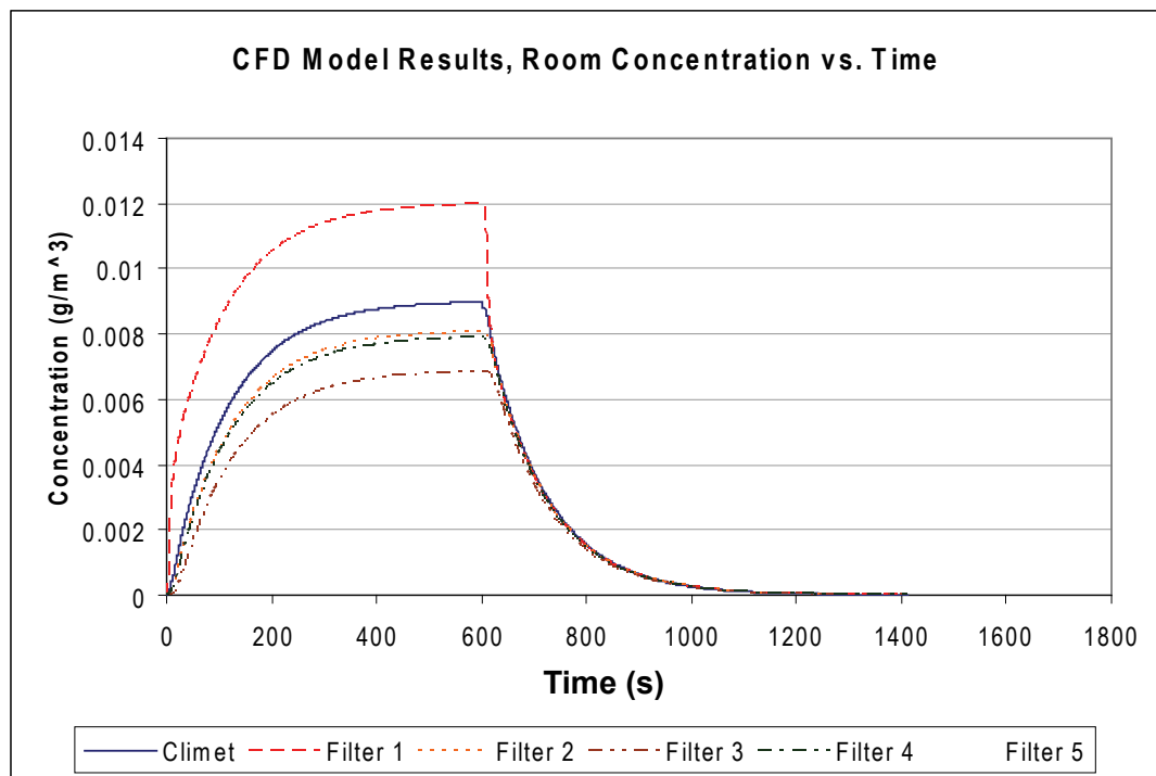
Figure B-11. KCl Concentration versus Time
