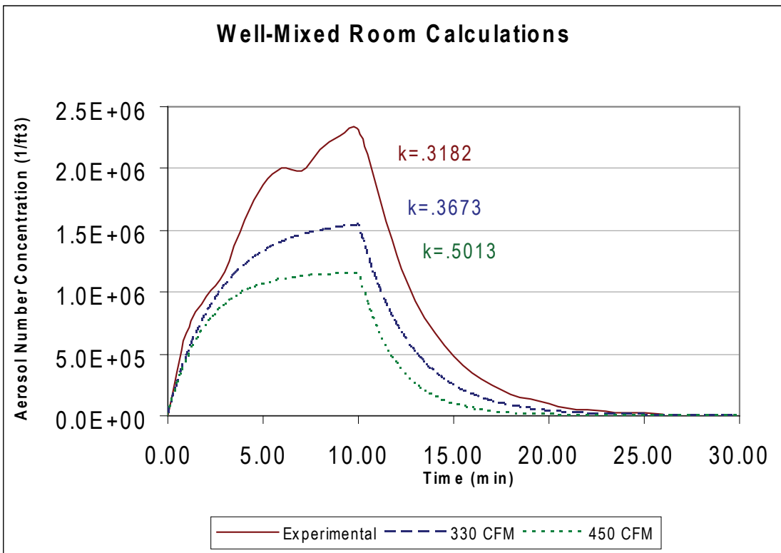
Figure 25. Well-Mixed Zone Model Results
