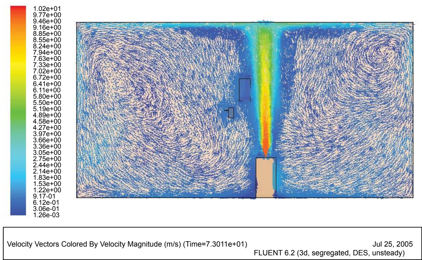
Figure B-5. Velocity Vector Flow Field
