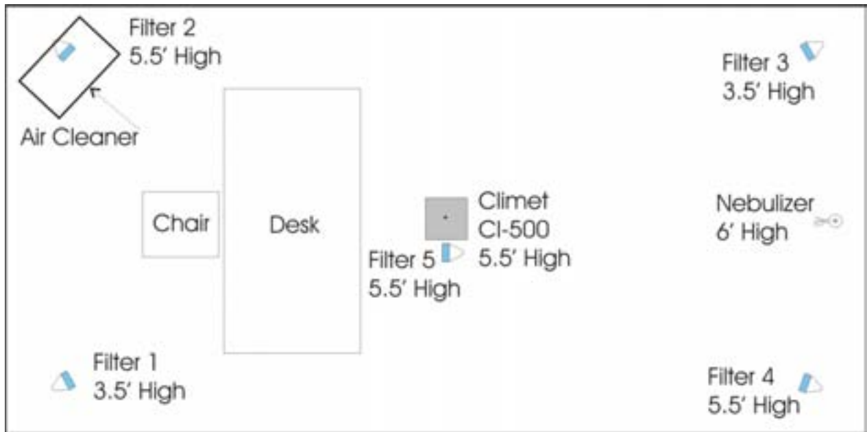
Figure 18. In-Room Test Configuration C
