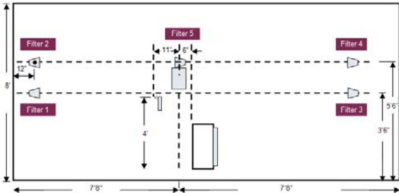
Figure B-2b. Model Dimensions (Side View)
