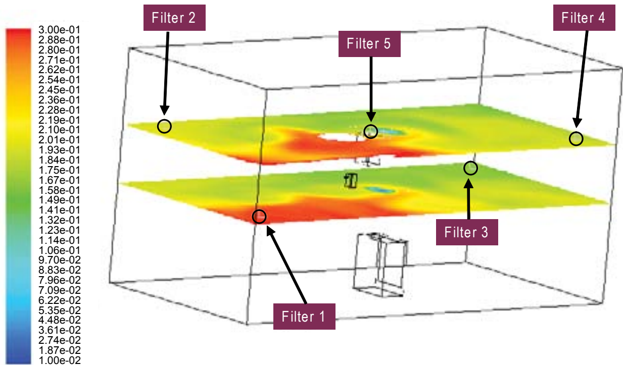
Figure B-8. KCl Concentration With Nebulizer at 10 Minutes of Operation (Cont'd)
