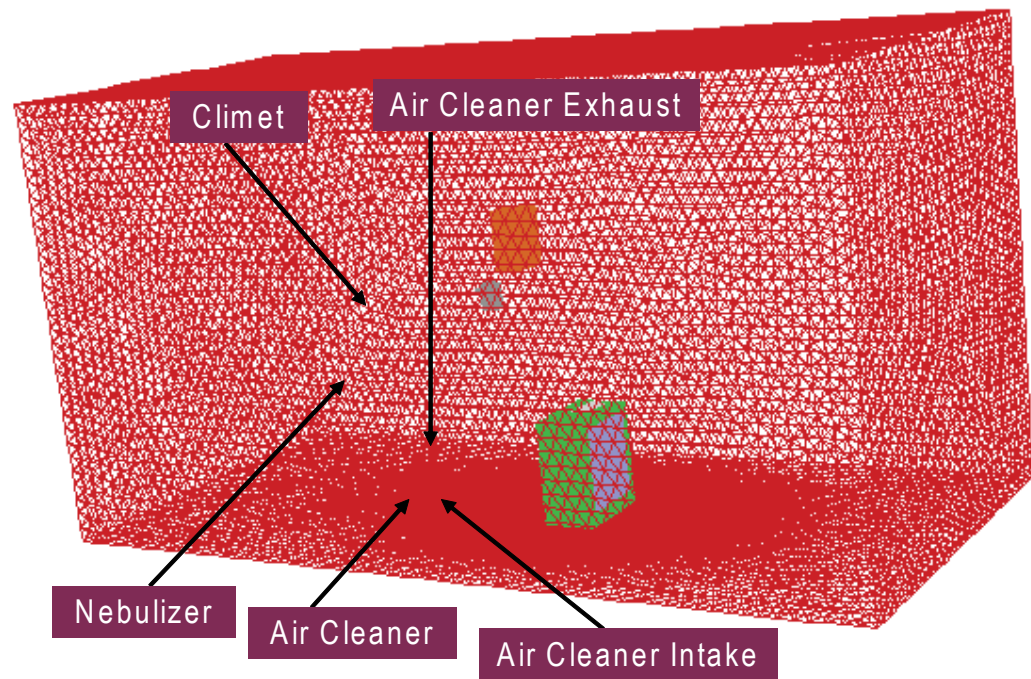
Figure B-3. Model Mesh with Outlines of Face Cells Illustrated
