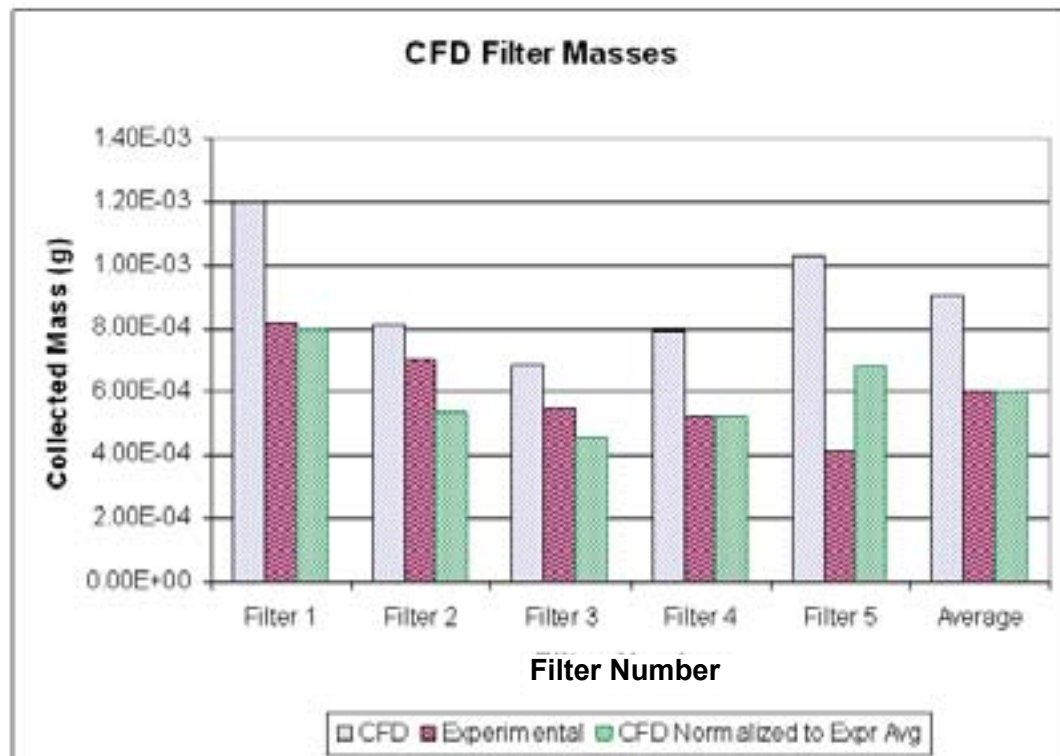
Figure B-12. Collected Mass of KCl in Filters
