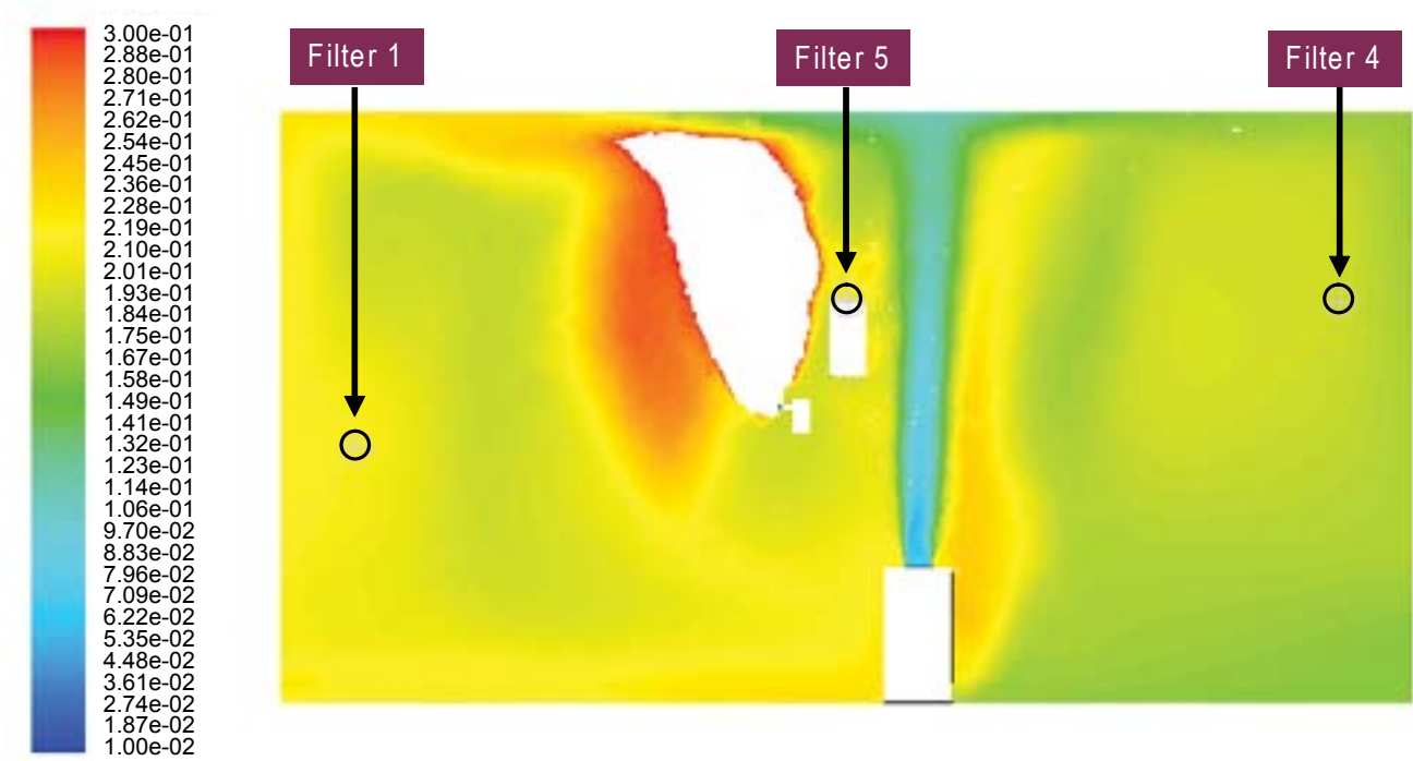
Figure B-7. KCl Concentration With Nebulizer at 10 Minutes of Operation
