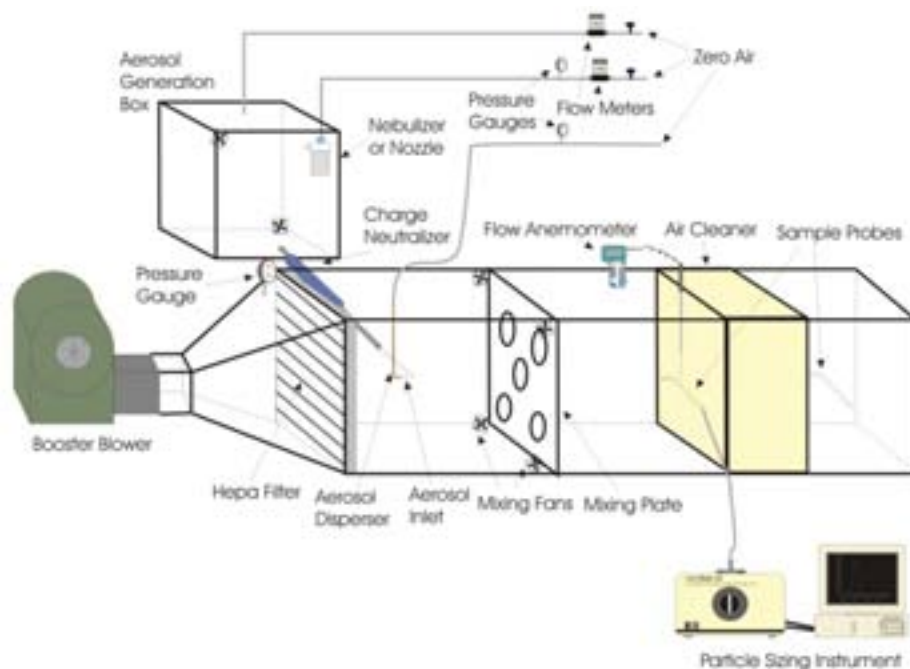
Figure 2. Schematic of the Single-Pass Efficiency Test Apparatus
