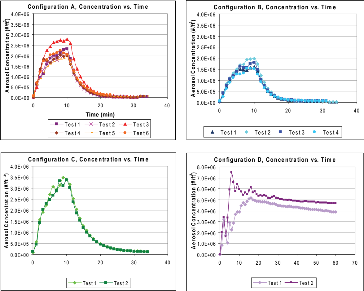
Figure 19. Concentration vs. Time Plots, Individual Configurations
