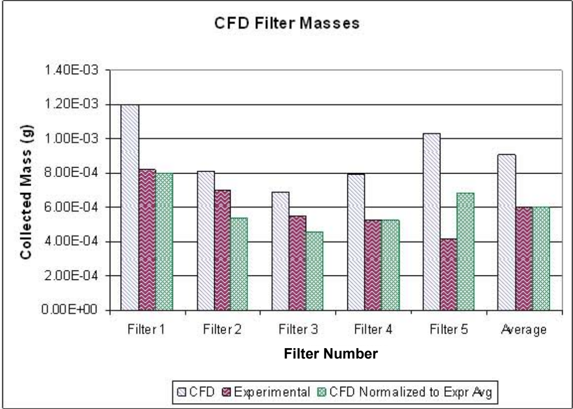
Figure 24. Filter Masses from CFD Calculations
