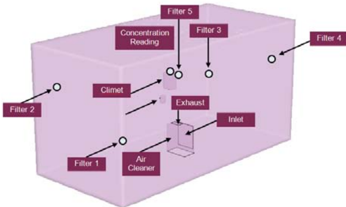
Figure B-1. Model Geometry
