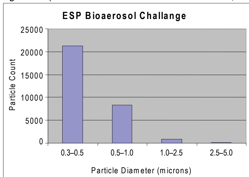
Figure 14. Upstream Particle Counts From ESP Bioaerosol Test, Run 2
