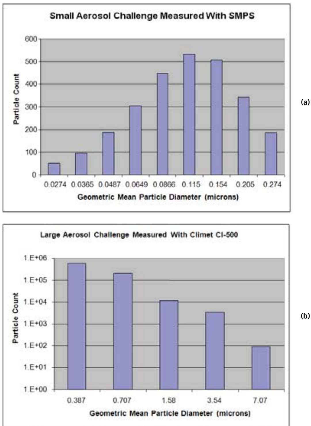
Figure 5. Representative Diameter Distributions of Test Aerosols Obtained Using TSI SMPS (a) and Climet CI-500 (b)
