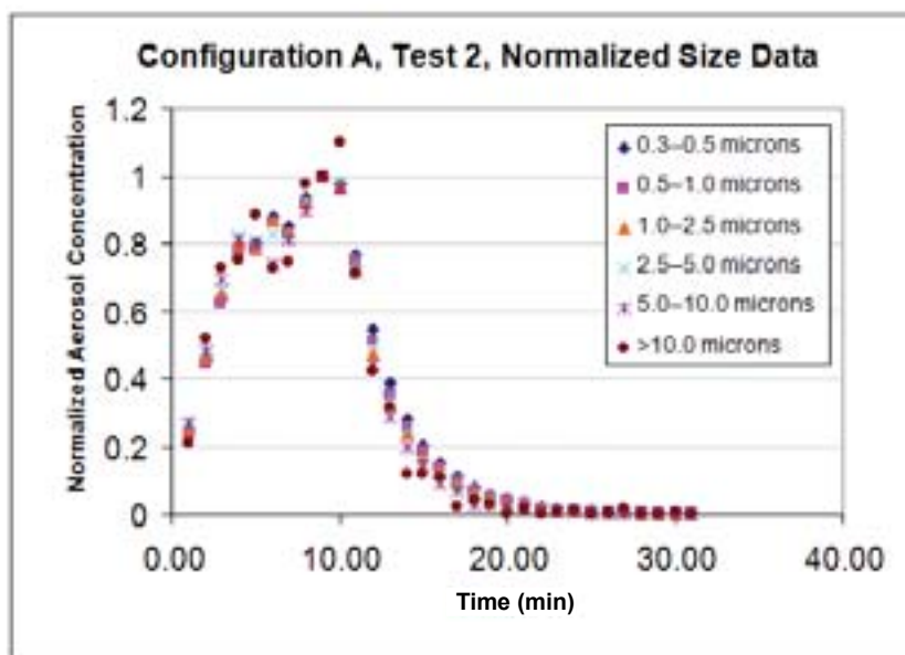
Figure 21. Size Resolved Concentration vs. Time
