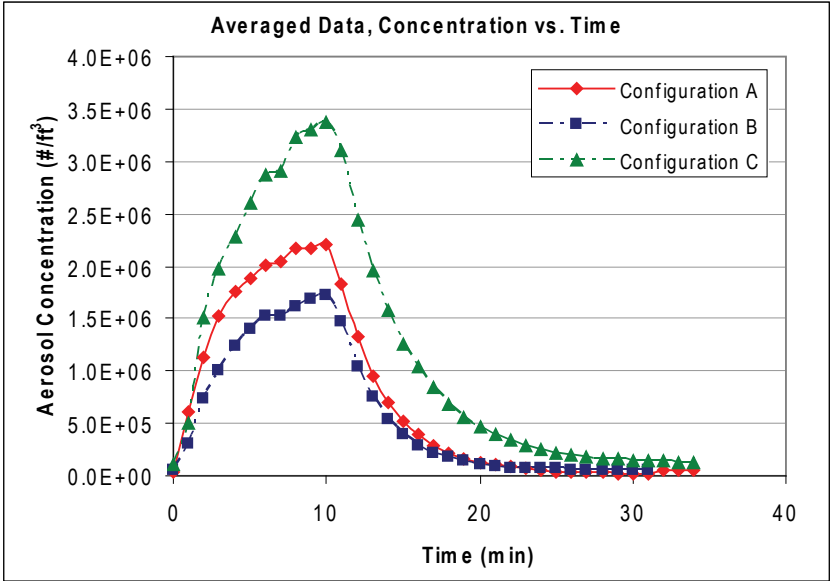
Figure 20. Concentration vs. Time Plot, Averaged Data
