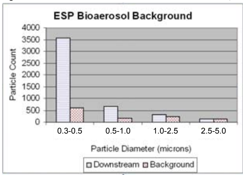
Figure 13. Downstream Particle Counts From ESP Bioaerosol Test, Run 2
