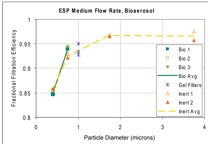
Figure 11. ESP Bioaerosol Filtration Efficiency
