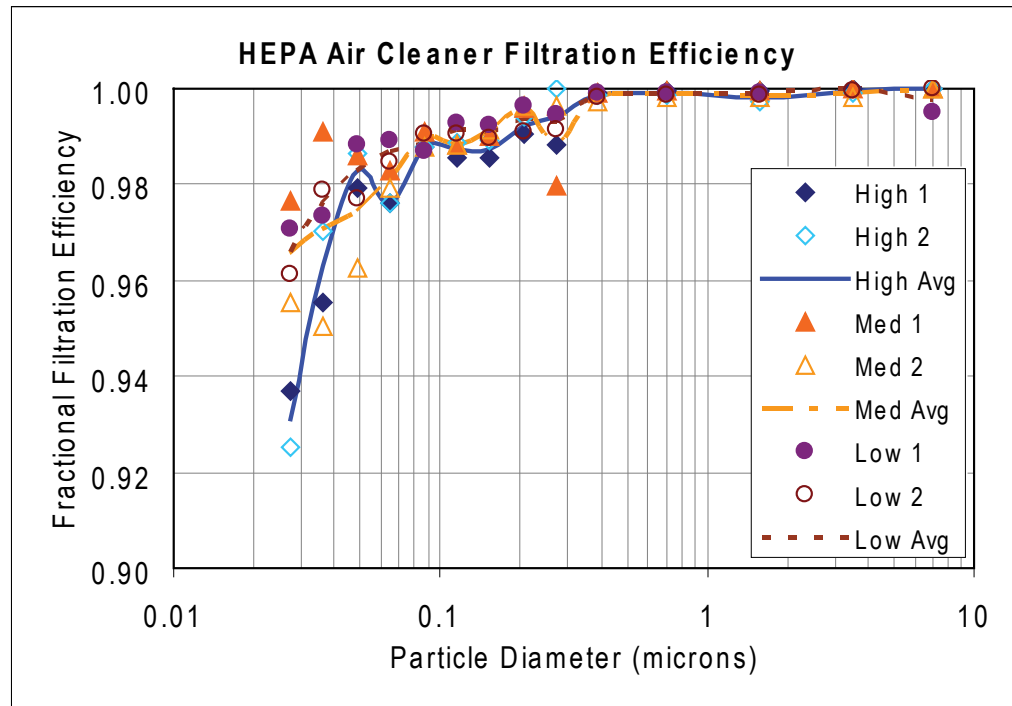
Figure 10. Filtration Efficiency for the HEPA Filter
