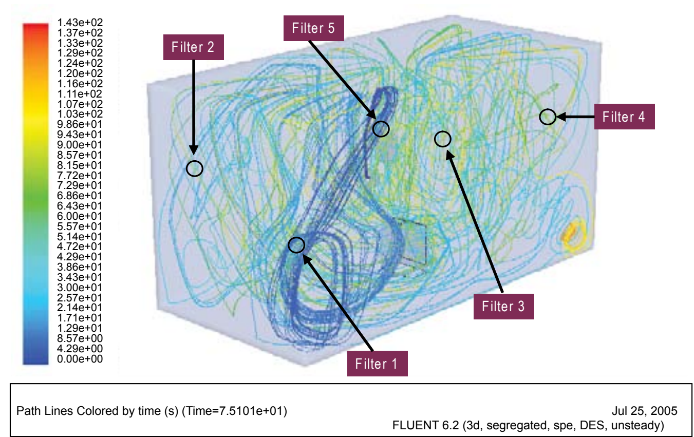
Figure B-6. Updated Pathlines (Colored by Total Residence Time)
