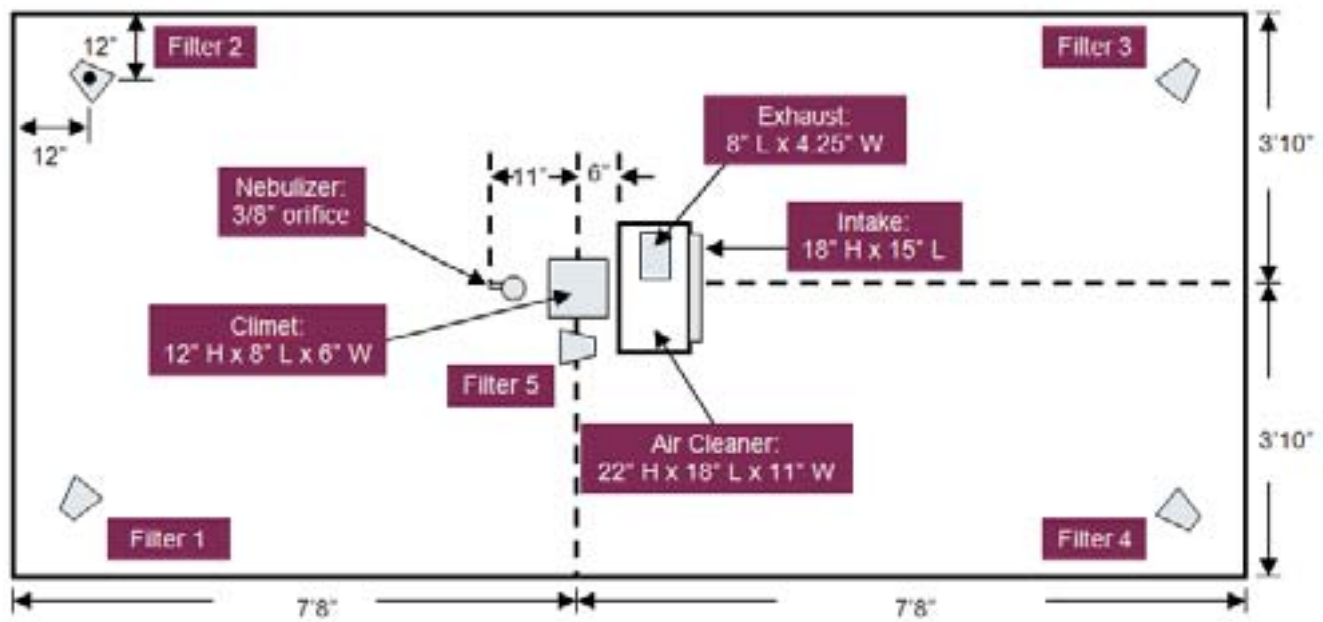
Figure B-2a. Model Dimensions (Plan View)
