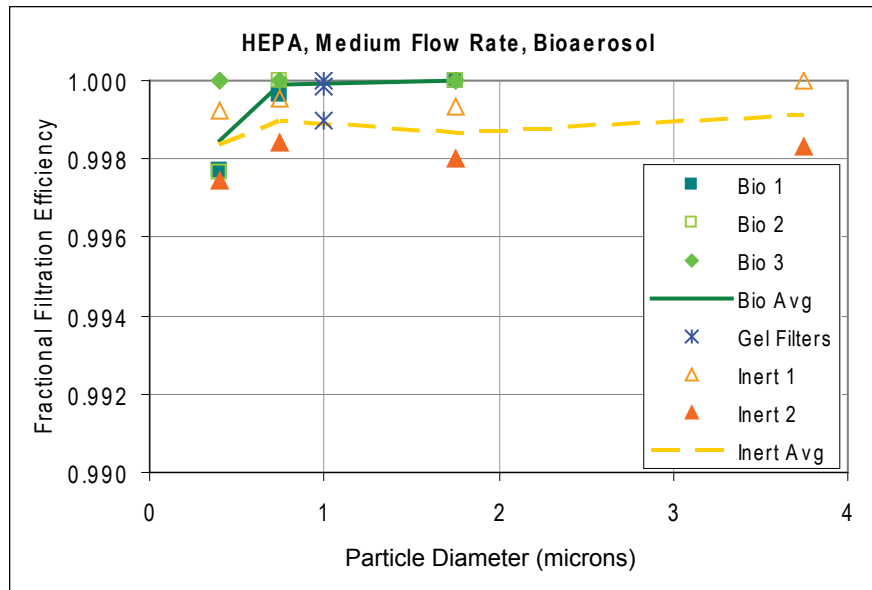
Figure 12. HEPA Bioaerosol Filtration Efficiency
