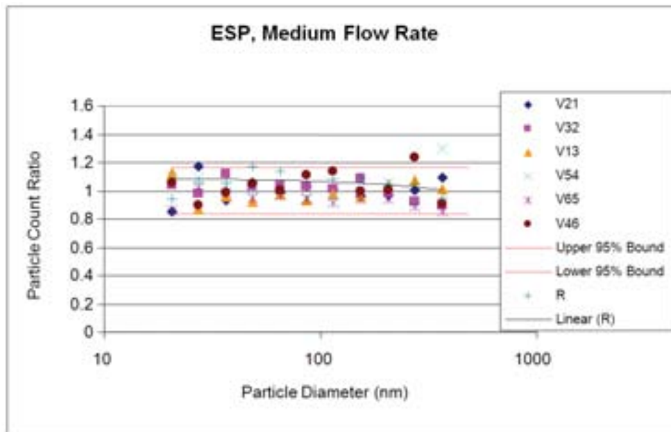
Figure 6. Plots of Bias Correction Factor ( R ) and Sampling Variability ( V )
