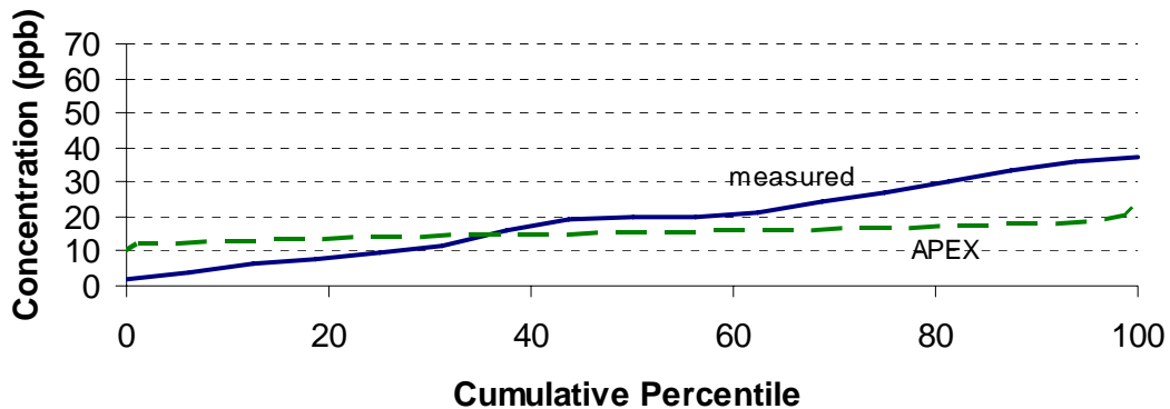
Weekly Average Indoor Ozone Concentration --Lake Arrowhead, Week of 7/12/95--
