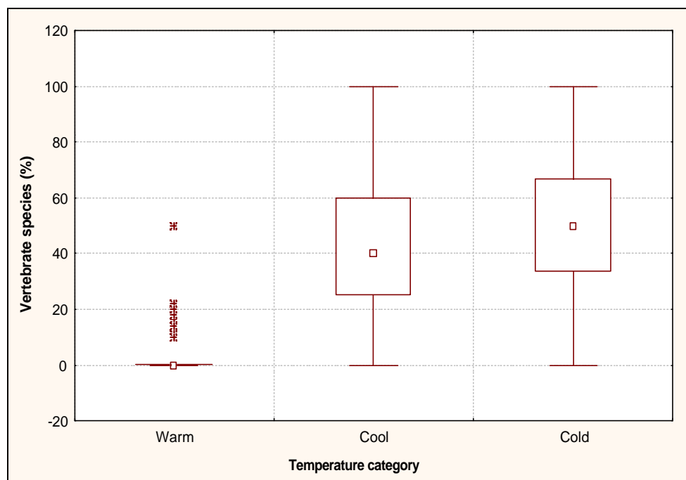
Figure 28. Percent of vertebrate species within each temperature guild. (percentages based on site relative abundance expanded by site weighting factor). Median, 75-25% quartiles, and non-outlier min-max, shown with inner box, outer box, and bars.
