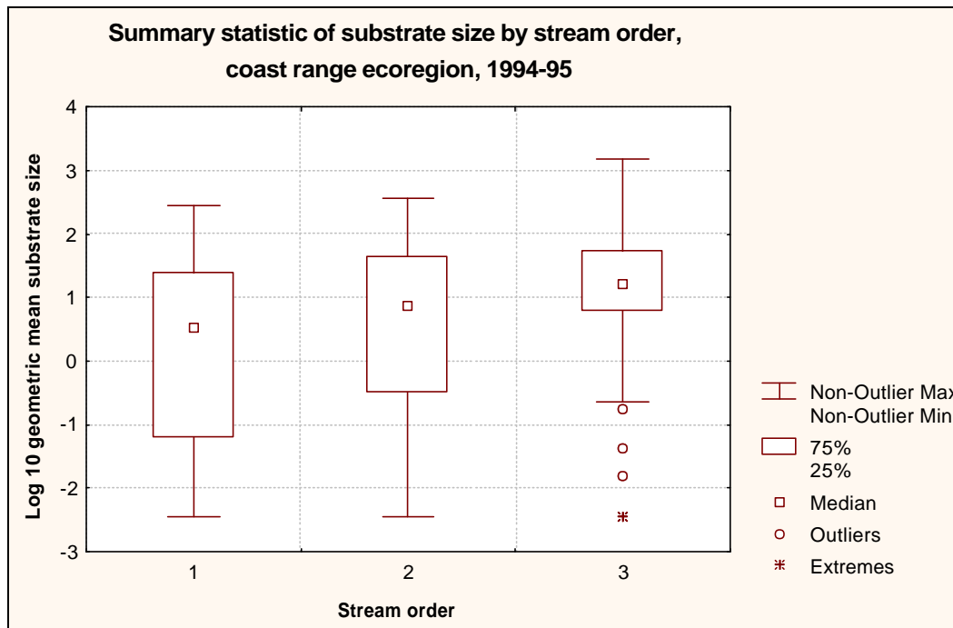
Figure 7. Summary of substrate size by stream order expressed as geometric mean (log10).
