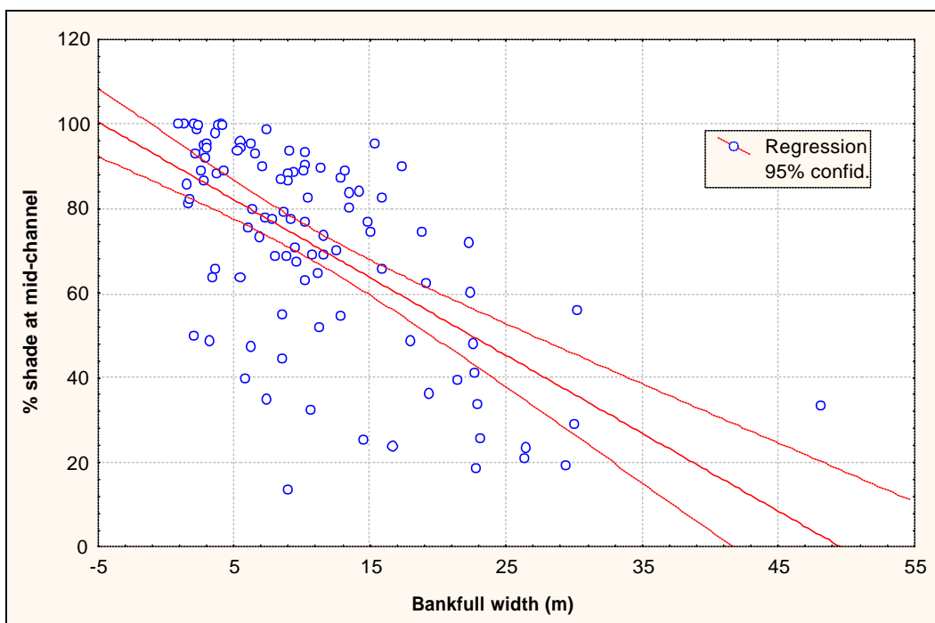
Figure 14. Relation of mid-channel shade to stream width ( r = -.62 ).
