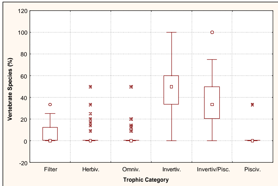
Figure 31. Percent of vertebrate species within each trophic guild, Coast Range ecoregion (1994-95) (percentages based on site relative abundance expanded by site weighting factor). Median, 75-25% quartiles, and non-outlier min-max, shown with inner box, outer box, and bars.
