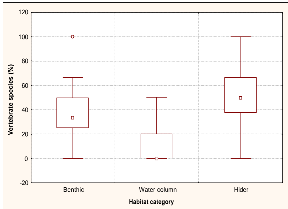
Figure 30. Percent of vertebrate species within each habitat guild, Coast Range ecoregion (1994-95) (percentages based on site relative abundance expanded by site weighting factor). Median, 75-25% quartiles, and non-outlier min-max, shown with inner box, outer box, and bars.
