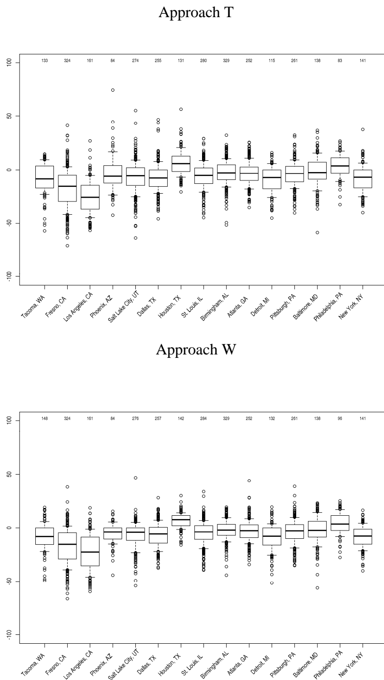
Figure F-2. Box and Whisker Plot of the Percent Difference in Calculated Hourly PM 2.5 Light Extinction between Approach T and the UFVA Approach (top plot) and between Approach W and the UFVA Approach (bottom plot) by Urban Study Area
