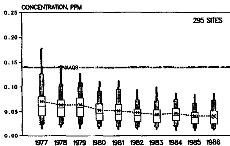
Figure 1-7. National boxplot trend in second highest 24-hour \text{SO}_2 concentrations, 1977 - 1986.
