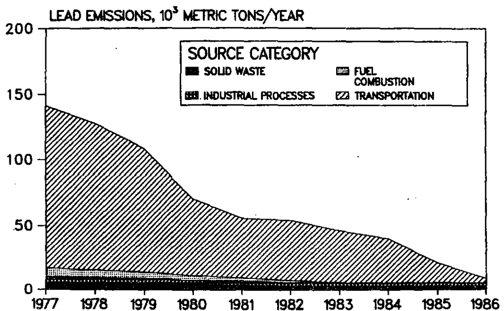
Figure 3-36. National trend in lead emissions, 1977-1986.
