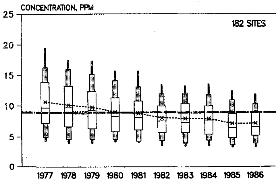
Figure 3-18. Boxplot comparisons of trends in second highest nonoverlapping 8-hour average carbon monoxide concentrations at 182 sites, 1977-1986.
