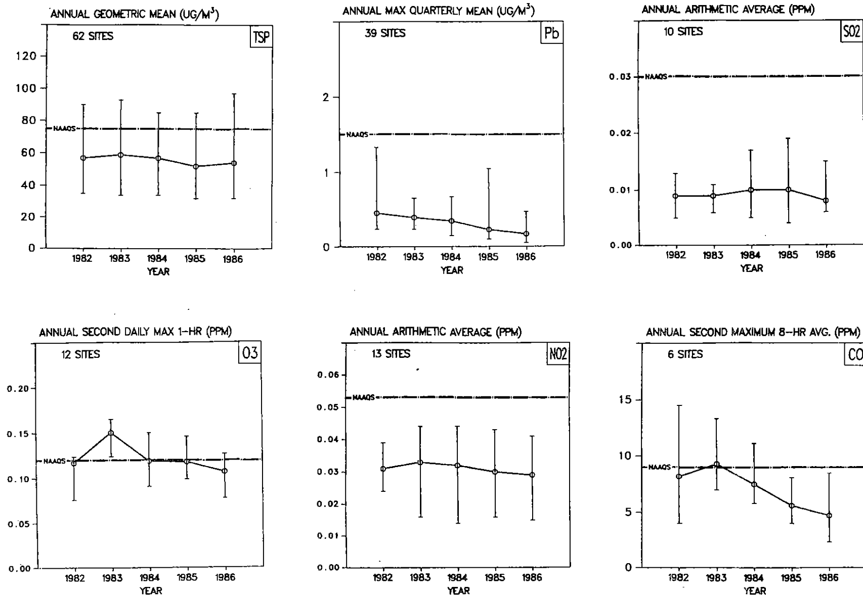
Figure 5-7. Air Quality Trends in the Composite Mean and Range of Pollutant-Specific Statistics for the Chicago, IL-IN Urbanized Area, 1982-1986.
