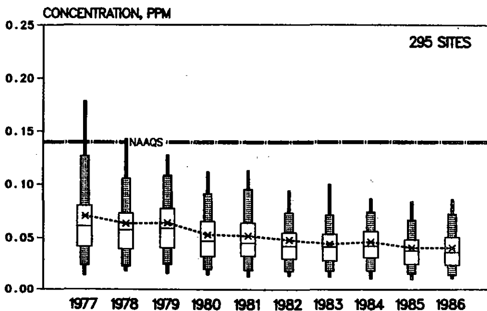
Figure 3-12. Boxplot comparisons of trends in second highest 24-hour average sulfur dioxide concentrations at 295 sites, 1977-1986.
