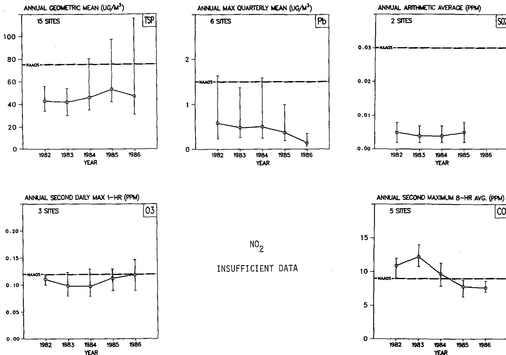
Figure 5-14. Air Quality Trends in the Composite Mean and Range of Pollutant-Specific Statistics for the Portland, OR-WA Urbanized Area, 1982-1986.
