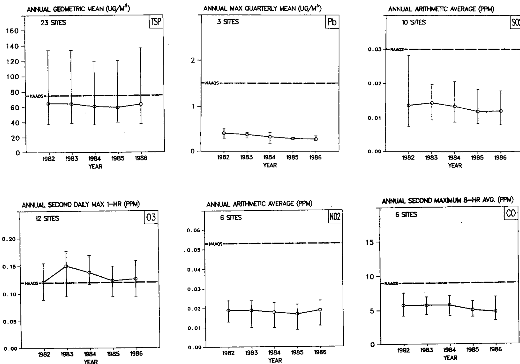
Figure 5-10. Air Quality Trends in the Composite Mean and Range of Pollutant-Specific Statistics for the St. Louis, MO-IL Urbanized Area, 1982-1986.
