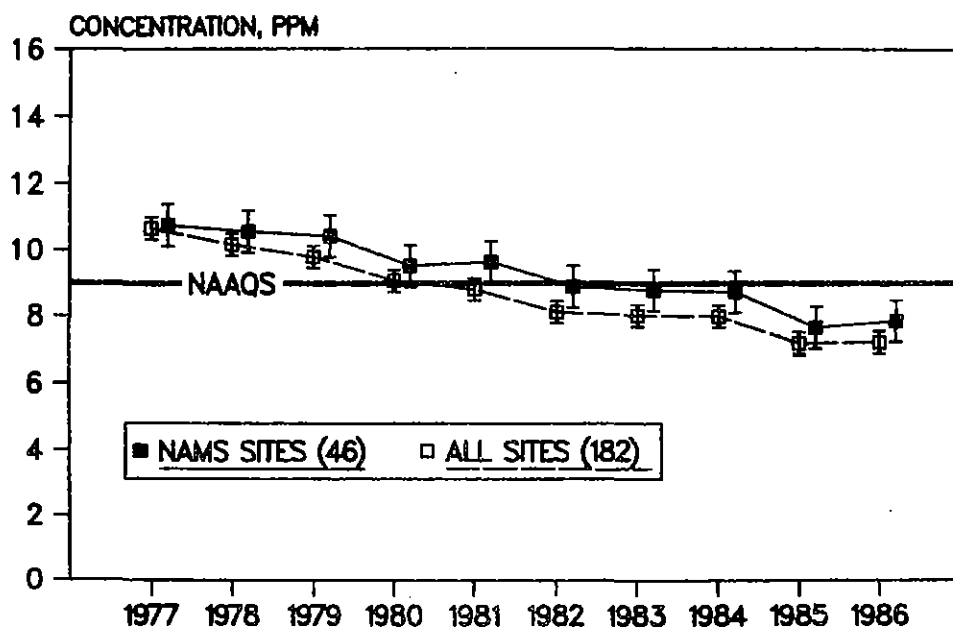
Figure 3-17. National trend in the composite average of the second highest nonoverlapping 8-hour average carbon monoxide concentration at both NAMS and all sites with 95 percent confidence intervals, 1977-1986.
