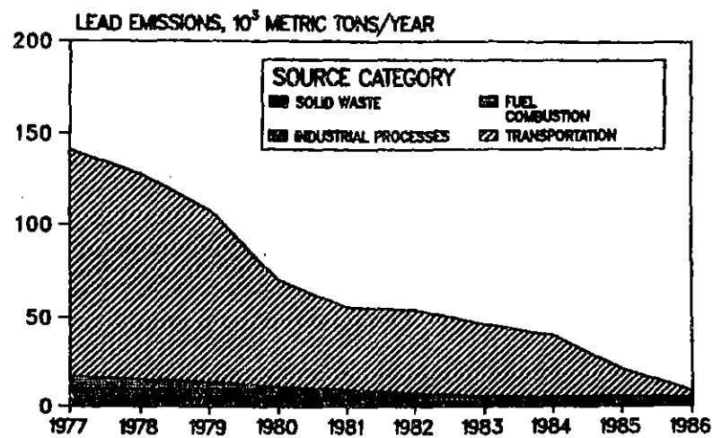
Figure 1-23. National trend in lead emissions, 1977 - 1986.
