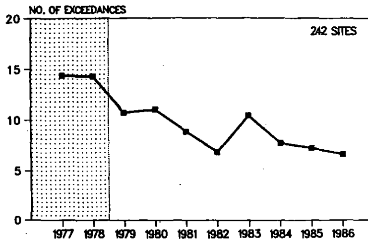
Figure 1-20. National trend in the composite average of the number of daily exceedances of the O 3 NAAQS in the O 3 season, 1977 - 1986.
