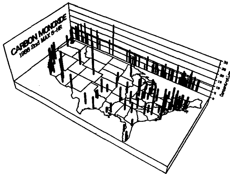
Figure 1-14. United States map of the highest second maximum nonoverlapping 8-hour average CO concentration by MSA, 1986.
