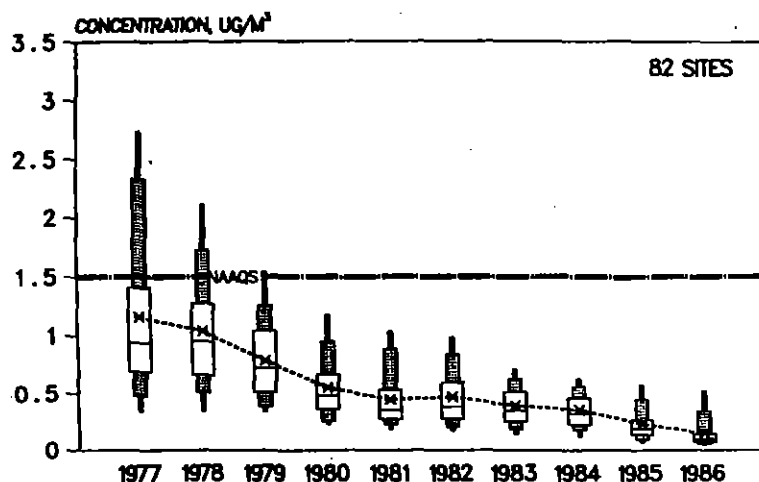
Figure 1-22. National boxplot trend in maximum quarterly average Pb concentrations, 1977 - 1986.
