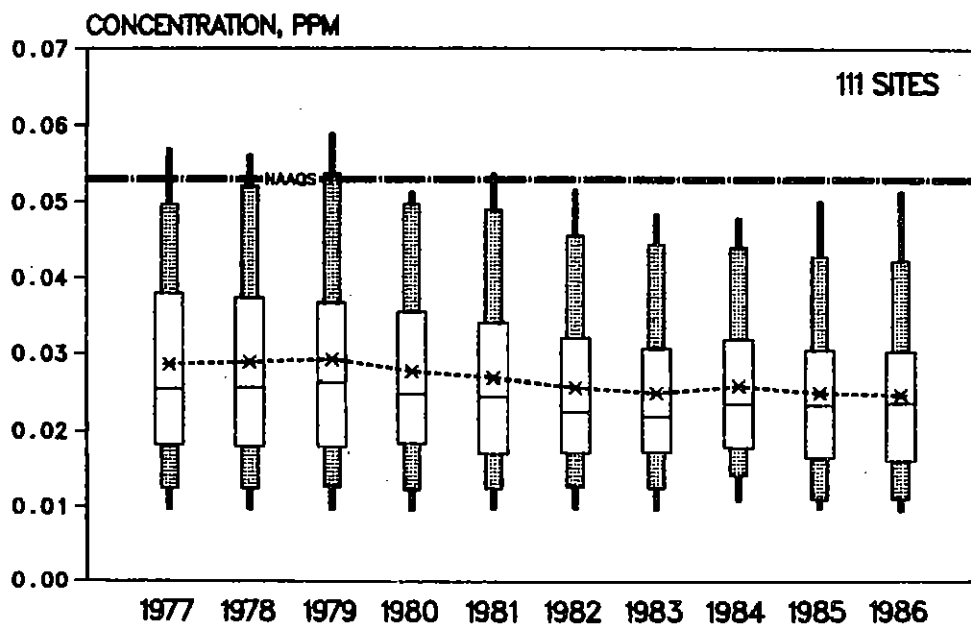
Figure 3-24. Boxplot comparisons of trends in annual mean nitrogen dioxide concentrations at 111 sites, 1977-1986.
