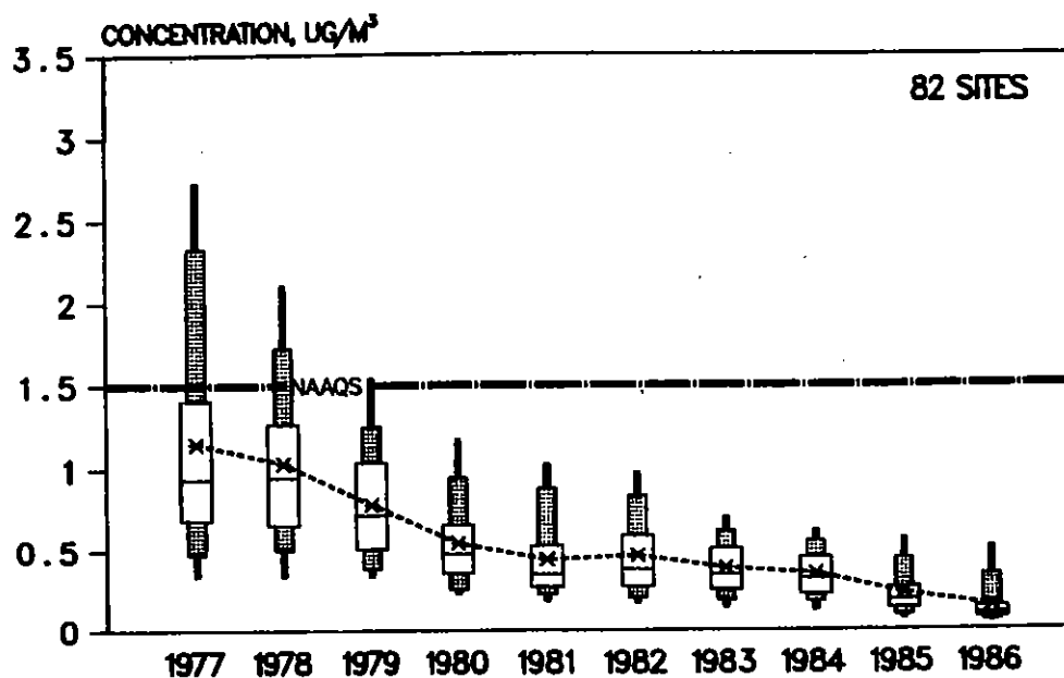
Figure 3-35. Boxplot comparisons of trends in maximum quarterly average lead concentrations at 82 sites, 1977-1986.
