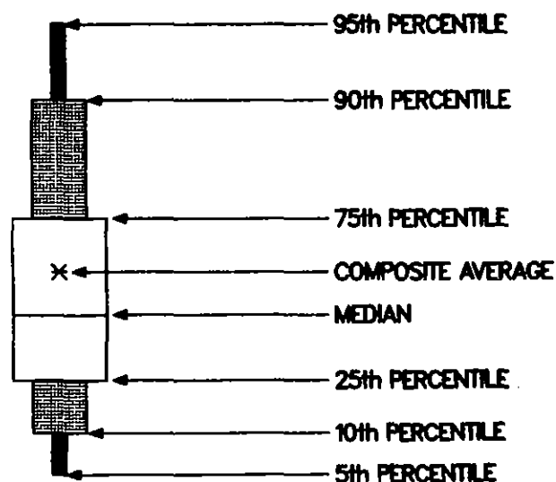
Figure 1-2. Illustrations of plotting conventions for boxplots.
