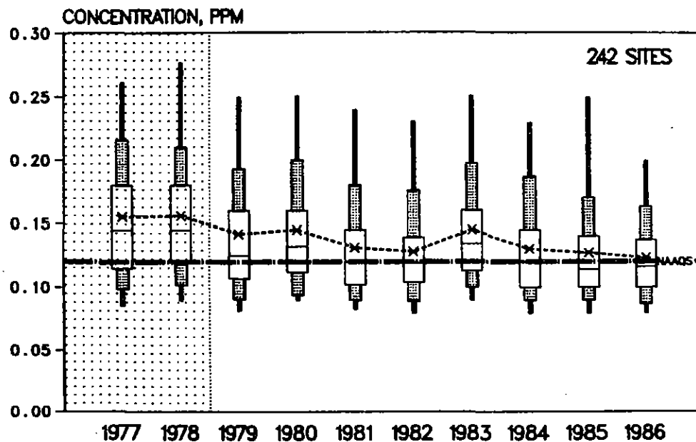
Figure 3-29. Boxplot comparisons of trends in annual second highest daily maximum 1-hour ozone concentration at 242 sites, 1977-1986.
