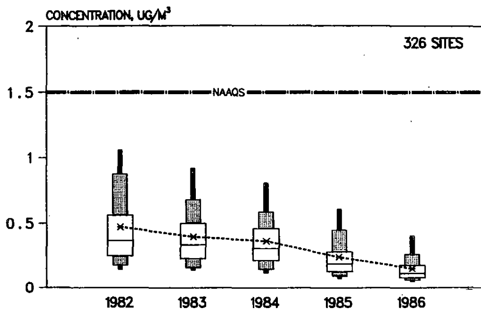
Figure 3-37. Boxplot comparisons of trends in maximum quarterly average lead concentrations at 326 sites, 1977-1986.
