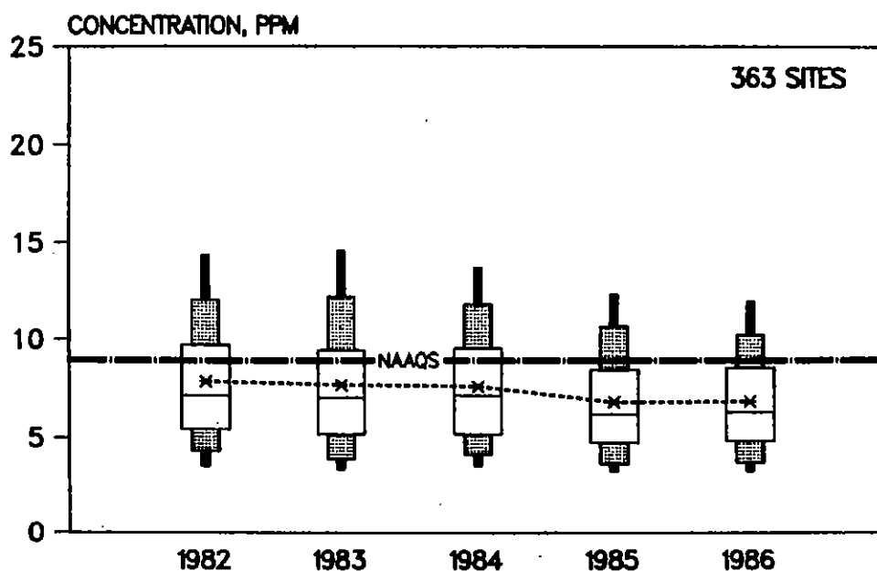
Figure 3-21. Boxplot comparisons of trends in second highest nonoverlapping 8-hour average carbon monoxide concentrations at 363 sites, 1982-1986.
