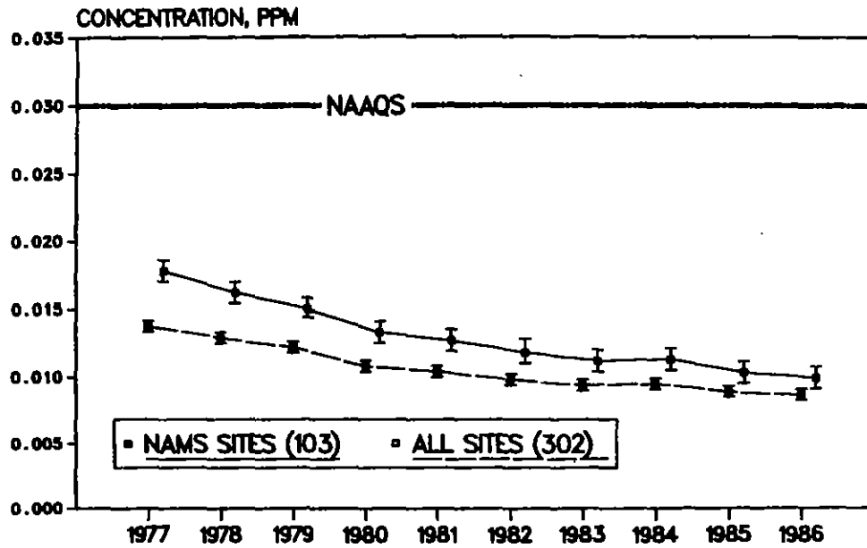
Figure 3-8. National trend in the composite average of the annual average sulfur dioxide concentration at both NAMS and all sites with 95 percent confidence intervals, 1977-1986.
