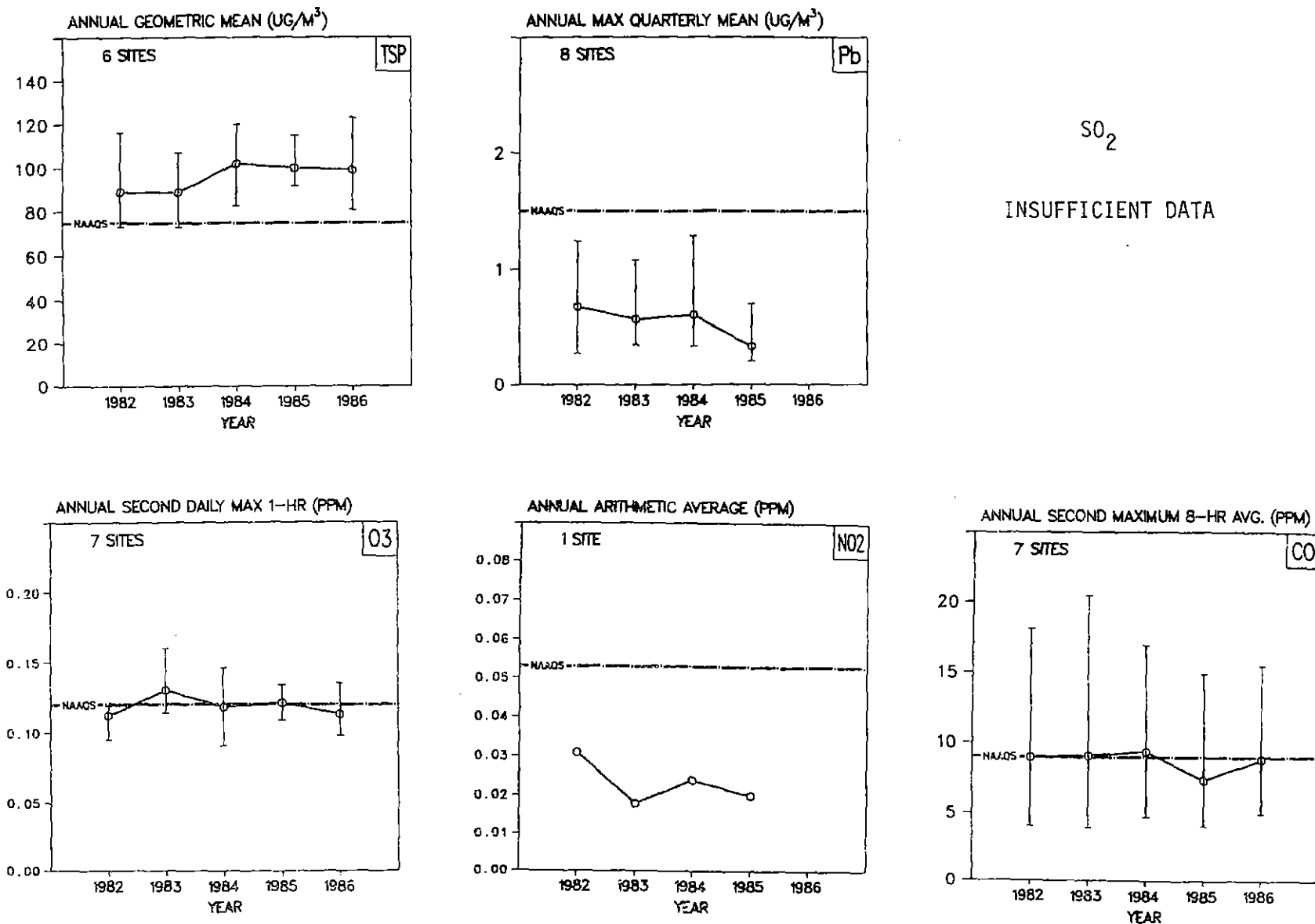
Figure 5-13. Air Quality Trends in the Composite Mean and Range of Pollutant-Specific Statistics for the Phoenix, AZ Urbanized Area, 1982-1986.
