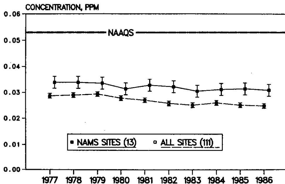
Figure 3-23. National trend in the composite average of nitrogen dioxide concentration at both NAMS and all sites with 95 percent confidence intervals, 1977-1986.
