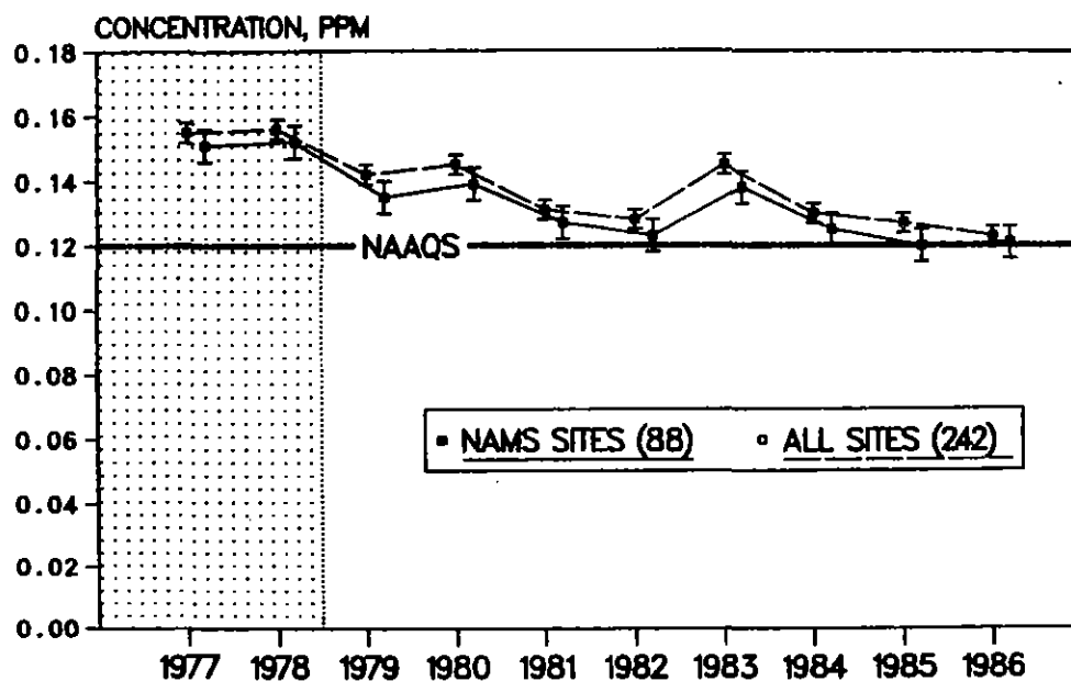
Figure 3-28. National trend in the composite average of the second highest maximum 1-hour ozone concentration at both NAMS and all sites with 95 percent confidence intervals, 1977-1986.
