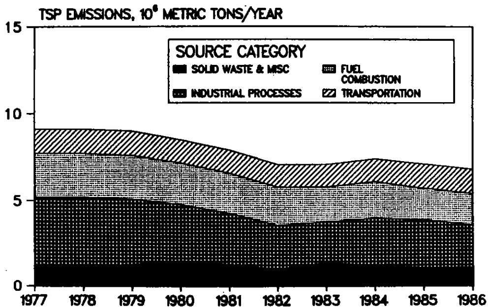
Figure 3-5. National trend in particulate emissions, 1977-1986.
