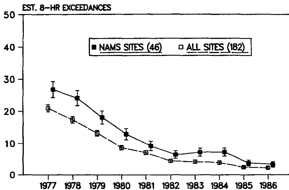
Figure 3-19. National trend in the composite average of the estimated number of exceedances of the 8-hour carbon monoxide NAAQS, at both NAMS and all sites with 95 percent confidence intervals, 1977-1986.
