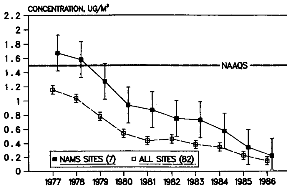
Figure 3-34. National trend in the composite average of the maximum quarterly average lead concentration at 82 sites and 7 NAMS sites with 95 percent confidence intervals, 1977-1986.
