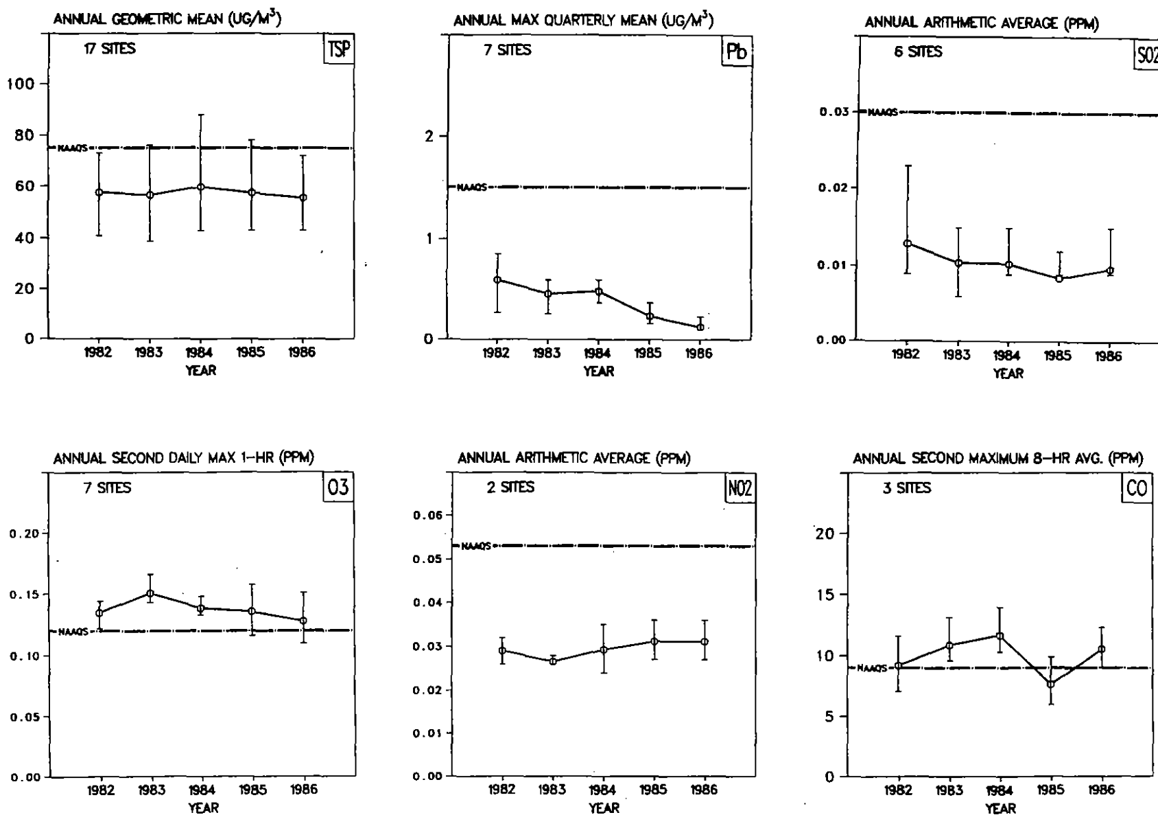
Figure 5-4. Air Quality Trends in the Composite Mean and Range of Pollutant-Specific Statistics for the Baltimore, MD Urbanized Area, 1982-1986.
