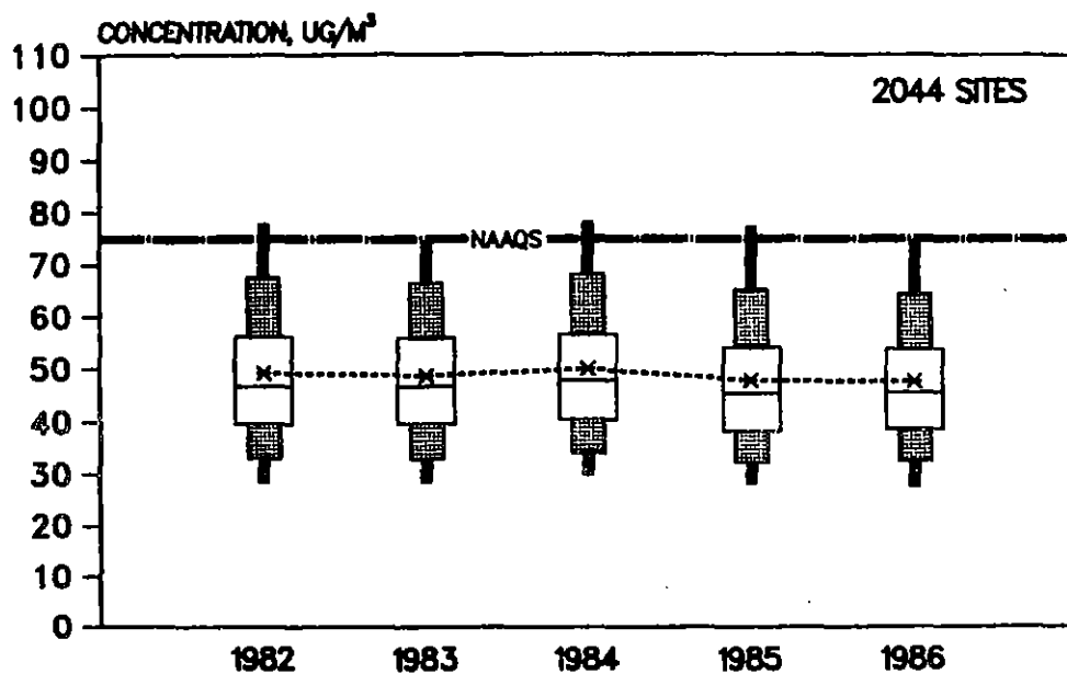
Figure 3-6. Boxplot comparisons of trends in annual mean total suspended particulate concentrations at 2044 sites, 1982-1986.
