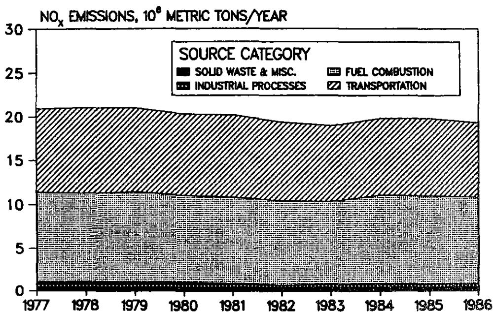
Figure 3-25. National trend in nitrogen oxides emissions, 1977-1986.
