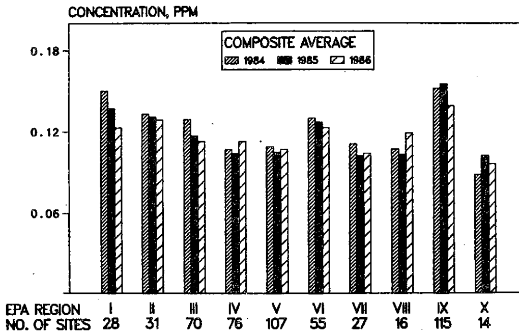
Figure 3-33. Regional comparison of the 1984, 1985, 1986 composite average of the second-highest daily 1-hour ozone concentrations.
