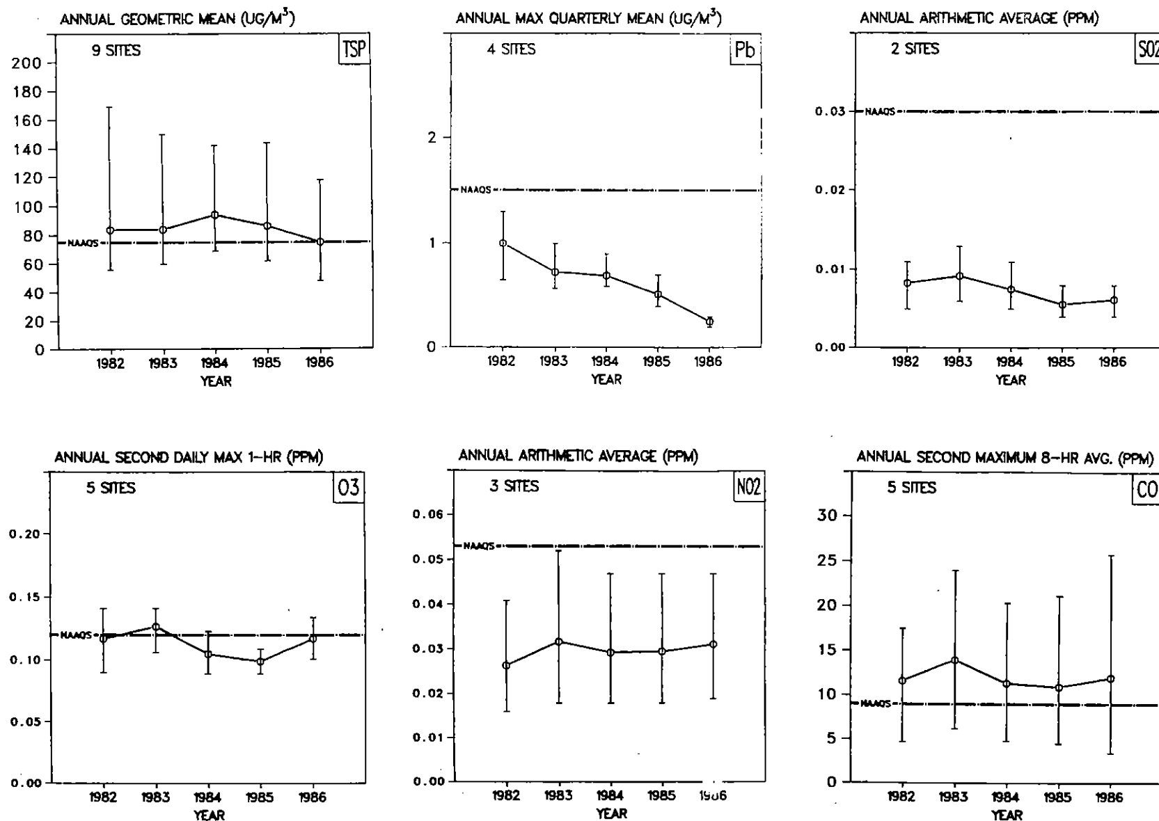
Figure 5-11. Air Quality Trends in the Composite Mean and Range of Pollutant-Specific Statistics for the Denver, CO Urbanized Area, 1982-1986.
