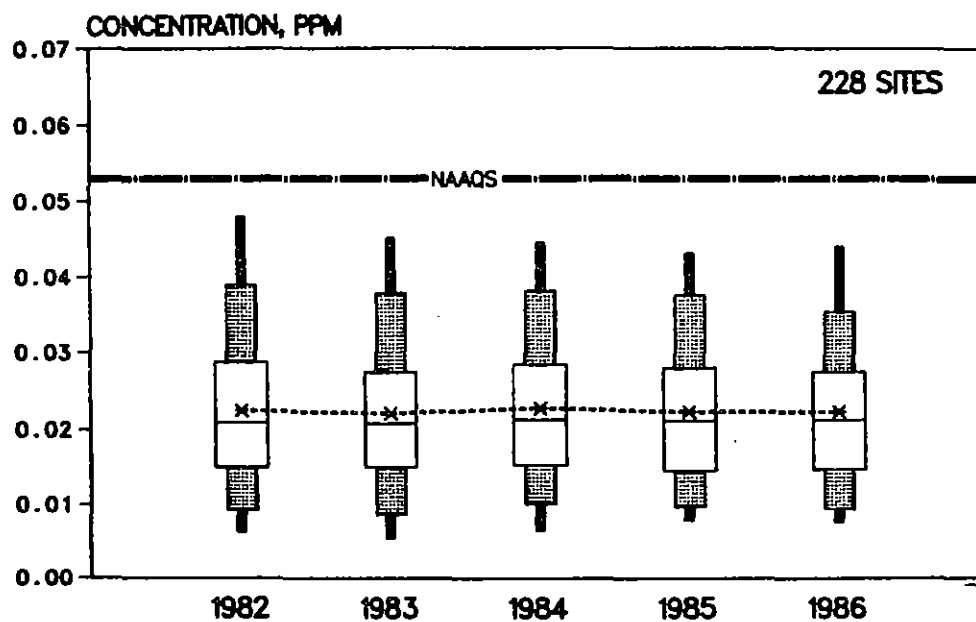
Figure 3-26. Boxplot comparisons of trends in annual mean nitrogen dioxide concentrations at 228 sites, 1982-1986.
