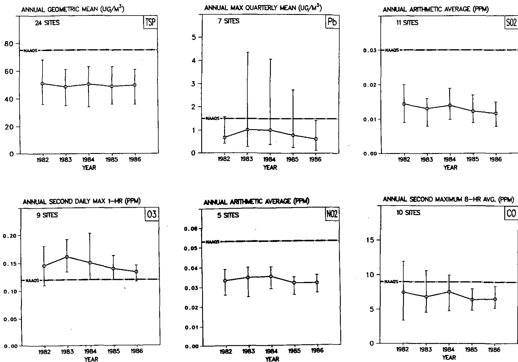
Figure 5-5. Air Quality Trends in the Composite Mean and Range of Pollutant-Specific Statistics for the Philadelphia, PA-NJ Urbanized Area, 1982-1986.
