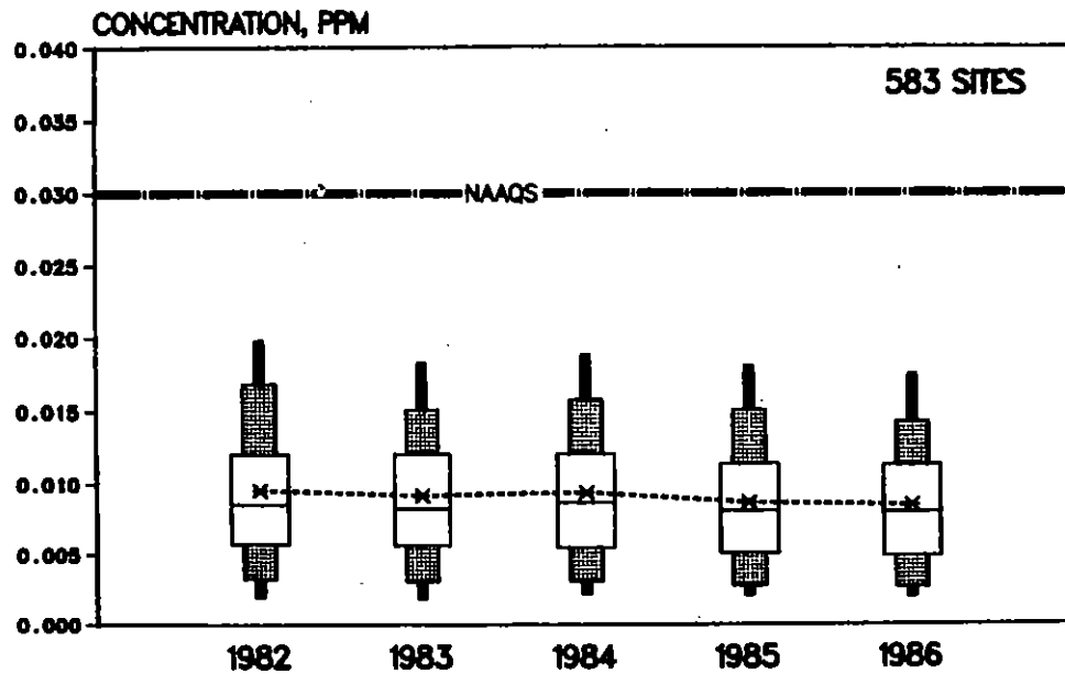
Figure 3-14. Boxplot comparisons of trends in annual mean sulfur dioxide concentrations at 583 sites, 1982-1986.
