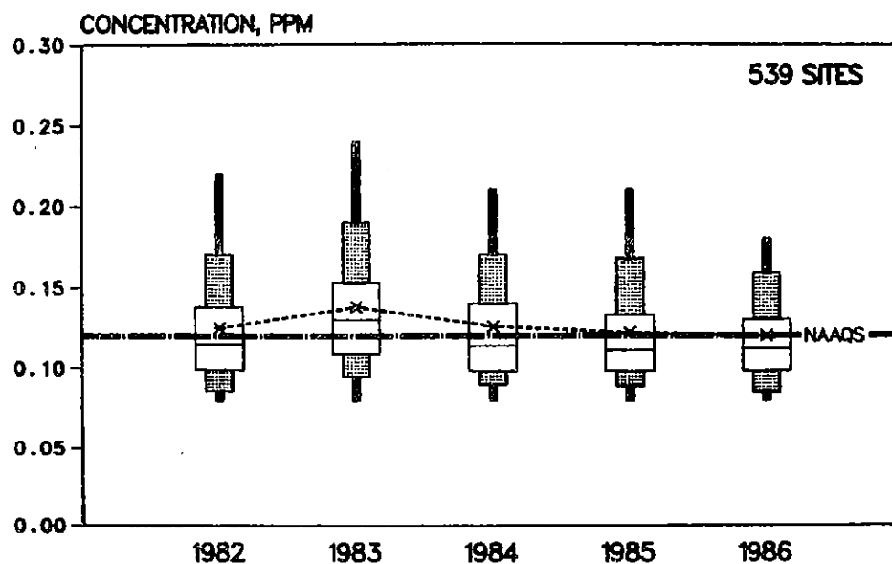
Figure 3-32. Boxplot comparisons of trends in annual second highest daily maximum 1-hour ozone concentrations at 539 sites, 1982-1986.
