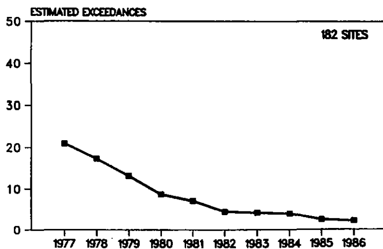
Figure 1-12. National trend in the composite average of the estimated number of exceedances of the 8-hour CO NAAQS, 1977 - 1986.
