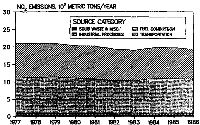
Figure 1-16. National trend in emissions of nitrogen oxides, 1977 - 1986.
