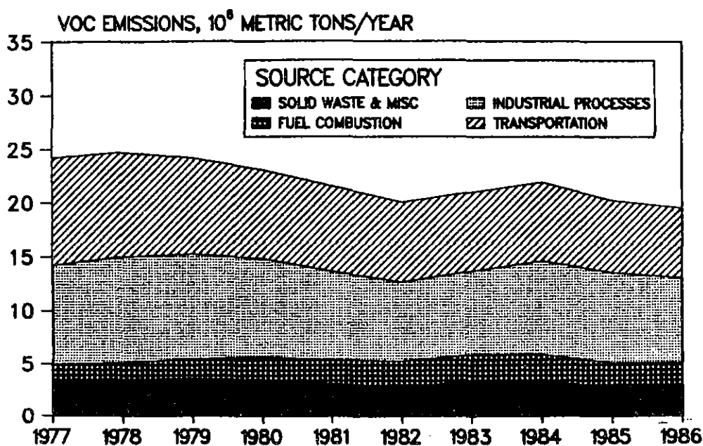
Figure 3-31. National trend in emissions of volatile organic compounds, 1977-1986.
