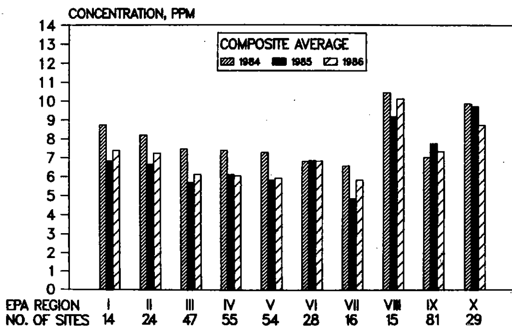
Figure 3-22. Regional comparison of the 1984, 1985, 1986 composite average of the second highest nonoverlapping 8-hour average carbon monoxide concentration.
