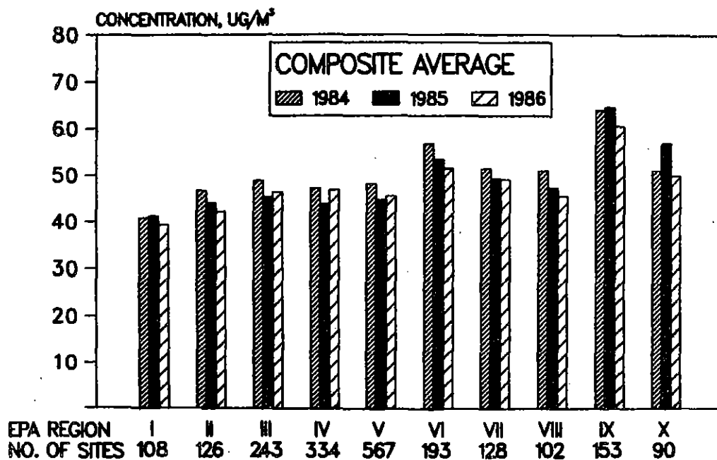
Figure 3-7. Regional comparison of the 1984, 1985, 1986 composite average of the geometric mean total suspended particulate concentration.
