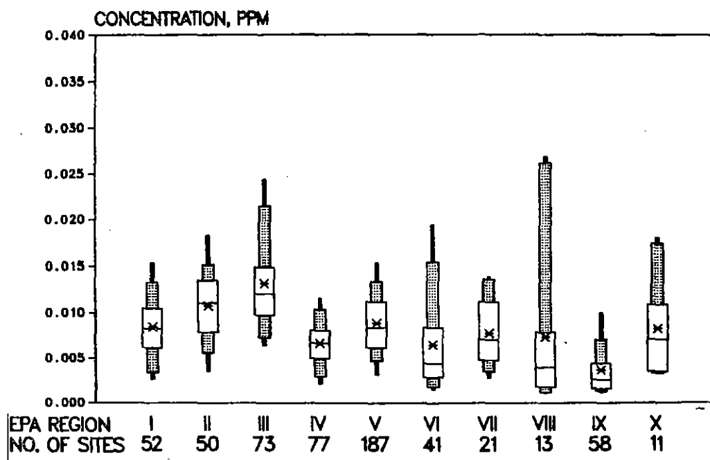
Figure 3-16. Regional boxplot comparisons of the annual average sulfur dioxide concentrations in 1986.
