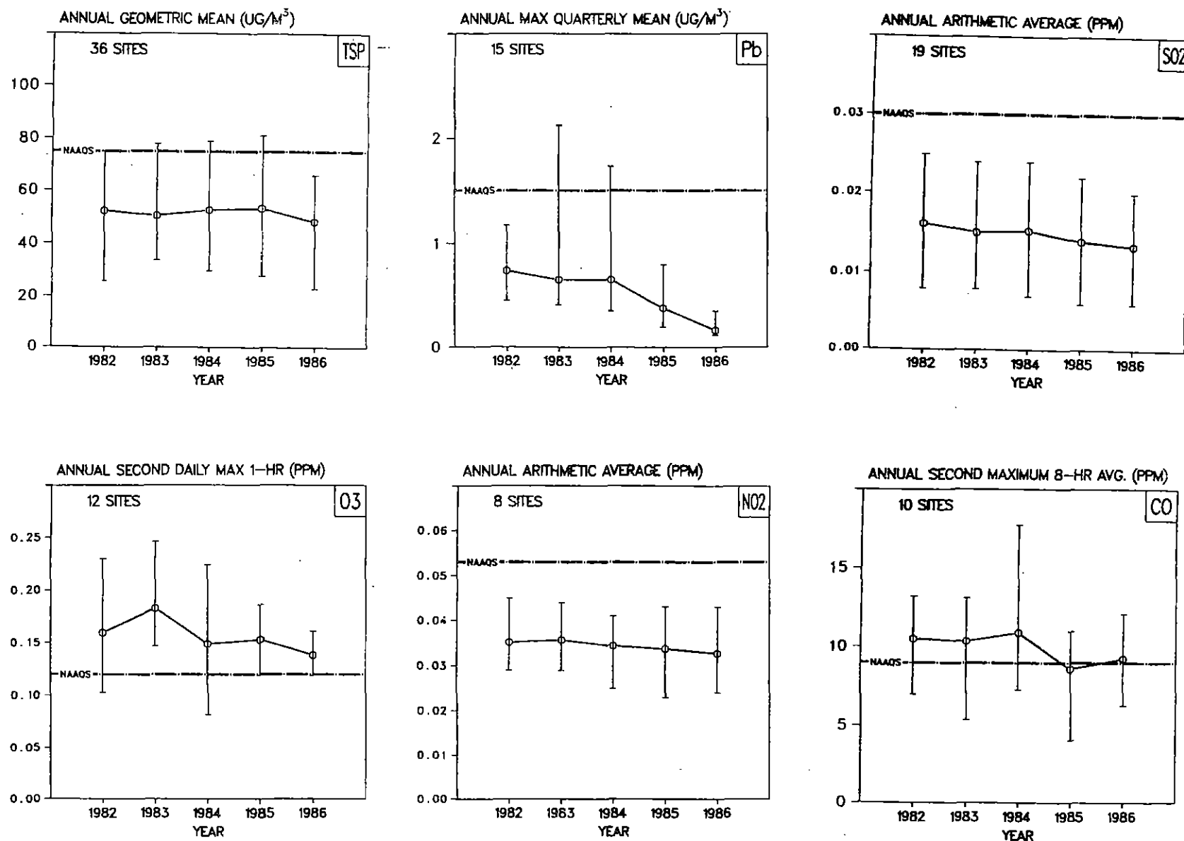
Figure 5-3. Air Quality Trends in the Composite Mean and Range of Pollutant-Specific Statistics for the New York, NY-NJ Urbanized Area, 1982-1986.
