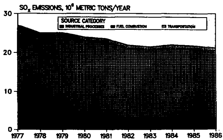
Figure 1-9. National trend in sulfur oxide emissions, 1977 - 1986.
