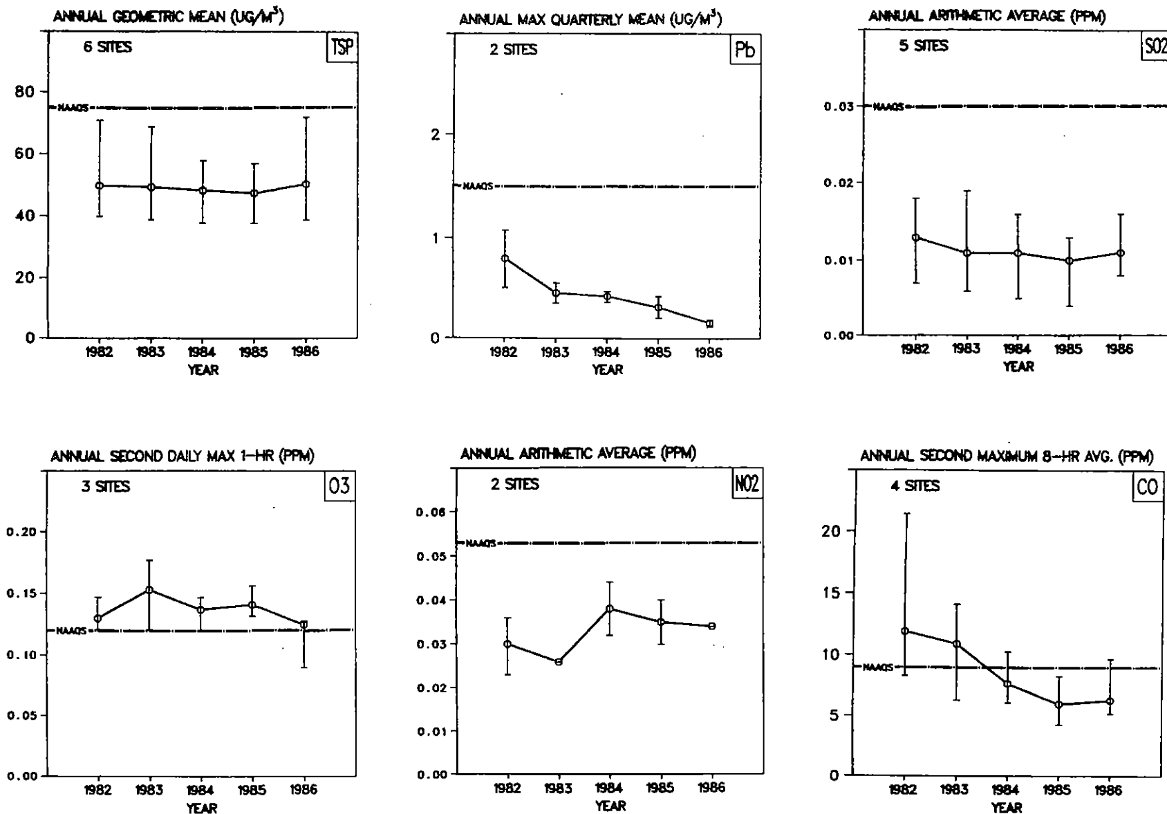
Figure 5-2. Air Quality Trends in the Composite Mean and Range of Pollutant-Specific Statistics for the Boston, MA Urbanized Area, 1982-1986.
