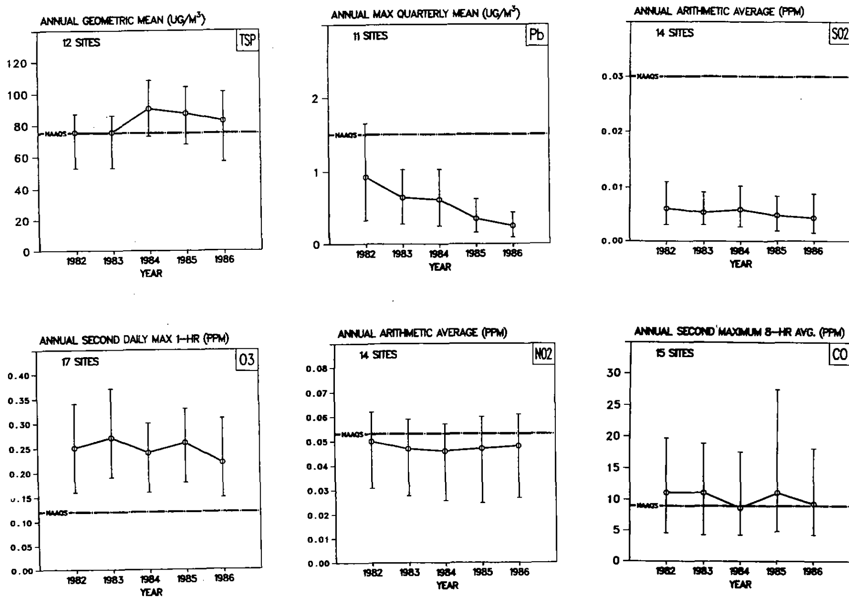
Figure 5-12. Air Quality Trends in the Composite Mean and Range of Pollutant-Specific Statistics for the Los Angeles - Long Beach, CA Urbanized Area, 1982-1986.
