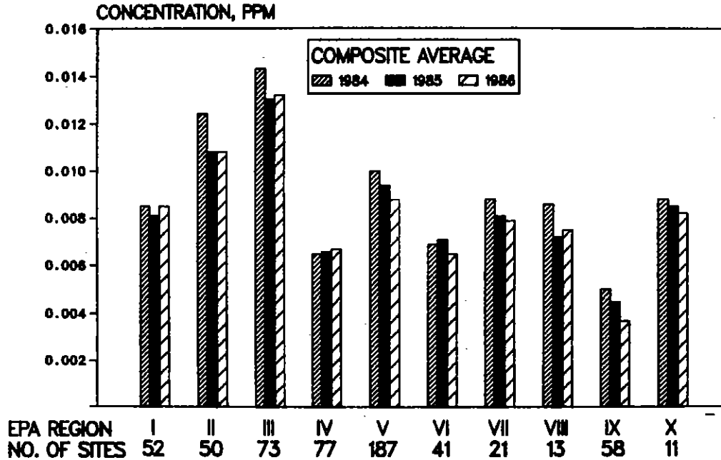
Figure 3-15. Regional comparison of the 1984, 1985, 1986 composite average of the annual average sulfur dioxide concentration.
