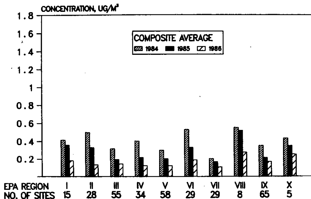
Figure 3-38. Regional comparison of the 1984, 1985, 1986 composite average of the maximum quarterly average lead concentration.
