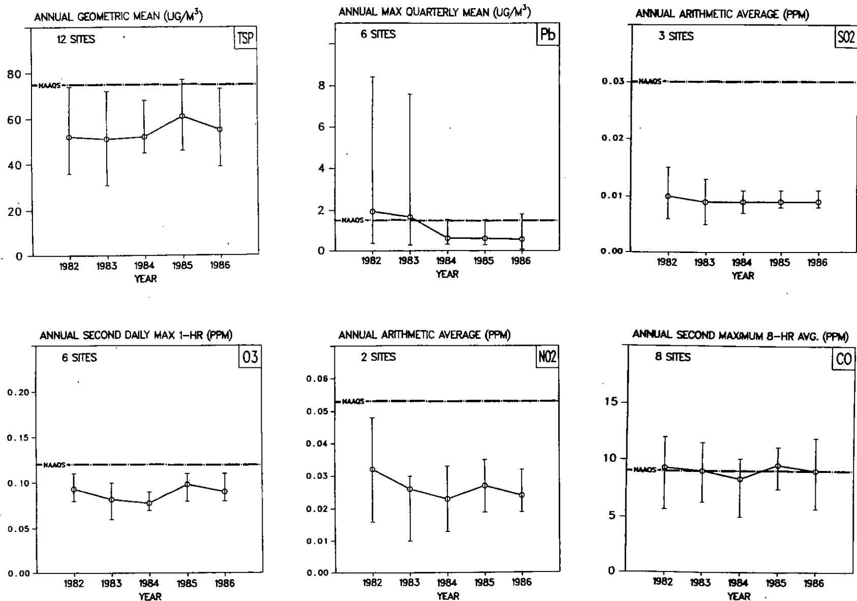
Figure 5-15. Air Quality Trends in the Composite Mean and Range of Pollutant-Specific Statistics for the Seattle, WA Urbanized Area, 1982-1986.
