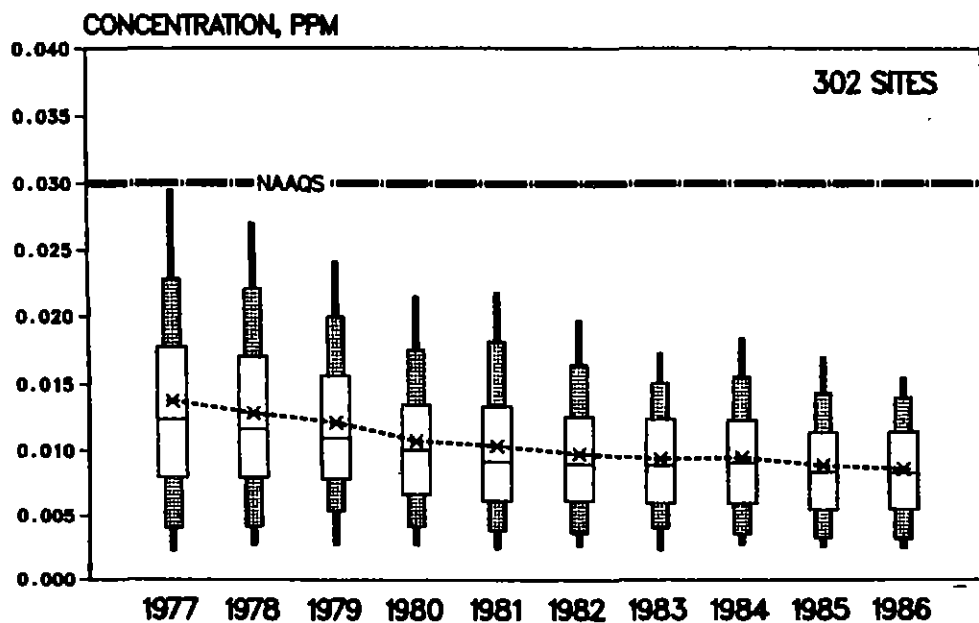
Figure 3-11. Boxplot comparisons of trends in annual mean sulfur dioxide concentrations at 302 sites, 1977-1986.
