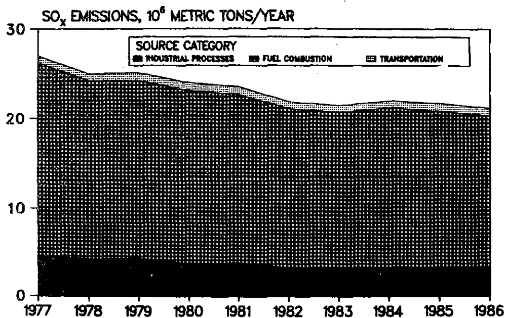
Figure 3-13. National trend in sulfur oxide emissions, 1977-1986.
