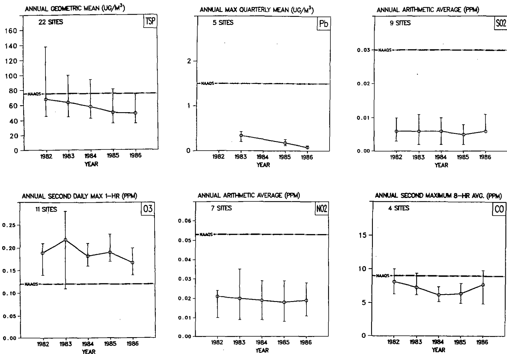
Figure 5-9. Air Quality Trends in the Composite Mean and Range of Pollutant-Specific Statistics for the Houston, TX Urbanized Area, 1982-1986.
