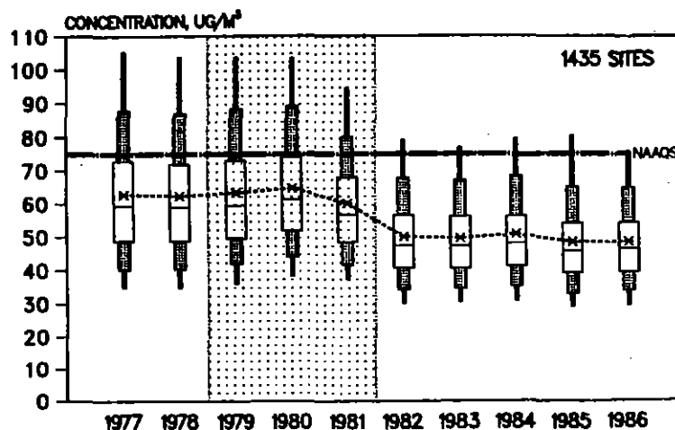
Figure 1-3. National boxplot trend in annual geometric mean TSP concentrations, 1977 - 1986.
