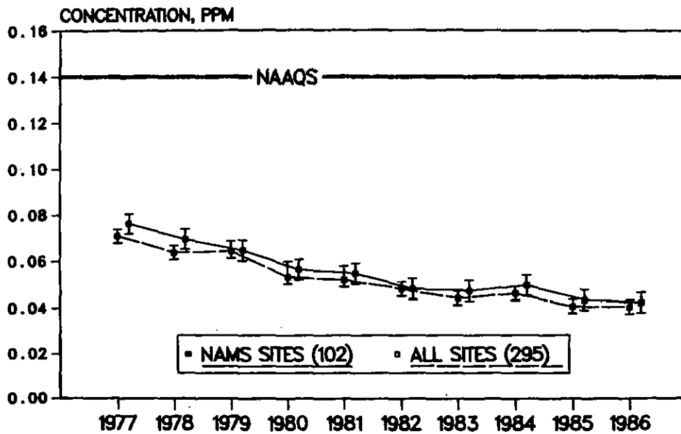
Figure 3-9. National trend in the composite average of the second-highest 24-hour sulfur dioxide concentration at both NAMS and all sites with 95 percent confidence intervals, 1977-1986.
