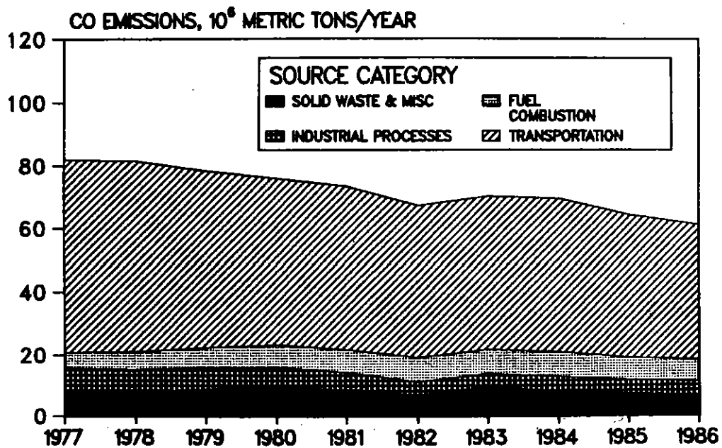
Figure 3-20. National trend in emissions of carbon monoxide, 1977-1986.
