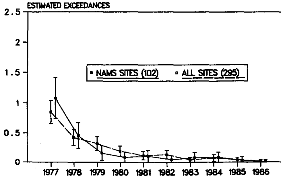
Figure 3-10. National trend in the composite average of the estimated number of exceedances of the 24-hour sulfur dioxide NAAQS at both NAMS and all sites with confidence intervals, 1977-1986.
