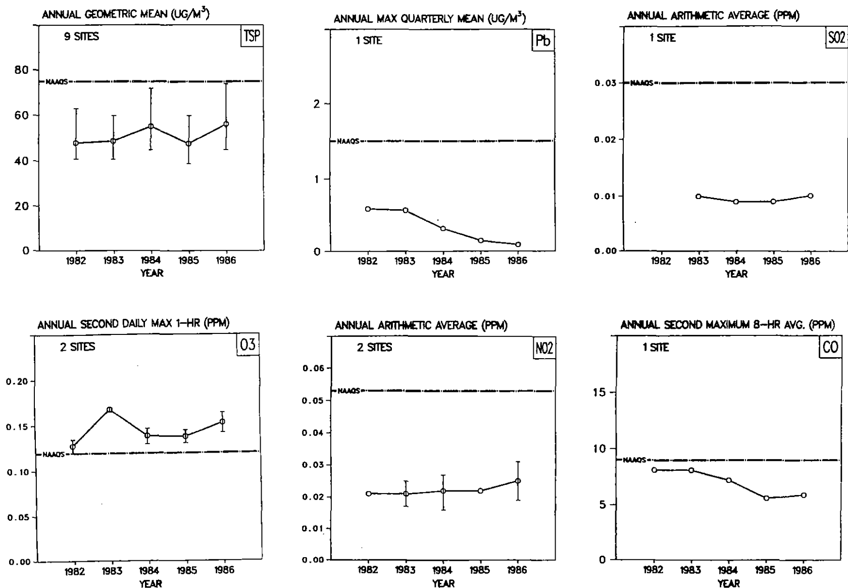
Figure 5-6. Air Quality Trends in the Composite Mean and Range of Pollutant-Specific Statistics for the Atlanta, GA Urbanized Area, 1982-1986.
