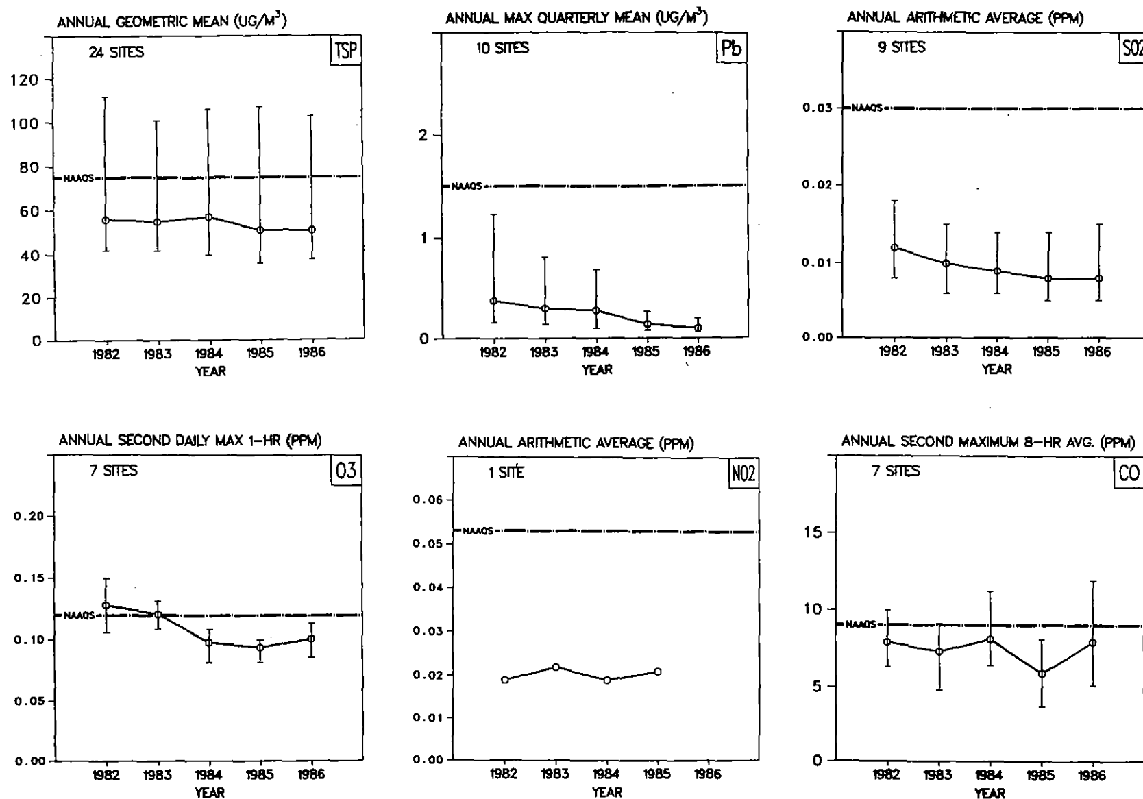
Figure 5-8. Air Quality Trends in the Composite Mean and Range of Pollutant-Specific Statistics for the Detroit, MI Urbanized Area, 1982-1986.
