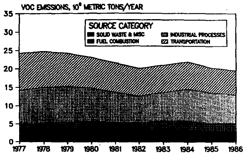
Figure 1-19. National trend in emissions of volatile organic compounds, 1977 - 1986.
