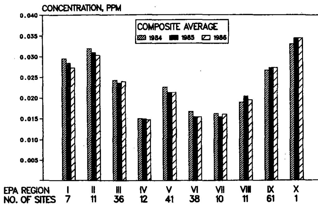
Figure 3-27. Regional comparison of 1984, 1985, 1986 composite average of the annual mean nitrogen dioxide concentration.
