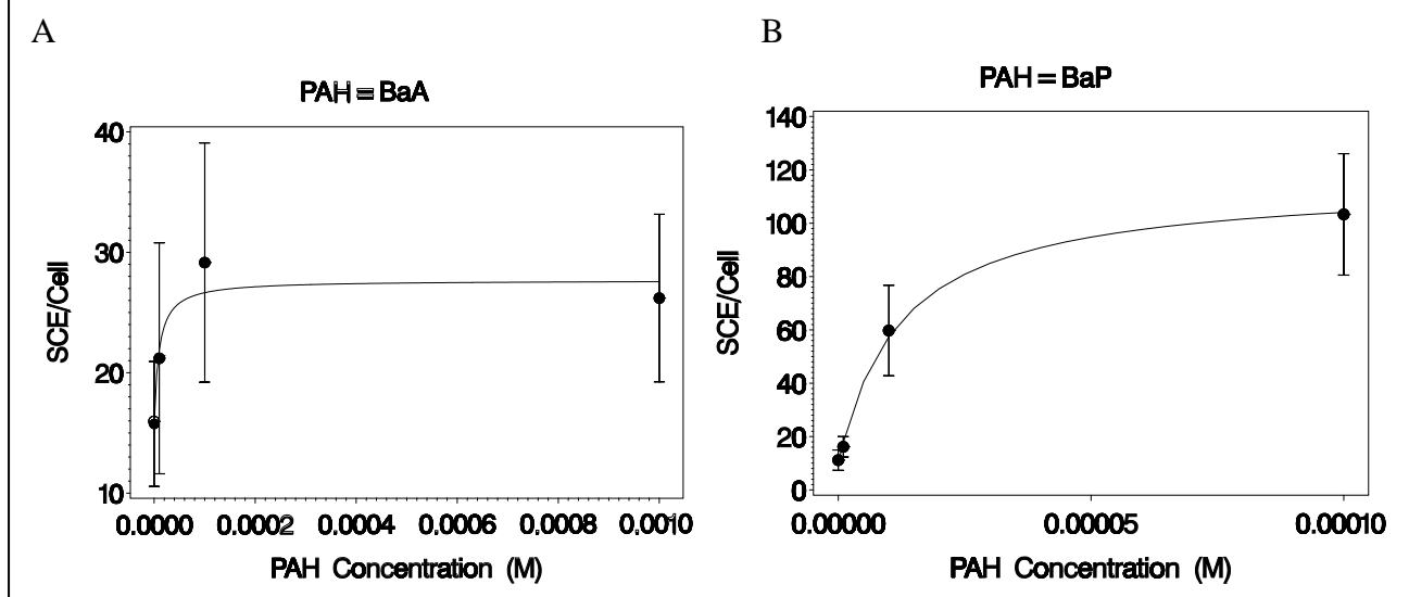
Figure 1: Observed sample means and predicted response from a Hill model. Sample means are denoted with dots and +/- one standard deviation from each mean is denoted by the error bars.
