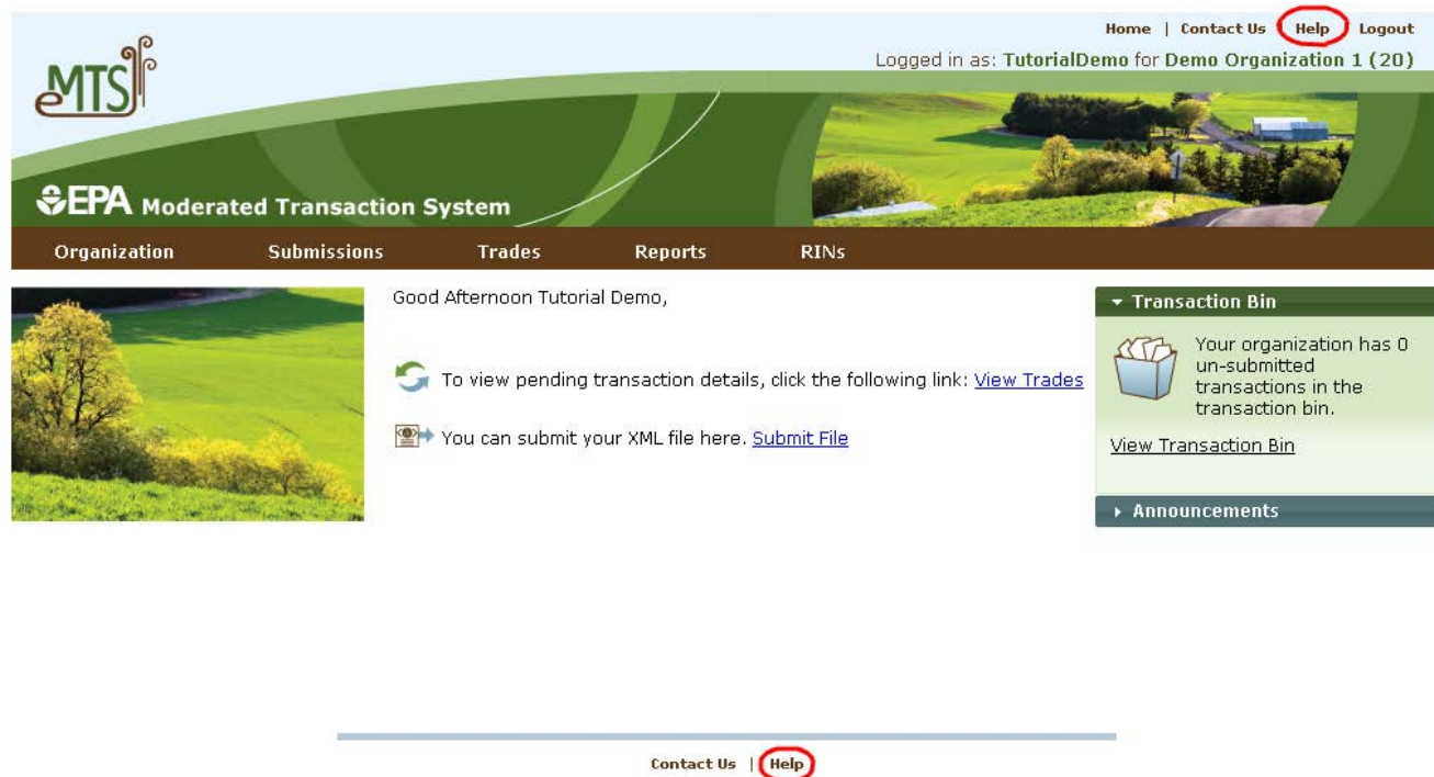
Figure 5-34: Help Page
