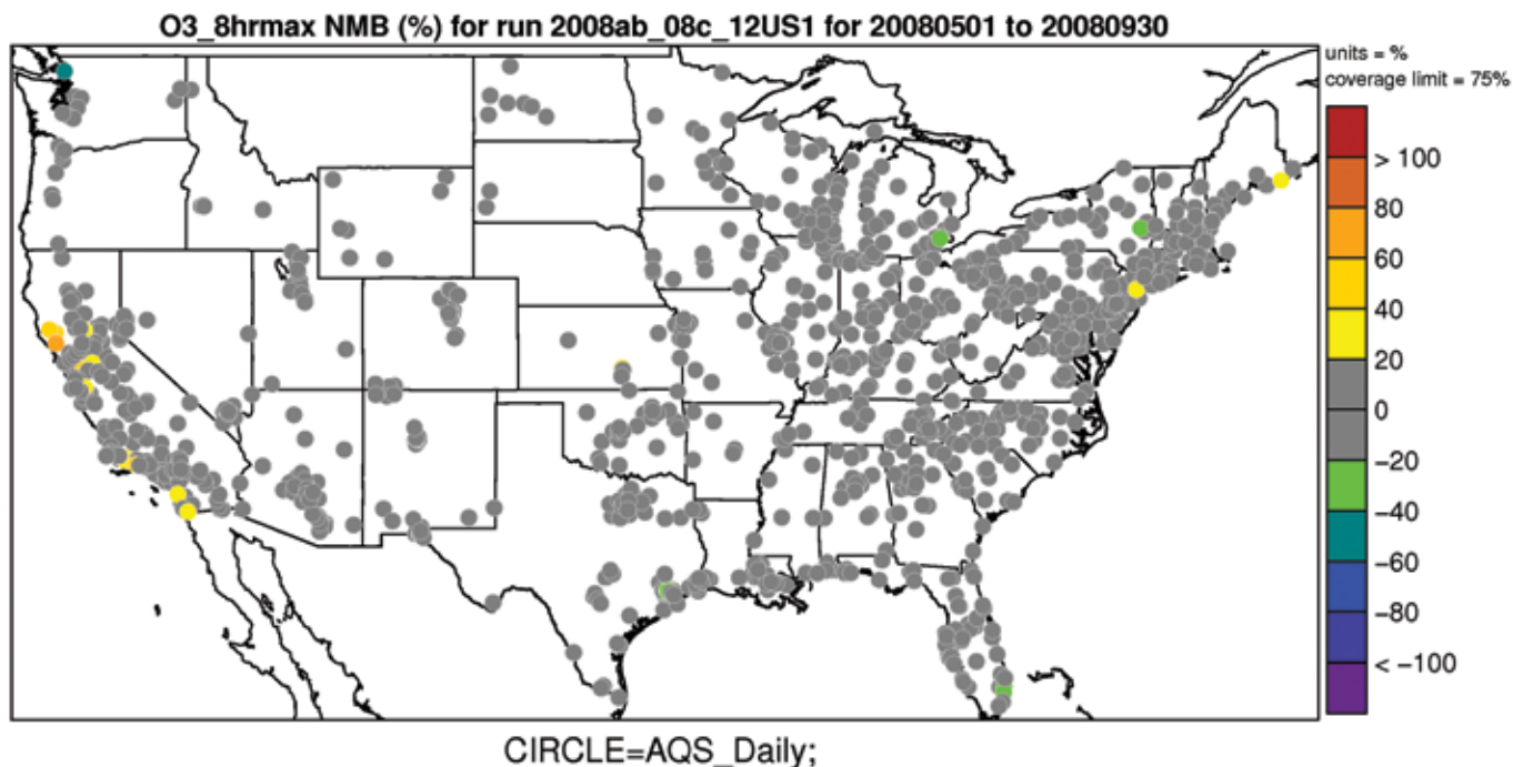
Figure 4-2. Normalized Mean Bias (%) of 8-hour daily maximum ozone greater than 60 ppb over the period May-September 2008 at monitoring sites in the continental U.S. modeling domain.
