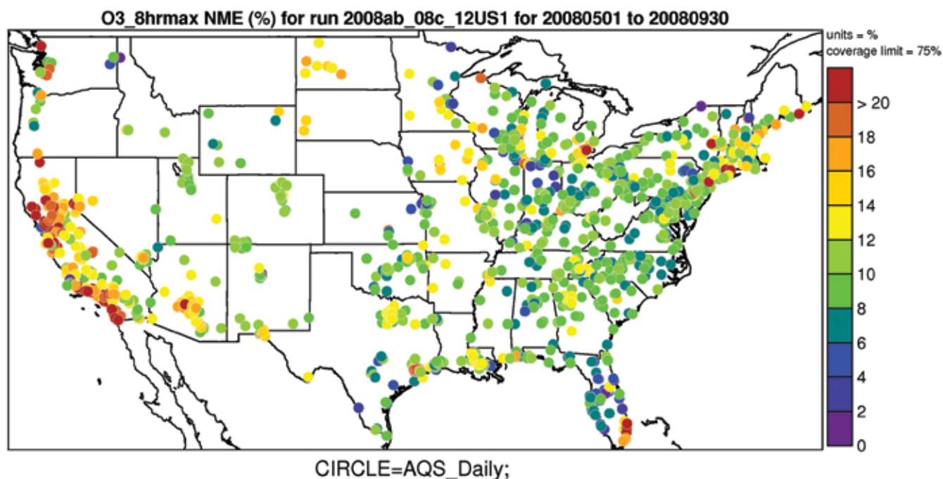
Figure 4-3. Normalized Mean Error (%) of 8-hour daily maximum ozone greater than 60 ppb over the period May-September 2008 at monitoring sites in the continental U.S. modeling domain.
