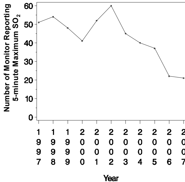
Figure 7-21. Temporal trends in the number of ambient monitors in operation per year for monitors reporting both 5-minute and 1-hour SO 2 concentrations
