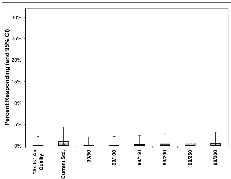
Figure 4-4. Percent of Asthmatic Children Engaged in Moderate or Greater Exertion Exhibiting Lung Function Response (Defined as a Decrease in FEV_1 \geq 15\% ) Attributable to SO_2 Within Given Ranges Under Different Air Quality Scenarios*
