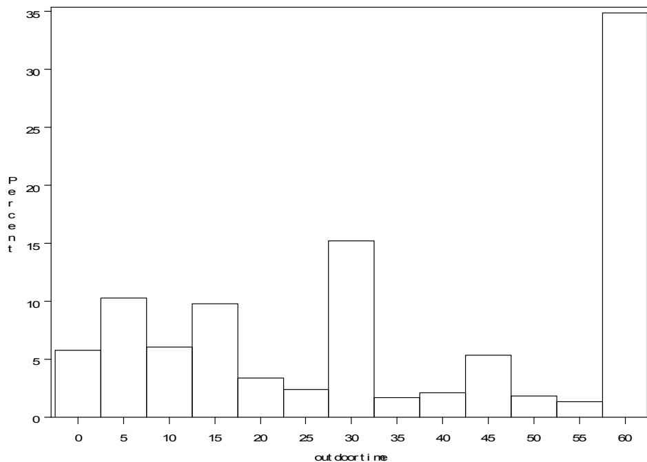
Figure 8-23. Duration of time spent outdoors (in minutes) using all CHAD events
