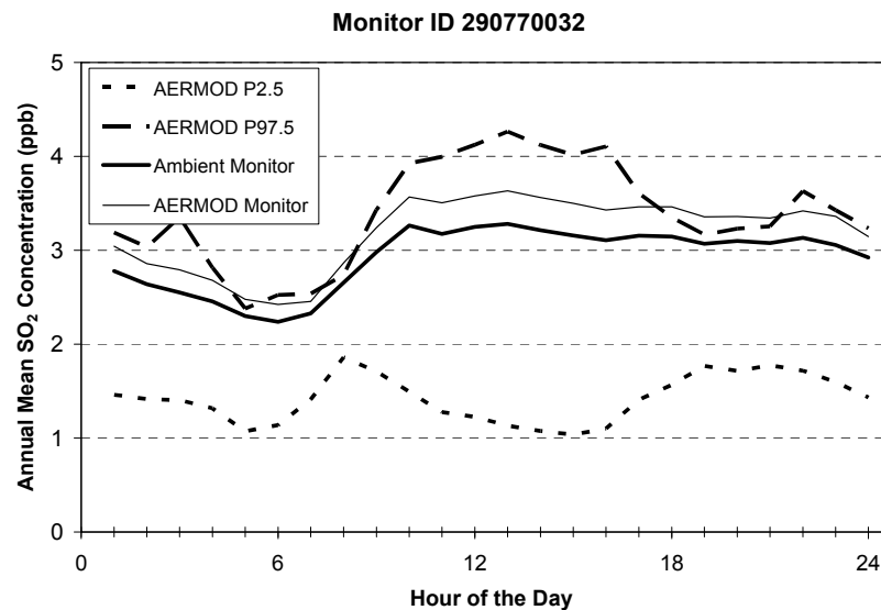
Figure 8-6. Comparison of measured ambient monitor SO 2 concentration distribution and diurnal profile with the modeled monitor receptor and receptors within 4 km of monitors 290770026 and 290770032 in Greene County, Mo.
