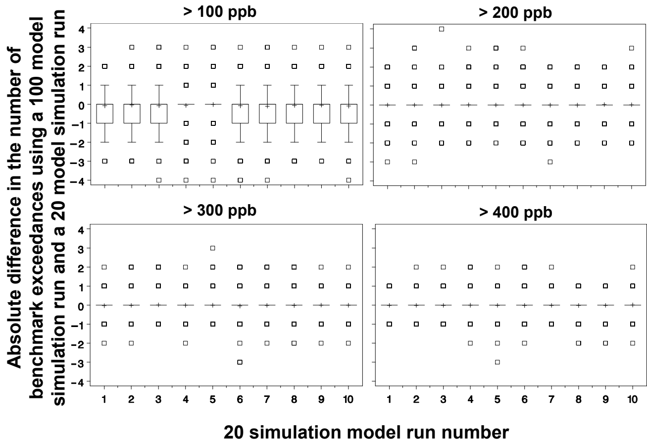
Figure 7-28. Distributions of the calculated difference between estimated concentration exceedances using a single 100 model simulation run and those estimated using ten independent 20 model simulation runs. Box represents the inner quartile range (IQR, or the 25 th to 75 th percentile), + indicates the mean, whiskers are 1.5 times the IQR.
