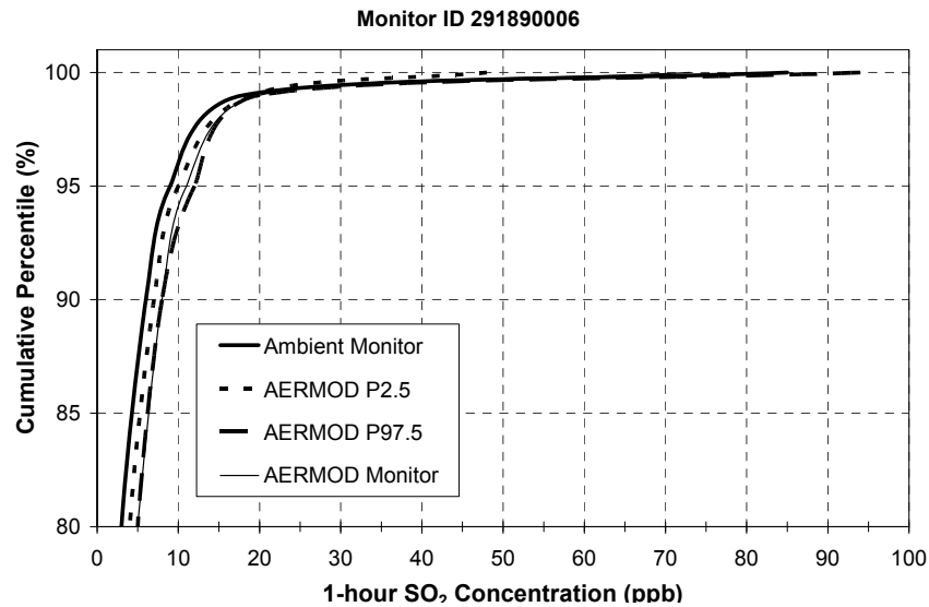
Figure 8-9. Comparison of measured ambient monitor SO 2 concentration distribution and diurnal profile with the modeled monitor receptor and receptors within 4 km of monitors 291890004 and 291890006 in St Louis, Mo.
