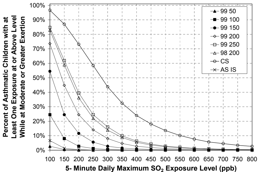
Figure 8-17. Percent of all asthmatics (top) and asthmatic children (bottom) with 5-minute daily maximum SO 2 exposures above selected exposure levels in St. Louis, year 2002 air quality as is and adjusted to just meeting the current and potential alternative standards.
