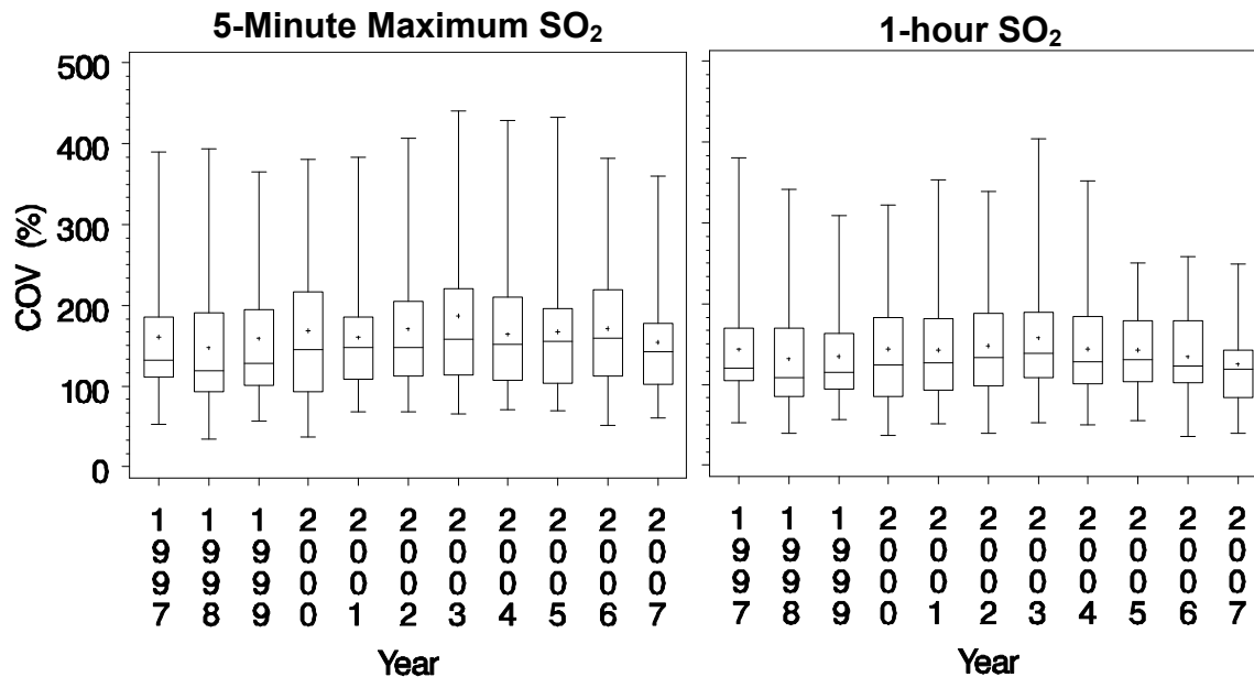
Figure 7-22. Temporal trends in the coefficient of variability (COV) for 5-minute maximum and 1-hour concentrations at the 98 monitors that reported both 5-minute and 1-hour SO 2 concentrations
