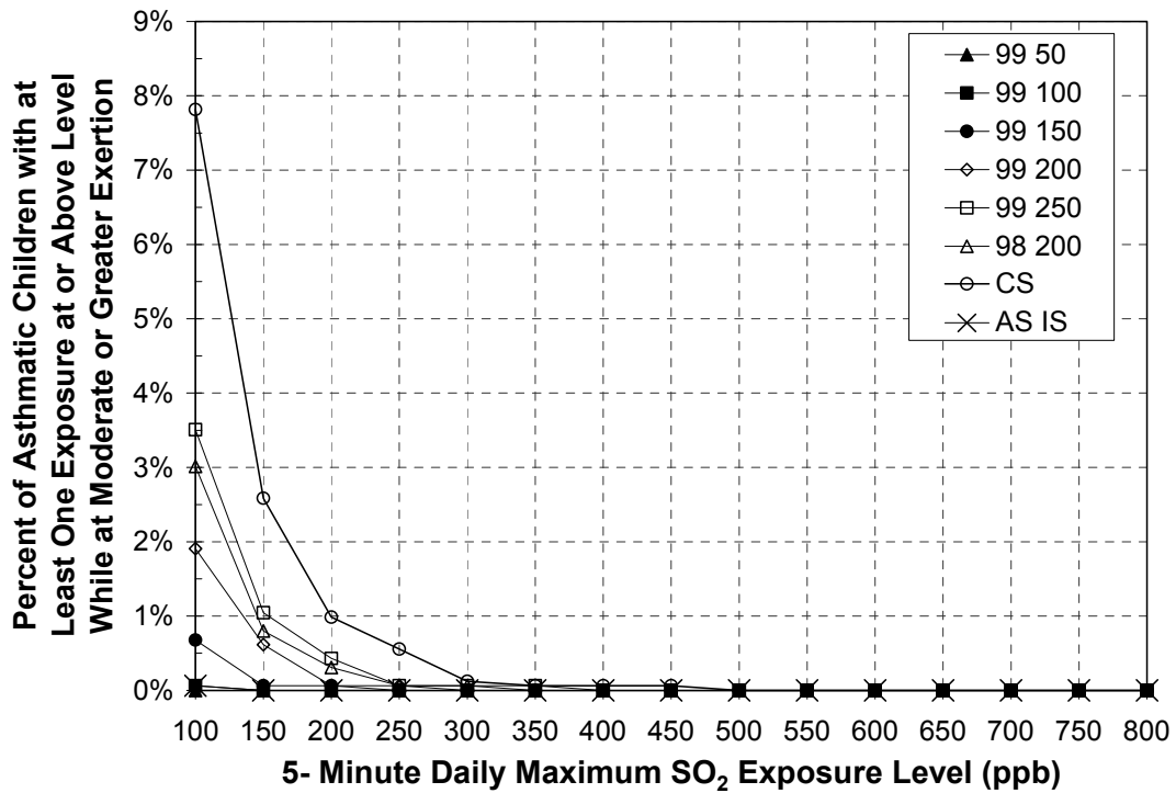
Figure 8-14. Percent of all asthmatics (top) and asthmatic children (bottom) with 5-minute daily maximum SO 2 exposures above selected exposure levels in Greene County, year 2002 air quality as is and adjusted to just meeting the current and potential alternative standards.
