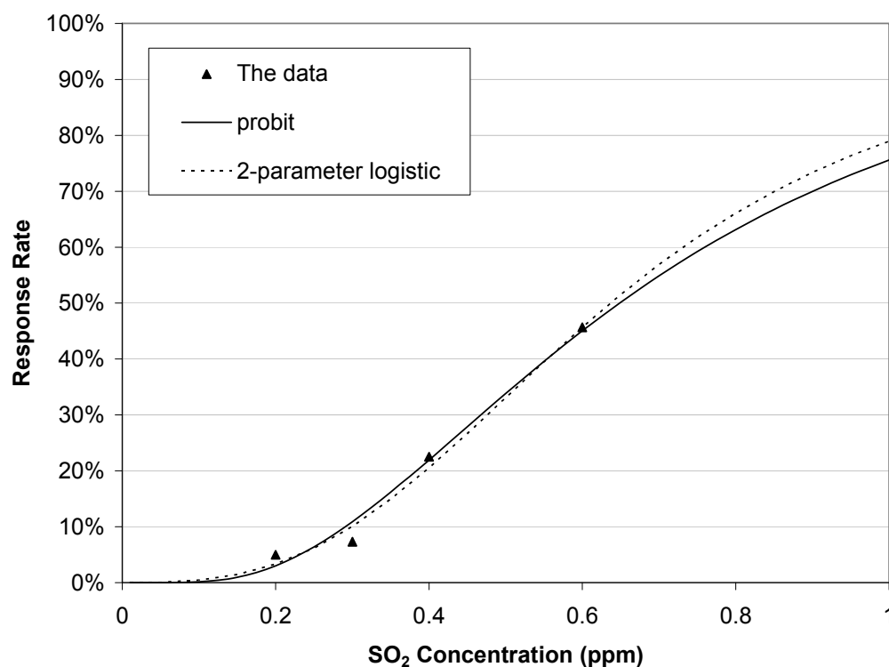
Figure 9-5. Bayesian-Estimated Median Exposure-Response Functions: Decrease in FEV1 > 20% for 5-Minute Exposures of Asthmatics Under Moderate or Greater Exertion*
