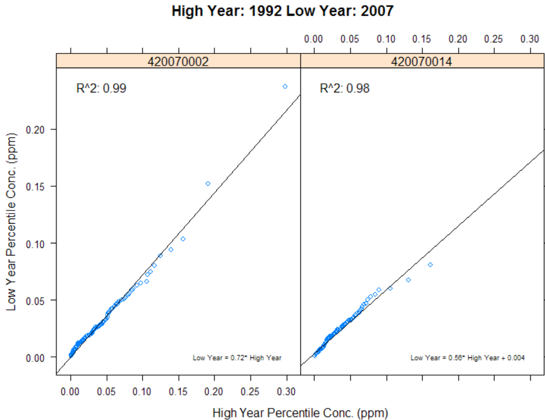
Figure 6-3. Comparison of measured daily maximum SO 2 concentration percentiles in Beaver County, PA for a high concentration year (1992) versus a low concentration year (2007) at two ambient monitors.
