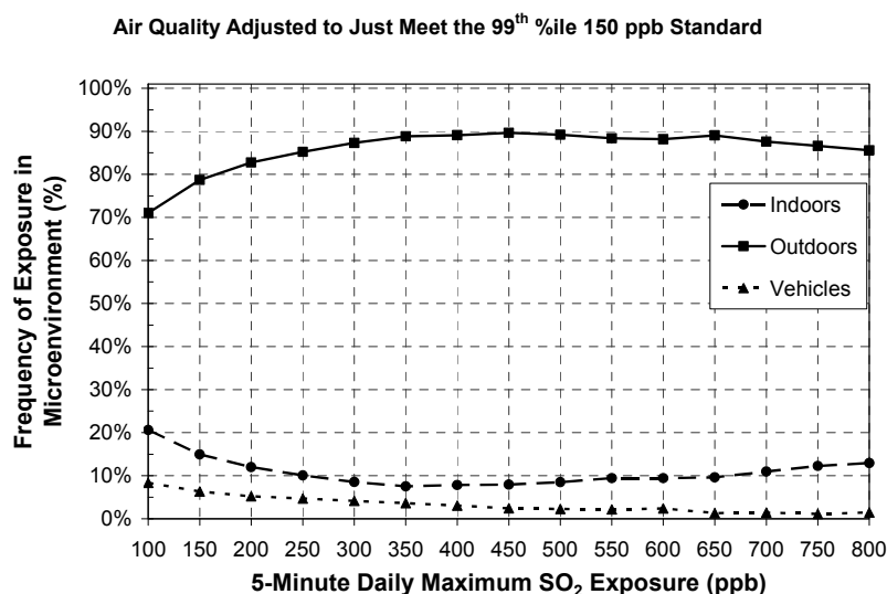
Figure 8-19. The frequency of estimated exposure level exceedances in indoor, outdoor, and vehicle microenvironments given as is air quality (top), air quality adjusted to just meeting the current standard (middle) and that adjusted to just meeting a 99 th percentile 1-hour daily maximum standard level of 150 ppb (bottom) in St. Louis.
