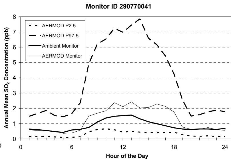
Figure 8-7. Comparison of measured ambient monitor SO 2 concentration distribution and diurnal profile with the modeled monitor receptor and receptors within 4 km of monitors 290770040 and 290770041 in Greene County, Mo.
