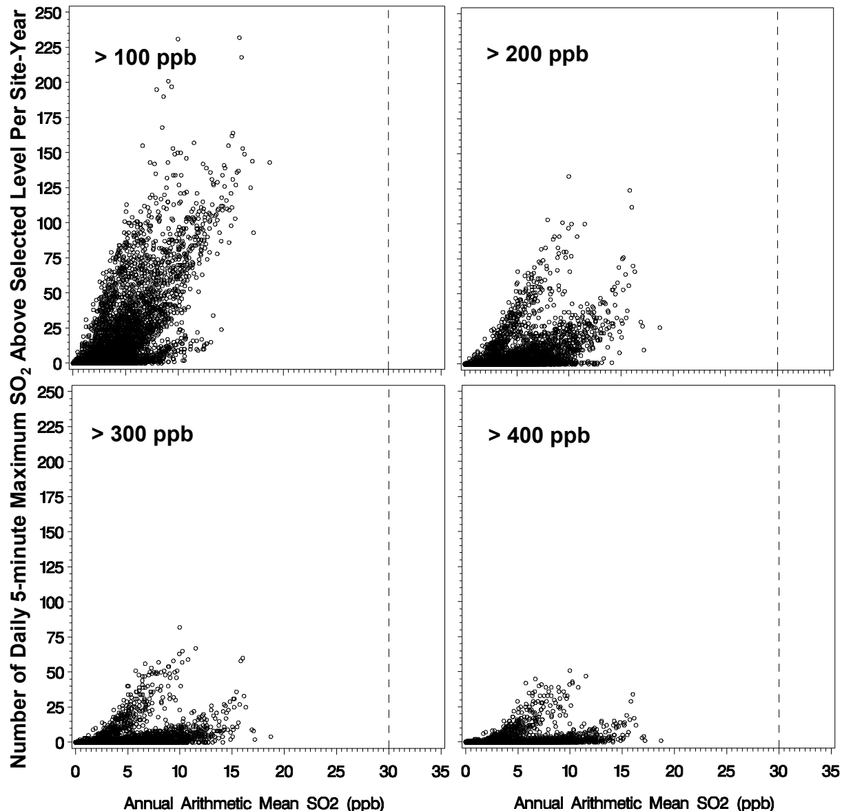
Figure 7-13. The number of modeled daily 5-minute maximum SO 2 concentrations above potential health effect benchmark levels per year at 809 ambient monitors given the annual average SO 2 concentration, 1997-2006 air quality as is. The level of the annual average SO 2 NAAQS of 30 ppb is indicated by the dashed line.
