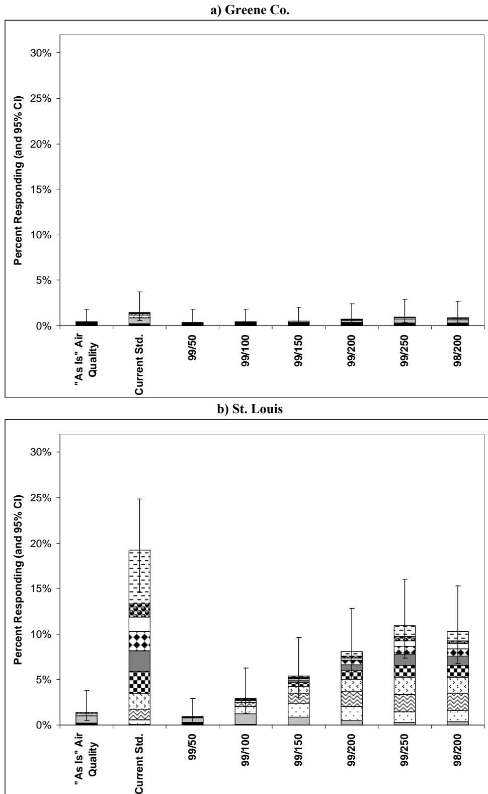
Figure 4-2. Percent of Asthmatic Children Engaged in Moderate or Greater Exertion Exhibiting Lung Function Response (Defined as an Increase in sRaw \geq 100%) Attributable to SO 2 Within Given Ranges Under Different Air Quality Scenarios*
