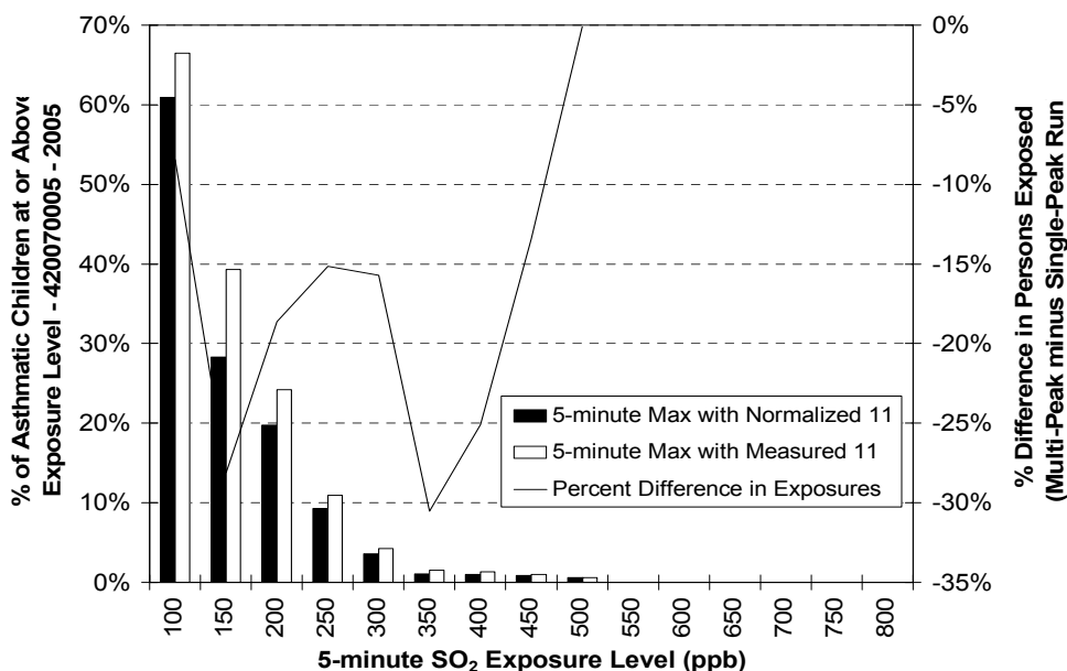
Figure 8-25. Percent of asthmatic children above given exposure level for two APEX simulations: one using multiple peak concentrations in an hour, the other assuming a single peak concentration. Continuous 5-minute monitoring data (ID 42007005, year 2005) were used as the air quality input.
