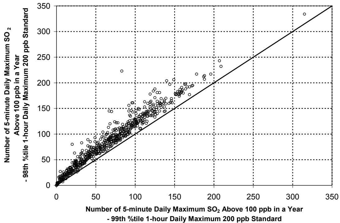
4 Figure 7-18. The number of modeled daily 5-minute maximum SO 2 concentrations 5 above 100 ppb per year given the 99 th and 98 th percentile forms at a 1-hour daily 6 maximum level of 200 ppb, using the 40-county air quality data set.
