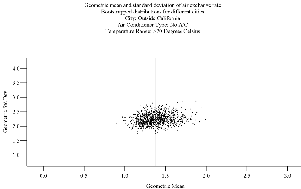
6 7 Figure 8-22. Example of boot strap simulation results used in evaluating random 8 sampling variation of AER (h-1) distributions (data from cities outside California).
