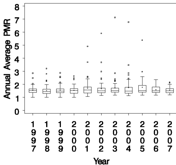
Figure 7-24. Distributions of annual average peak-to-mean ratios (PMRs) derived from the 98 monitors reporting both 5-minute maximum and 1-hour SO 2 concentrations, Years 1997 through 2007.
