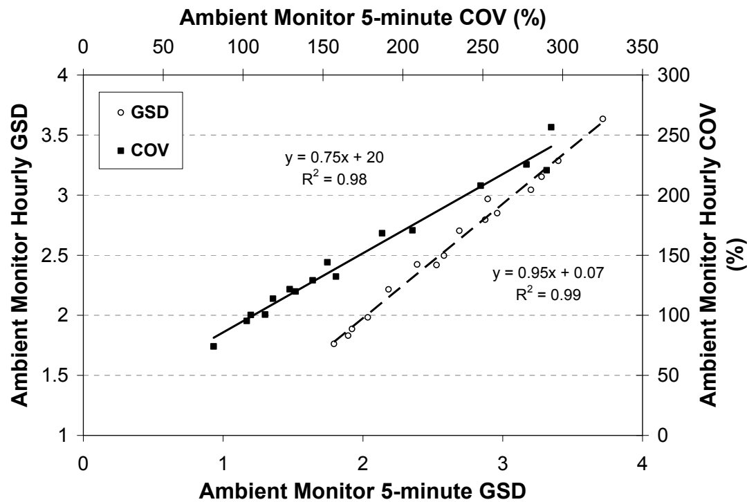
Figure 7-5. Comparison of hourly and 5-minute concentration COVs and GSDs at sixteen monitors reporting all twelve 5-minute SO 2 concentrations over multiple years of monitoring.
