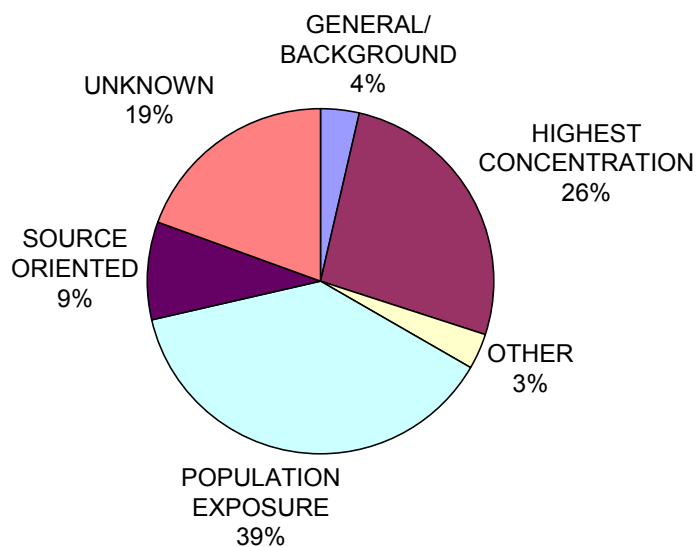
Figure 7-1. Distribution of site-years of data considering monitoring objectives and scale: monitors that reported 5-minute maximum \text{SO}_2 concentrations (top) and the broader \text{SO}_2 monitoring network (bottom).
