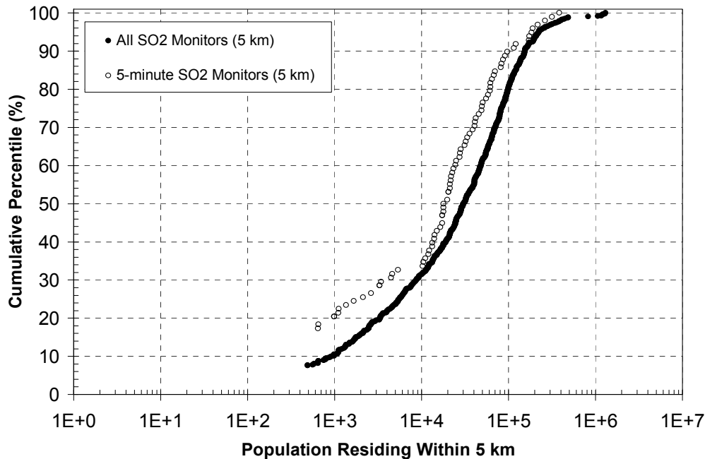
Figure 7-4. Distribution of the population residing within a 5 km radius of ambient monitors: monitors reporting 5-minute maximum SO 2 concentrations and the broader SO 2 monitoring network.
