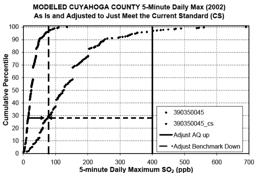
Figure 6-5. Comparison of adjusted ambient monitoring concentrations or adjusted benchmark level (dashed line) to simulate just meeting the current annual average standard at one ambient monitor in Cuyahoga County for year 2002.
