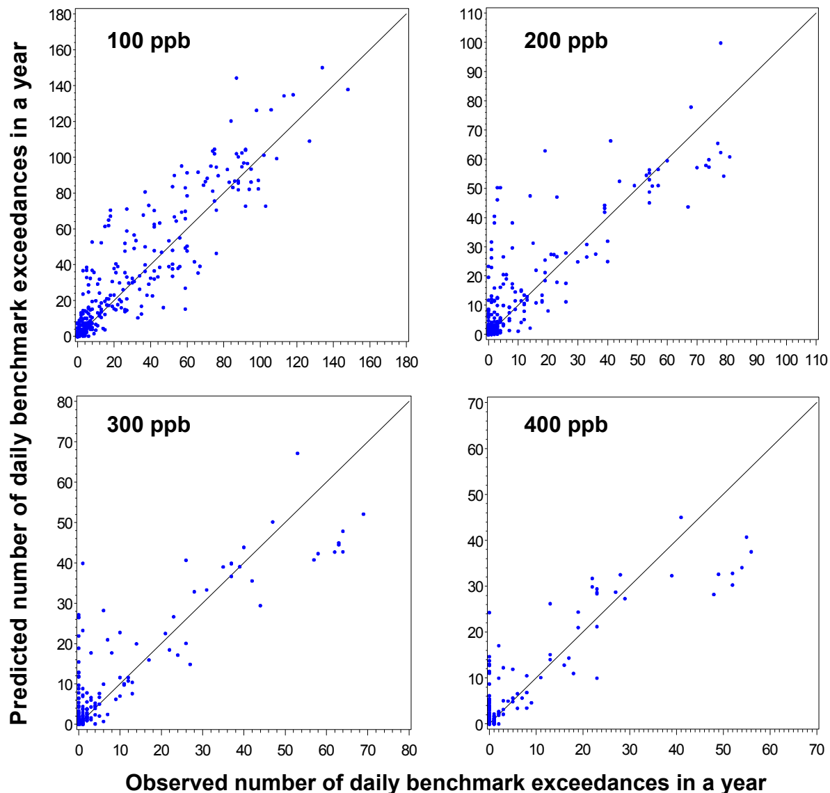
Figure 7-27. Comparison of observed and predicted number of daily benchmark exceedances in a year at monitors reporting 5-minute maximum SO 2 concentrations.
