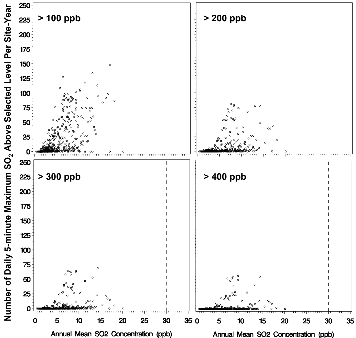
Figure 7-10. The number of measured daily 5-minute maximum SO 2 concentrations above potential health effect benchmark levels per year at 98 monitors given the annual average SO 2 concentration, 1997-2007 air quality as is. The level of the annual average SO 2 NAAQS of 30 ppb is indicated by the dashed line.
