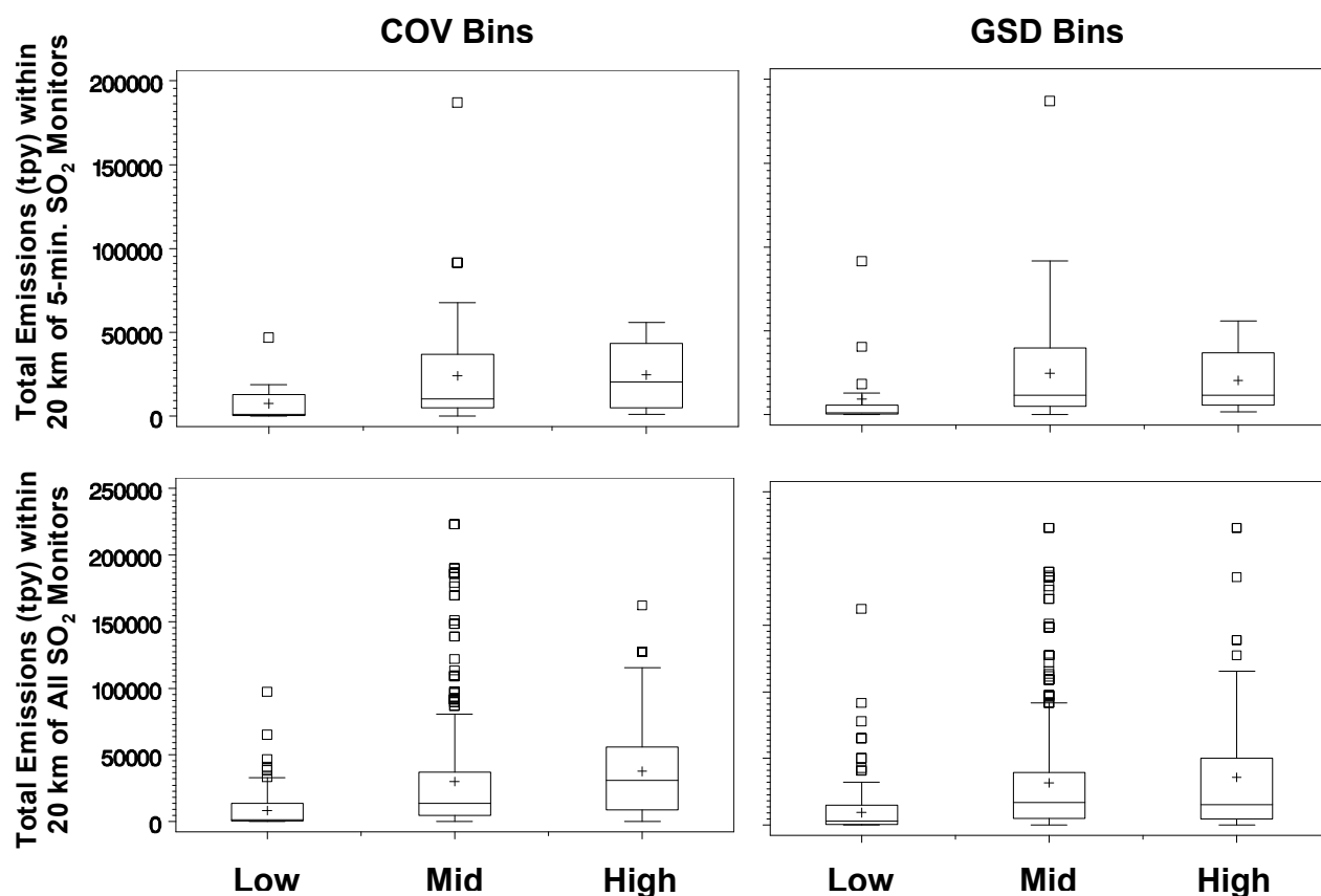
Figure 7-8. Distribution of total SO 2 emissions (tpy) within 20 km of monitors by COV (left) and GSD (right) concentration variability bins: monitors reporting 5-minute maximum SO 2 concentrations (top) and the broader SO 2 monitoring network (bottom).
