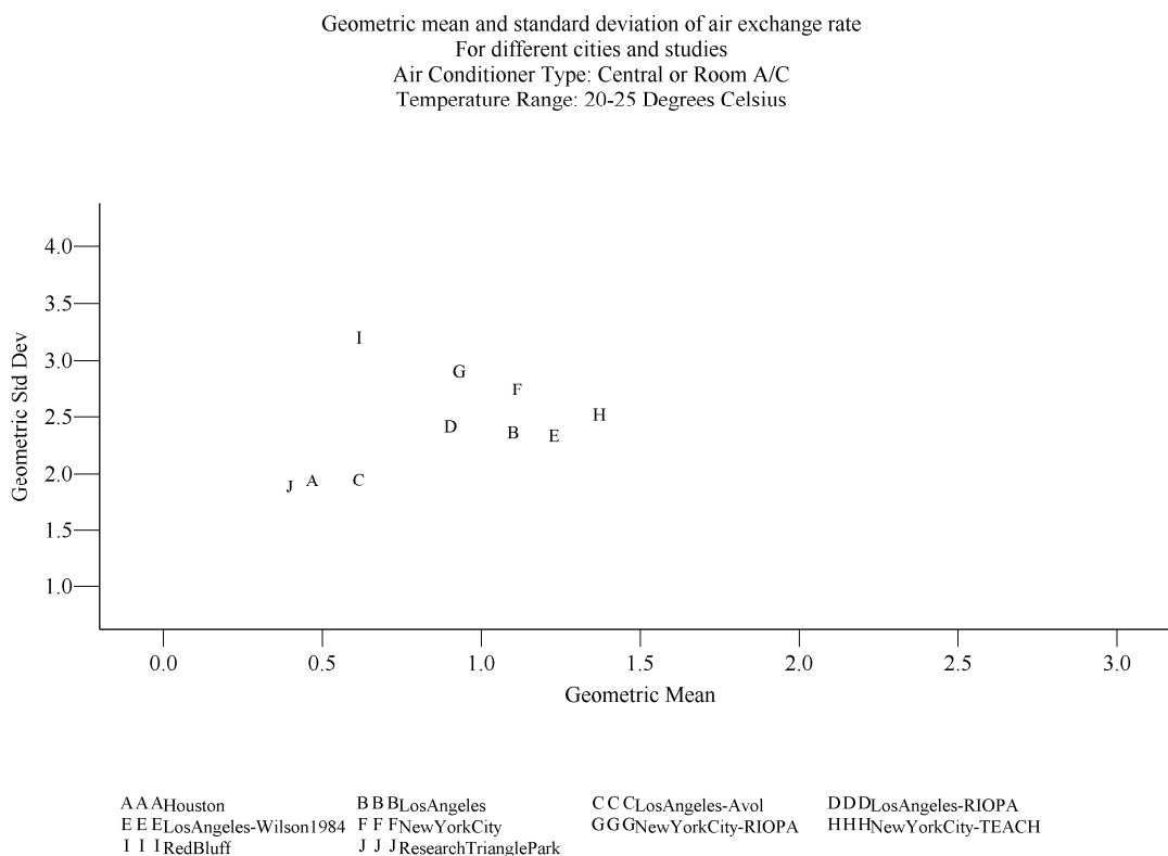
Figure 8-20. Example comparison of estimated geometric mean and geometric standard deviations of AER (h -1 ) for homes with air conditioning in several cities.
