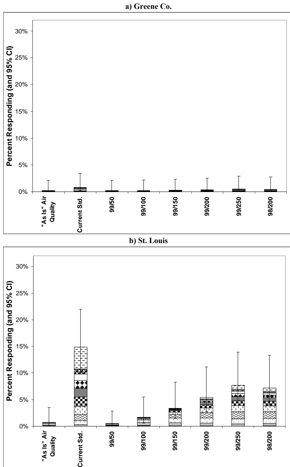
Figure 4-3. Percent of Asthmatics Engaged in Moderate or Greater Exertion Exhibiting Lung Function Response (Defined as a Decrease in FEV_1 \geq 15\% ) Attributable to SO_2 Within Given Ranges Under Different Air Quality Scenarios*
