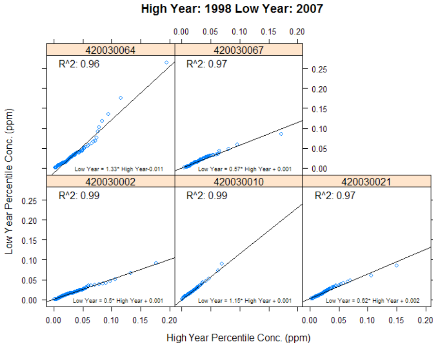
Figure 7-23. Comparison of measured daily maximum SO 2 concentration percentiles in Allegheny County PA for one high concentration year (1998) versus a low concentration years (2007) at five ambient monitors.
