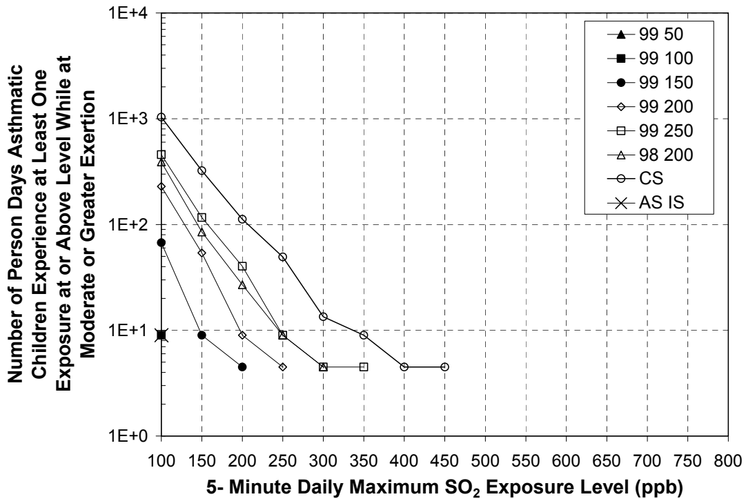
Figure 8-15. Number person days all asthmatics (top) and asthmatic children (bottom) experience 5-minute daily maximum SO 2 exposures above selected exposure levels in Greene County, year 2002 air quality as is and adjusted to just meeting the current and potential alternative standards.
