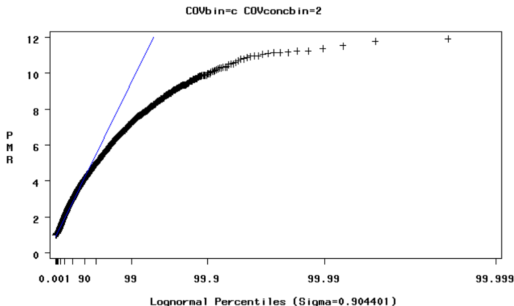
Figure 7-26. Example of a measured peak-to-mean ratio (PMRs) distribution with the percentiles of a fitted lognormal distribution.
