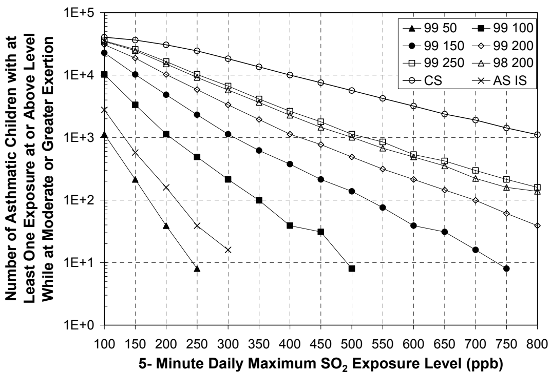
Figure 8-16. Number of all asthmatics (top) and asthmatic children (bottom) with 5-minute daily maximum SO 2 exposures above selected exposure levels in St. Louis, year 2002 air quality as is and adjusted to just meeting the current and potential alternative standards.
