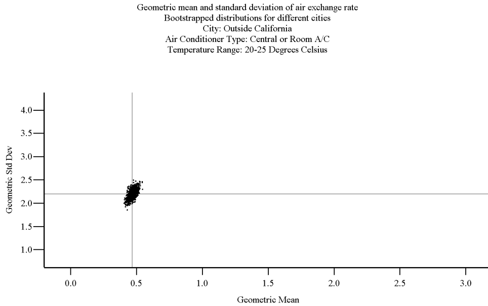
1 2 Figure 8-21. Example of boot strap simulation results used in evaluating random sampling 3 variation of AER (h-1) distributions (data from cities outside California).
