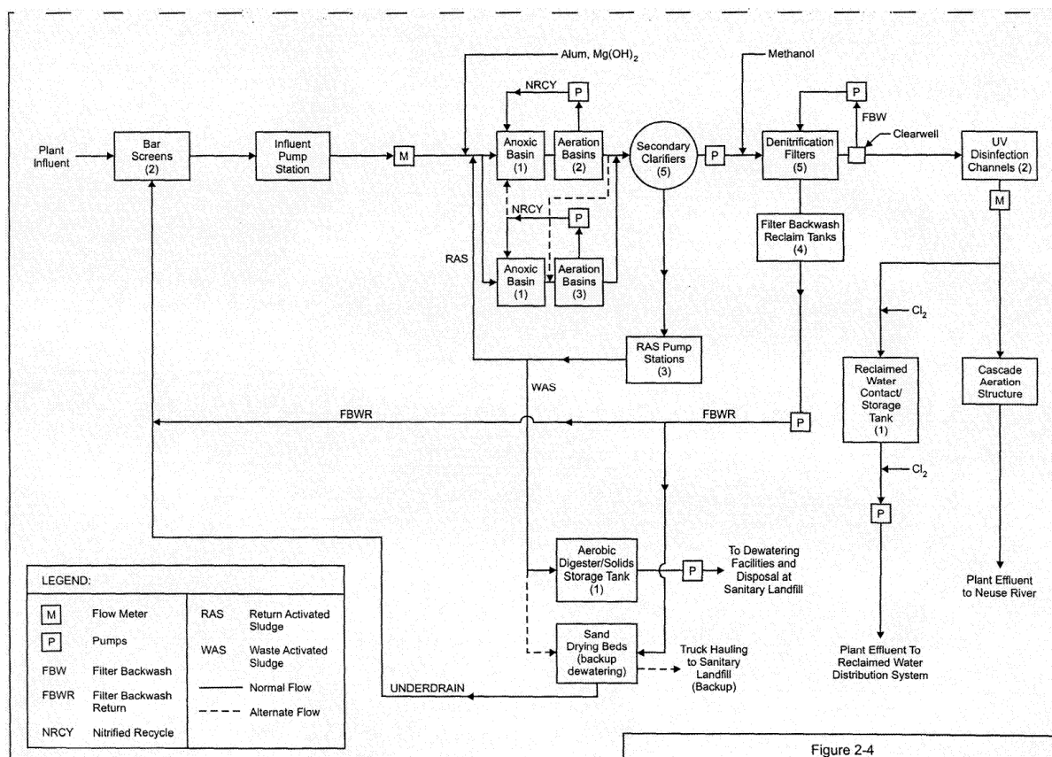
Figure 2. Central Johnston County WWTP process schematic.
