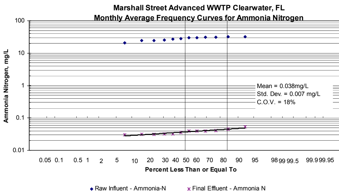
Figure 3-10. Marshall Street Advanced WWTP, Clearwater, Florida: Monthly average frequency curves for ammonia nitrogen.
