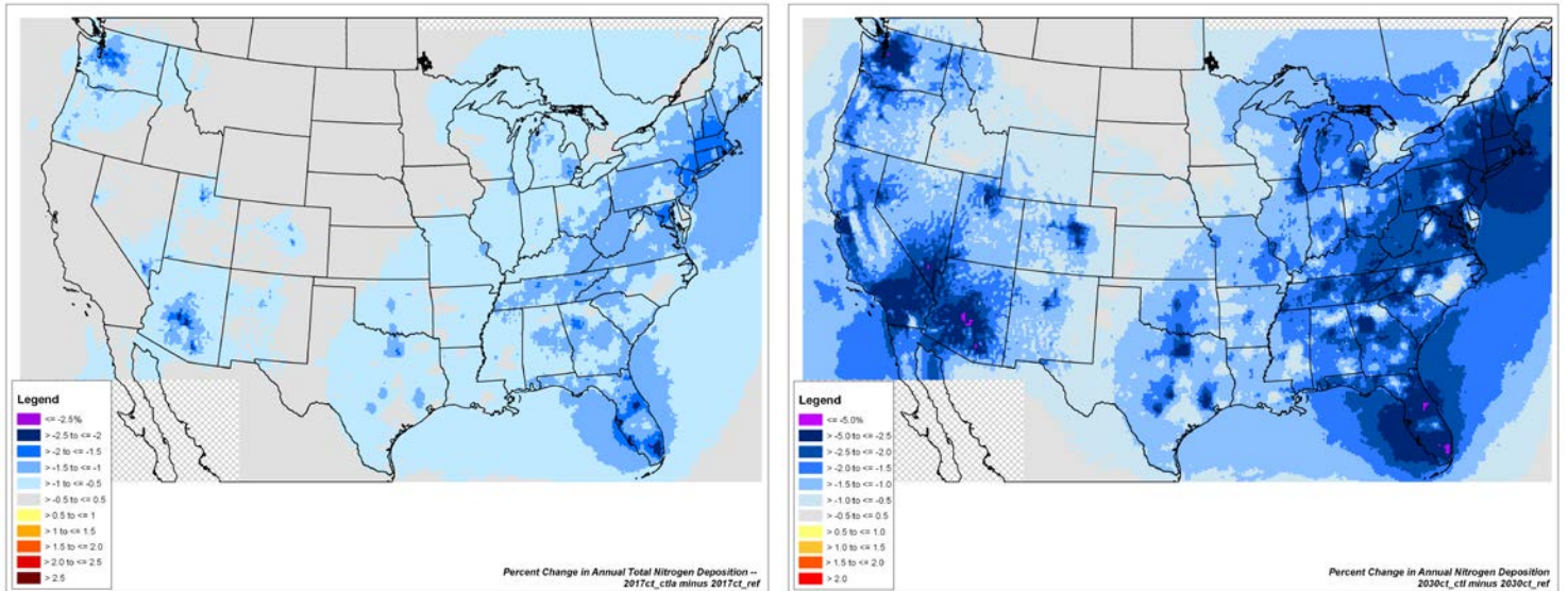
Figure III-21. Percent Changes in Annual Total Nitrogen Deposition Between the Reference Case and the Control Case in 2017 (left) and 2030 (right)
