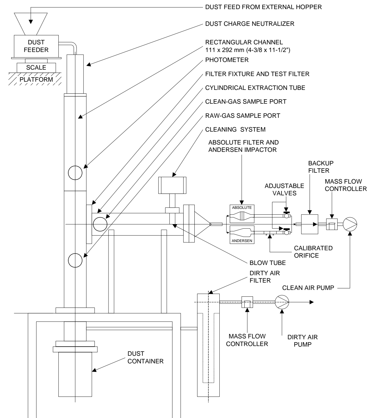
Figure 1. Diagram of filtration efficiency media analyzer test apparatus.
