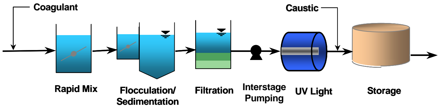
Exhibit 3.4: Plant Schematic for UV Disinfection
