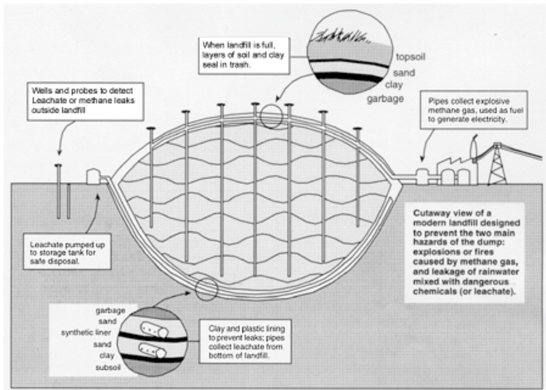
Figure II-4: Cross-Section of a Municipal Solid Waste Landfill
