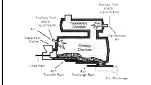
Figure III-24: Cross-Section of an Incinerator
