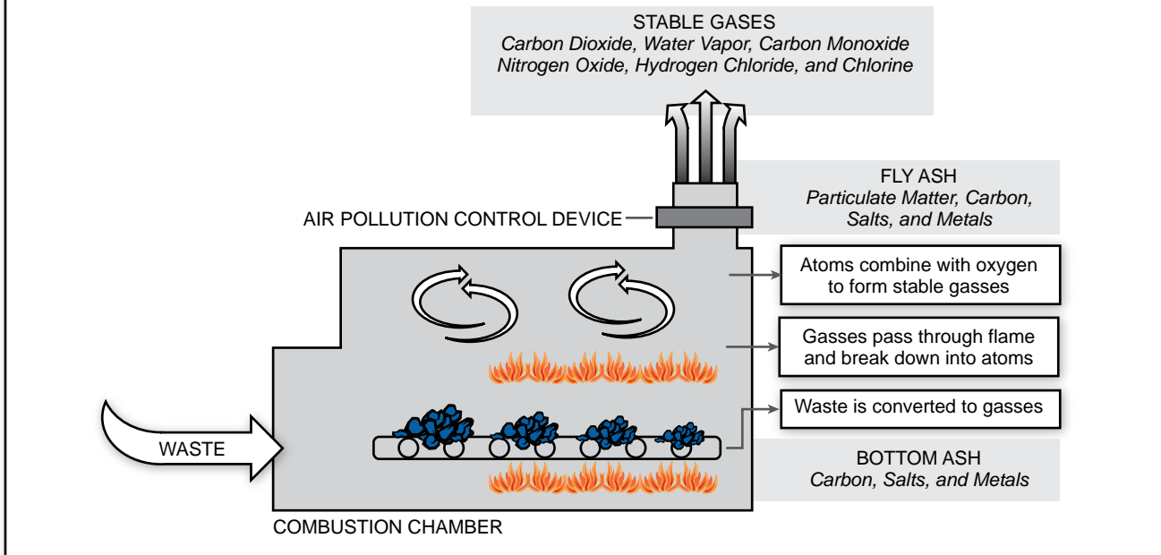
Figure III-23: The Combustion Process
