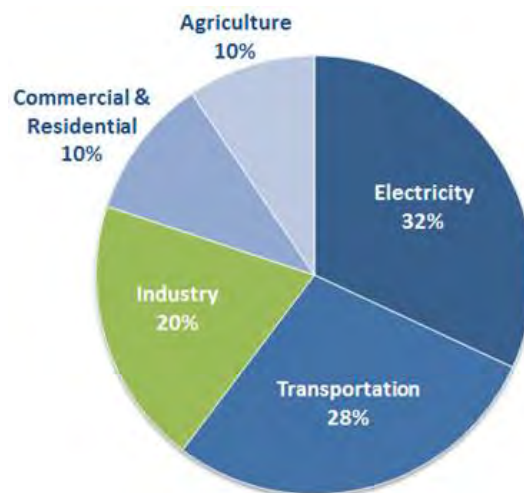
Figure 1: 2013 Total U.S. Greenhouse Gas Emissions by Sector 3
