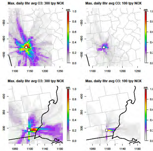
Figure 5-4. Spatial plot of ozone season highest daily 8-hr maximum O 3 from the hypothetical source NO x emissions.
