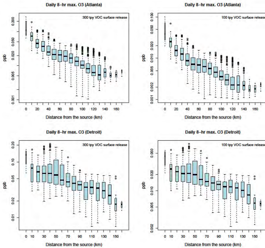
Figure 5-5. Distribution of ozone season highest daily 8-hr maximum O 3 by distance from the hypothetical source VOC emissions. Results for Atlanta on top row and Detroit the bottom row.
