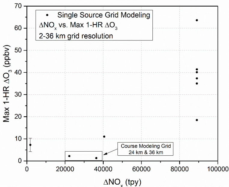
Figure 6-1. Published single source NO x emissions impacts on downwind hourly O 3 estimated using photochemical grid modeling.
