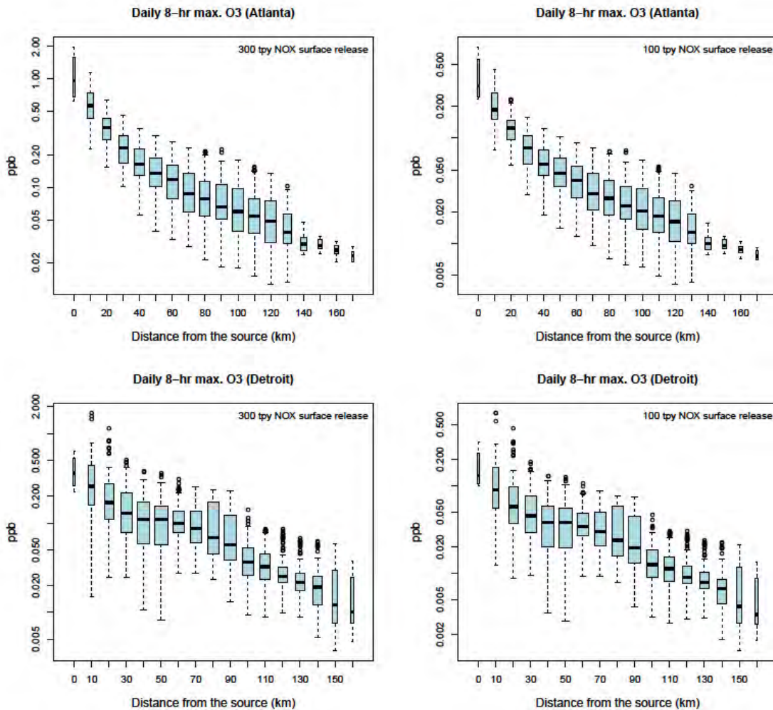
Figure 5-3. Distribution of ozone season highest daily 8-hr maximum O 3 by distance from the hypothetical source NO x emissions. Results for Atlanta are shown on the top row and Detroit the bottom row.
