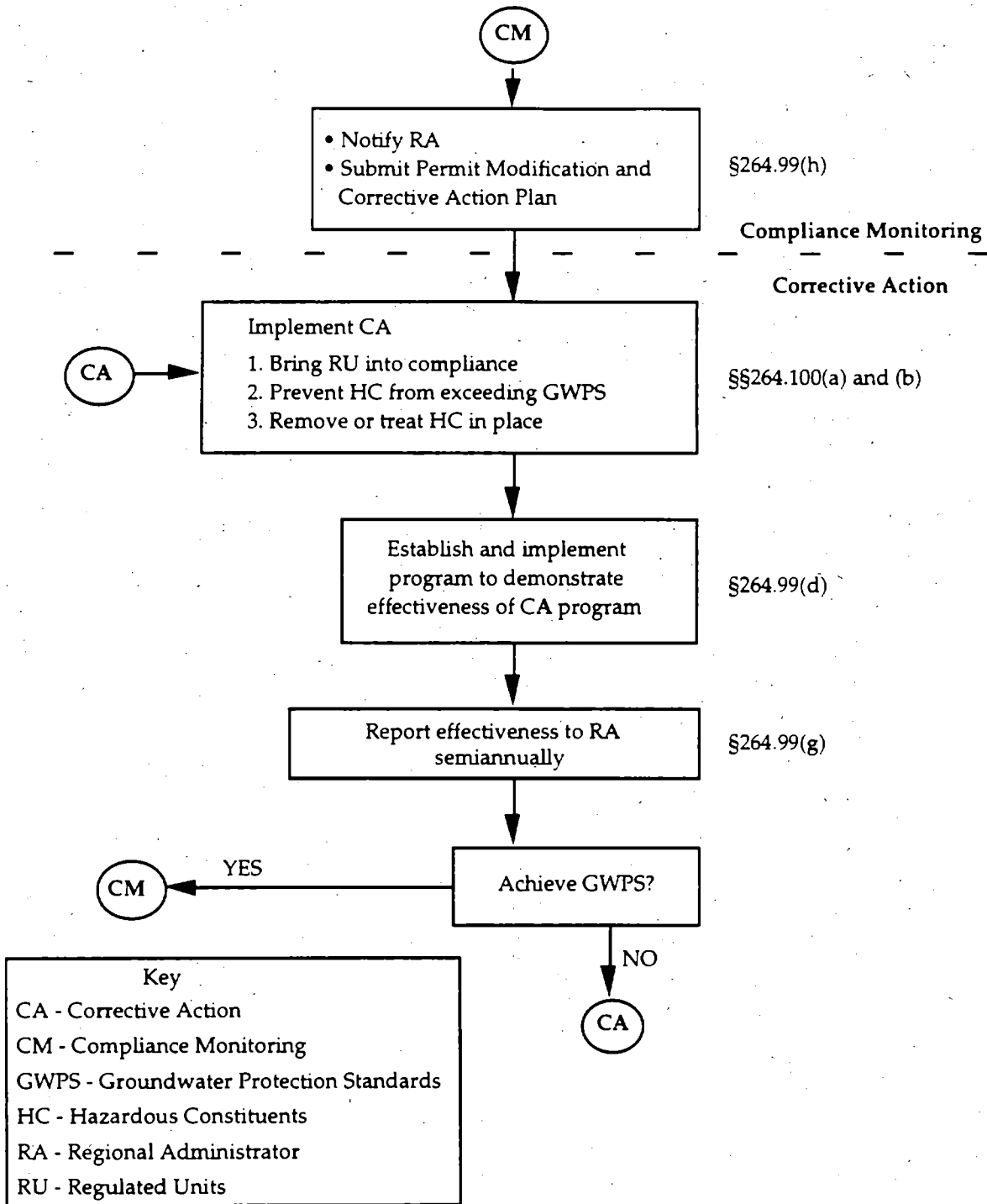
Figure 8 OVERVIEW OF THE CORRECTIVE ACTION PROGRAM (§264.100)
