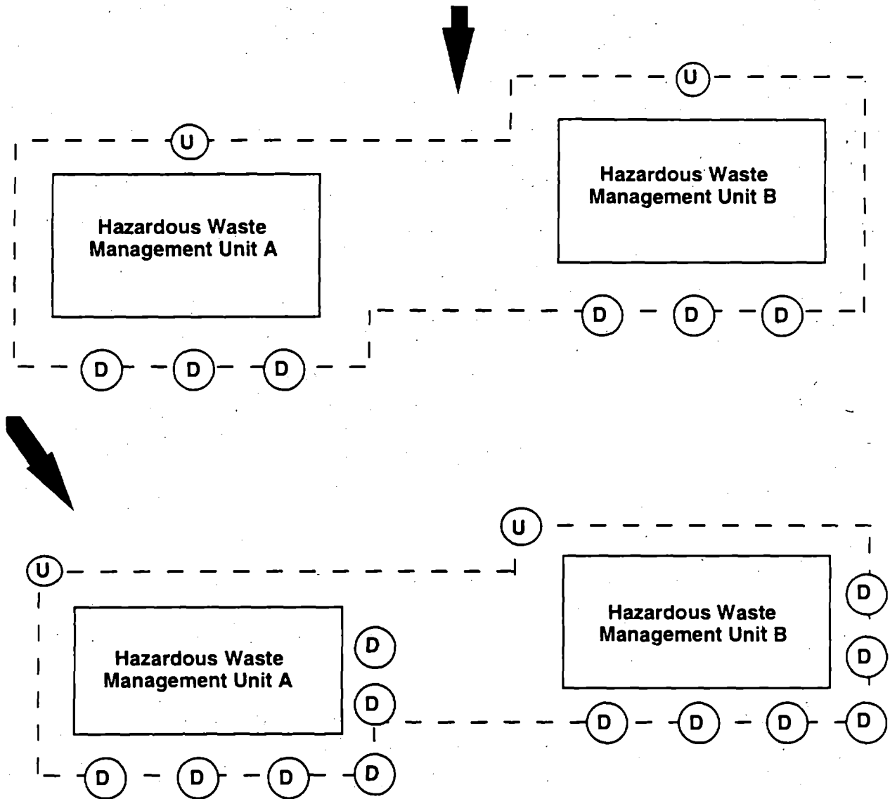
Figure 4 EXAMPLES OF GROUNDWATER MONITORING SYSTEMS FOR MULTIPLE REGULATED UNITS
