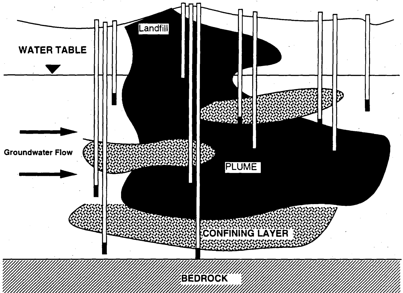
Figure 10 SAMPLE OF ASSESSMENT PHASE MONITORING WELL PLACEMENT
