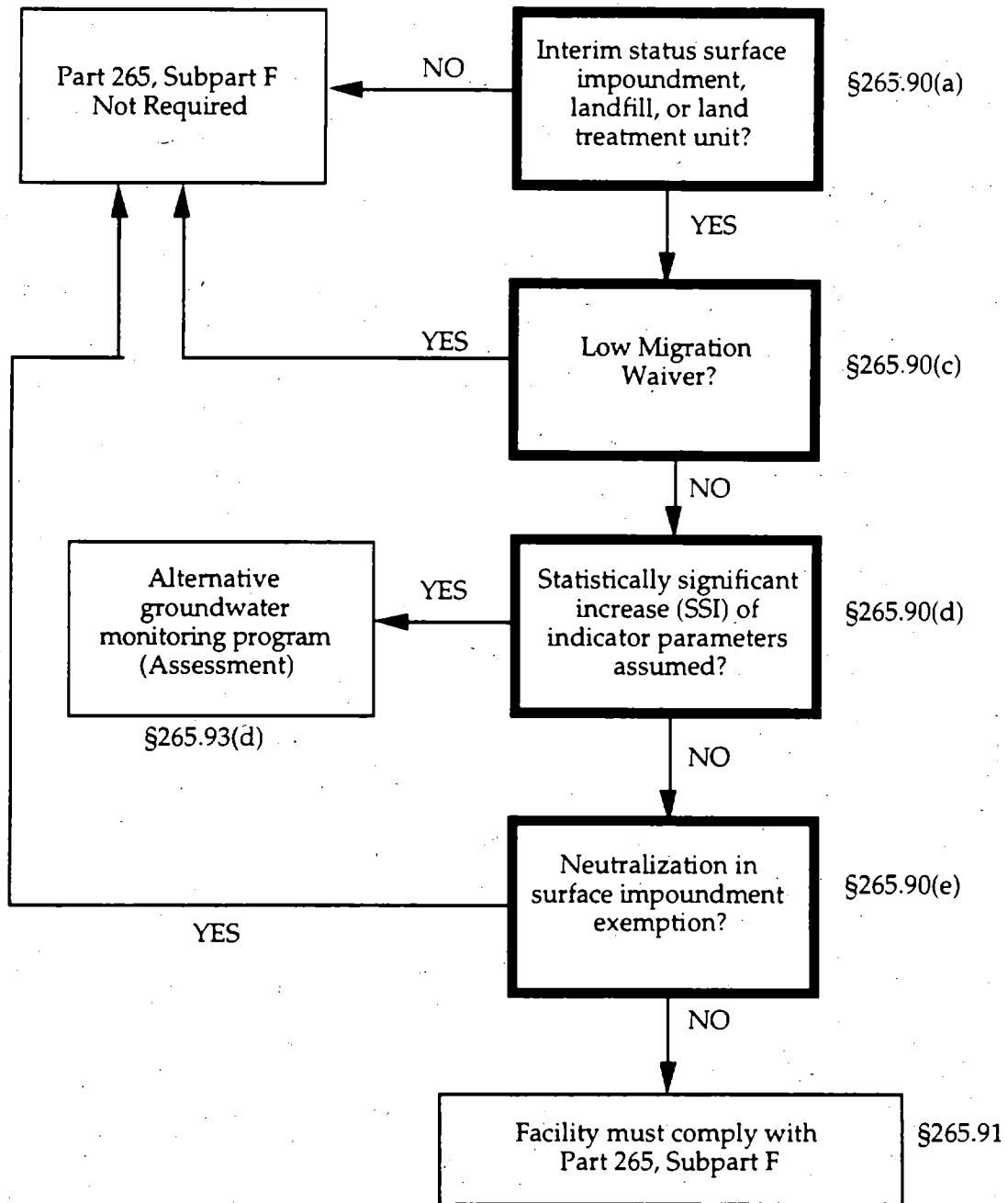
Figure 9 APPLICABILITY OF GROUNDWATER MONITORING FOR INTERIM STATUS FACILITIES
