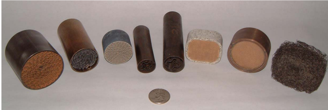
Figure 5-3: Some of the catalyst substrate types evaluated by EPA with Class I and Class II engines included (from left to right) 100 cpsi metal monoliths (in 50 mm and 33 mm diameters); 200 cpsi metal monolith; catalyzed tube pre-catalysts (in 20 mm and 25 mm diameters); 400 cpsi coridierite (square-oval and round) and metal-mesh. The 50 mm diameter catalyst on the far left was used with Class II engine test configurations. The remaining catalysts were tested with Class I engines.
