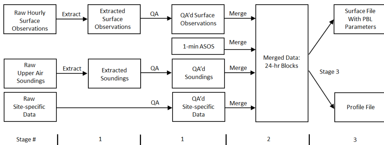
Figure 1-1. AERMET Processing
