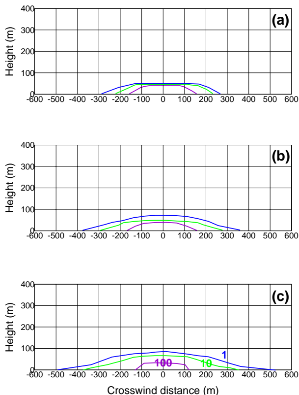
Figure 7. Gaussian plume model results using AERMOD. Plume cross sections at downwind distances of: a) 300m, b) 600m, and c) 1200m. View looking upstream.
