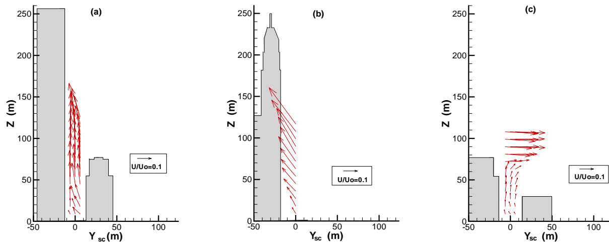
Figure 5. Velocity vectors on the downwind side of tall buildings (shown in silhouette on the left side of each figure. a) Chase Manhattan building (Federal Reserve building on right), b) Woolworth building, c) unknown building approximately 300m northeast of WTC site.
