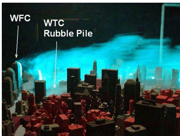
Figure 3. Visualization of smoke in a vertical plane parallel to the direction of the freestream flow (from left to right).
