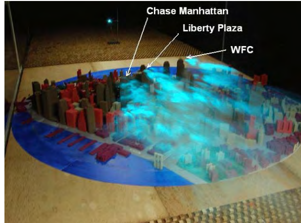
Figure 4. Visualization of smoke in a horizontal plane just above the height of the tallest buildings using a laser light sheet.
