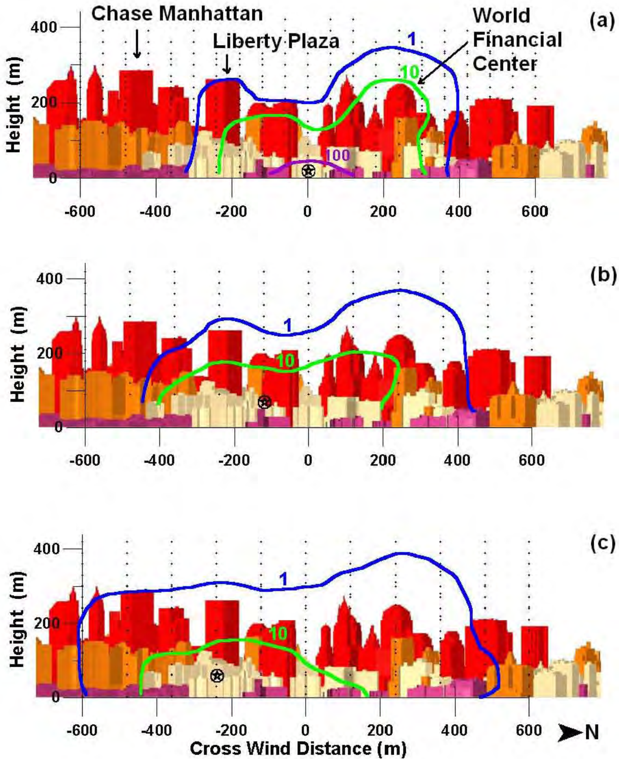
Figure 6. Plume cross sections at downwind distances of: a) 300m, b) 600m, and c) 1200m. View looking upstream against skyline of city. Shorter buildings indicated in lighter colors.
