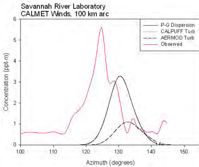
Figure 3.5.2 – Example of azimuth of fitted plume on receptor arc.
