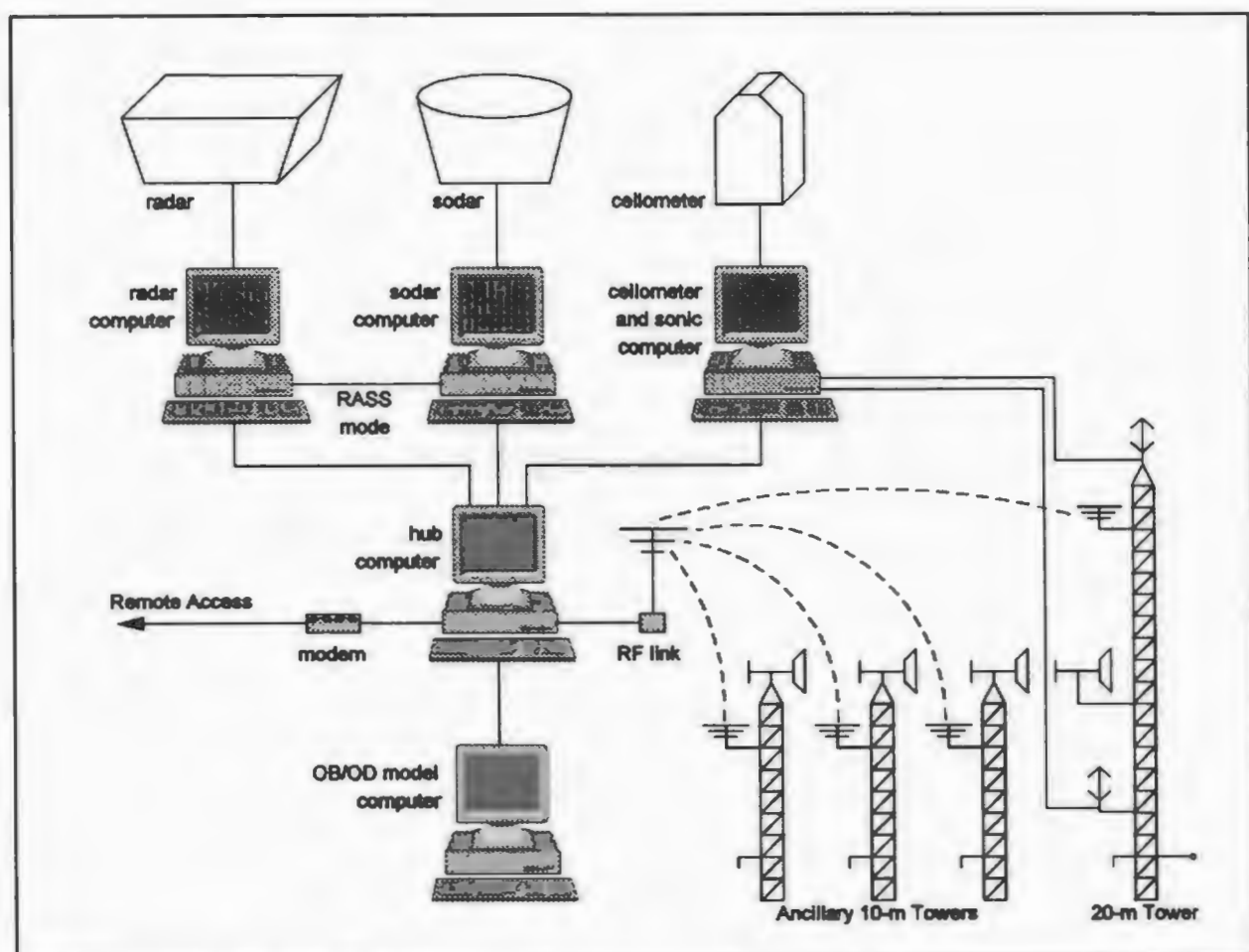
Figure 2. Schematic of mobile meteorological monitoring system.
