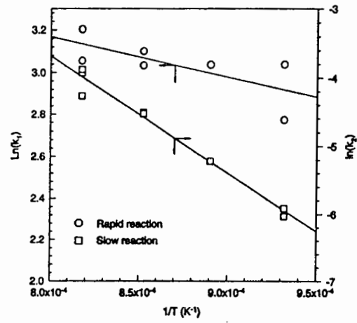
Figure 5. Arrhenius plots of the rate constants.
