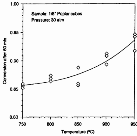
Figure 4. Effect of reaction temperature.
