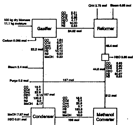
Figure 1. Schematic flow diagram of the Hynol process.
