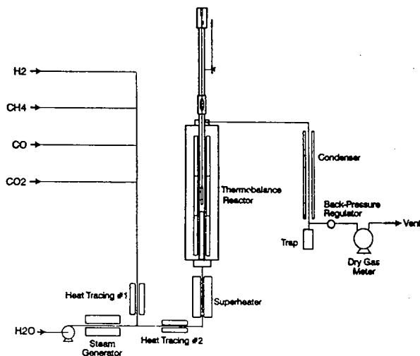
Figure 2. Flow diagram of the TBR system.
