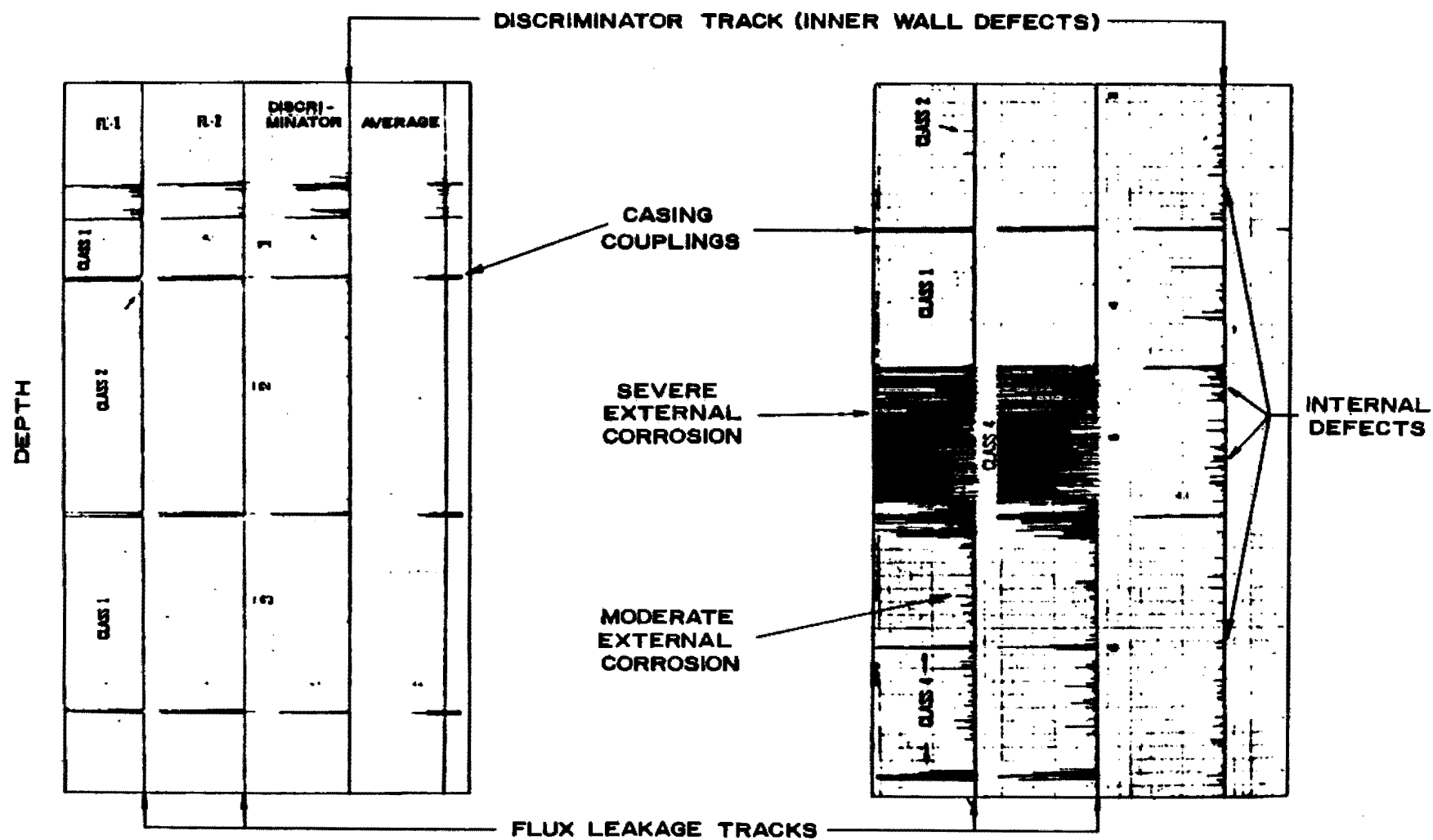
Figure 13 TYPICAL DISPLAY OF THE VERTILOG
