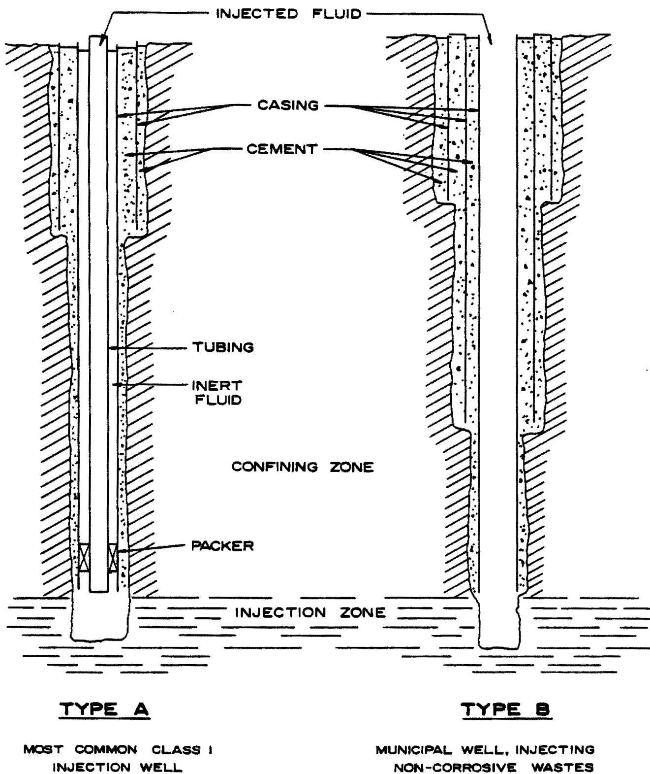
Figure 2 CLASS 1 INJECTION WELLS
