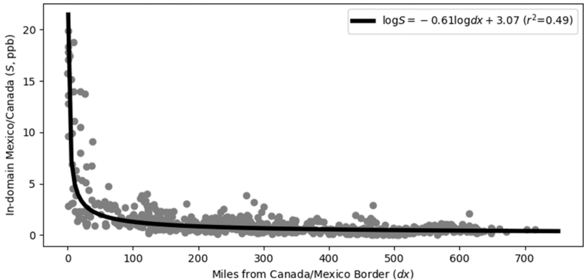
Figure 4. Mexico/Canada source contribution ( S ) in 2023 at monitors by distance from border ( dx ).
