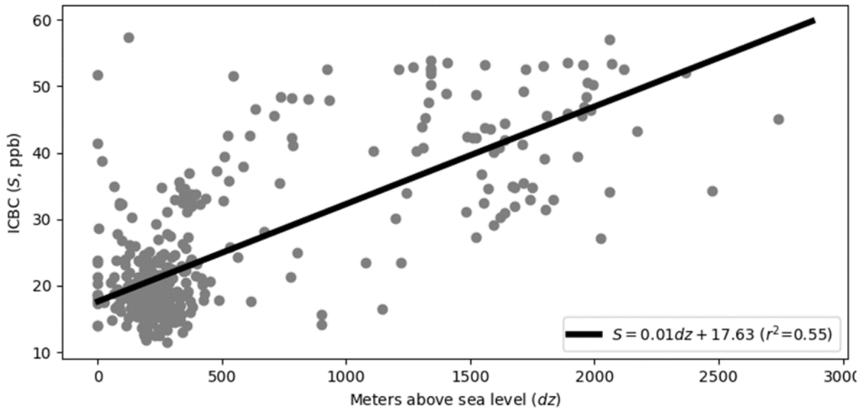
Figure 5. Initial and Boundary Conditions contribution (ICBC) to projected 2023 design values as a function of elevation at AQS monitors that are farther than 100 miles from the border.
