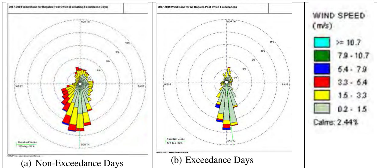
Figure 7. Nogales, Arizona PM10 nonattainment area: wind roses for non-exceedance and exceedance days (ADEQ, 2012, pp. Appendix A, Figure 9)
