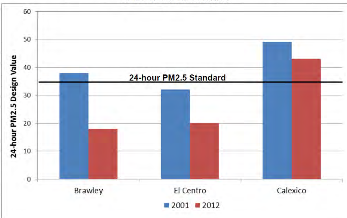
Figure 2. 2001 and 2012 24-hour PM 2.5 Design Values for three Monitoring Sites in Imperial County, California (CARB, 2014, pp. 15, Figure 2.5) 36
