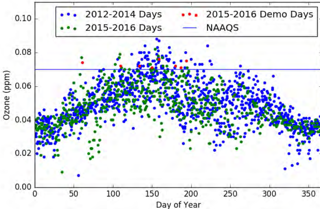
Figure 6. Measured O_3 as a function of day-of-year with example days highlighted as influenced by international sources marked in red and other days marked in green.
