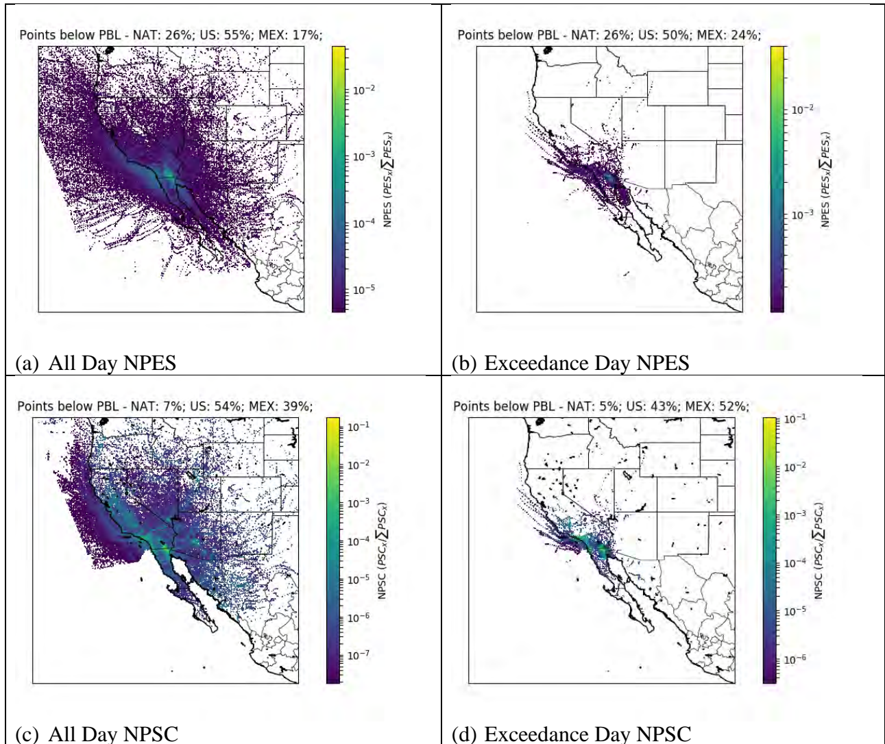
Figure 9. Imperial County, California O_3 nonattainment area: El Centro 72-hour back trajectory Normalized Potential Emission Sensitivity maps (a,b) and Normalized Potential Source
