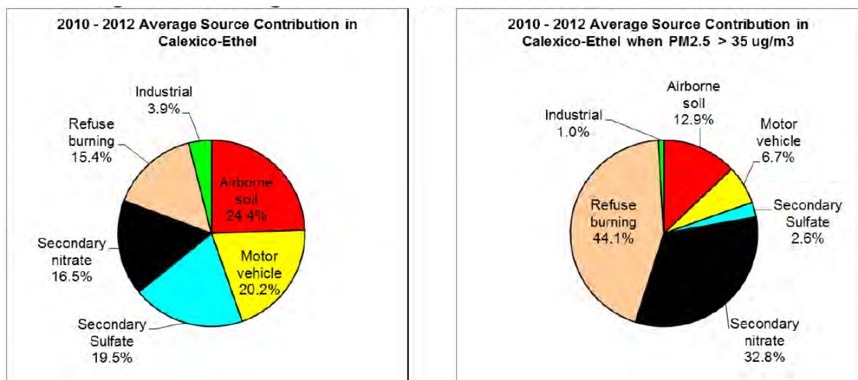
Figure 11. Average source contributions between 2010 and 2012 (CARB, 2014, p. Figure B2) 49
