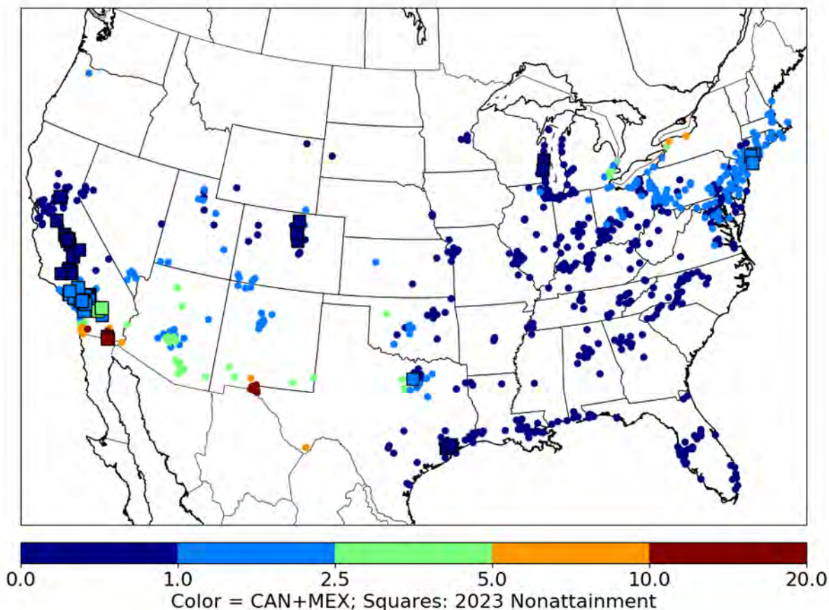
Figure 3. O 3 (fourth highest maximum daily 8-hour average) contributions from in-domain Mexican and Canadian anthropogenic emissions at AQS monitors in 2023 projections. Monitors that are projected as nonattainment in 2023 are outlined squares and all other monitors are smaller circles.
