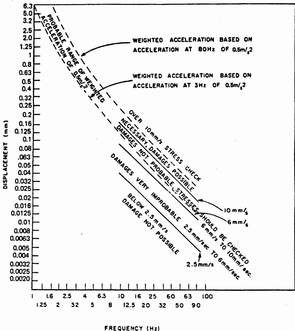
FIGURE D-3. Rough evaluation of vibrations of stationary floor vibrations by measurement of vibration displacements amplitude and frequency
