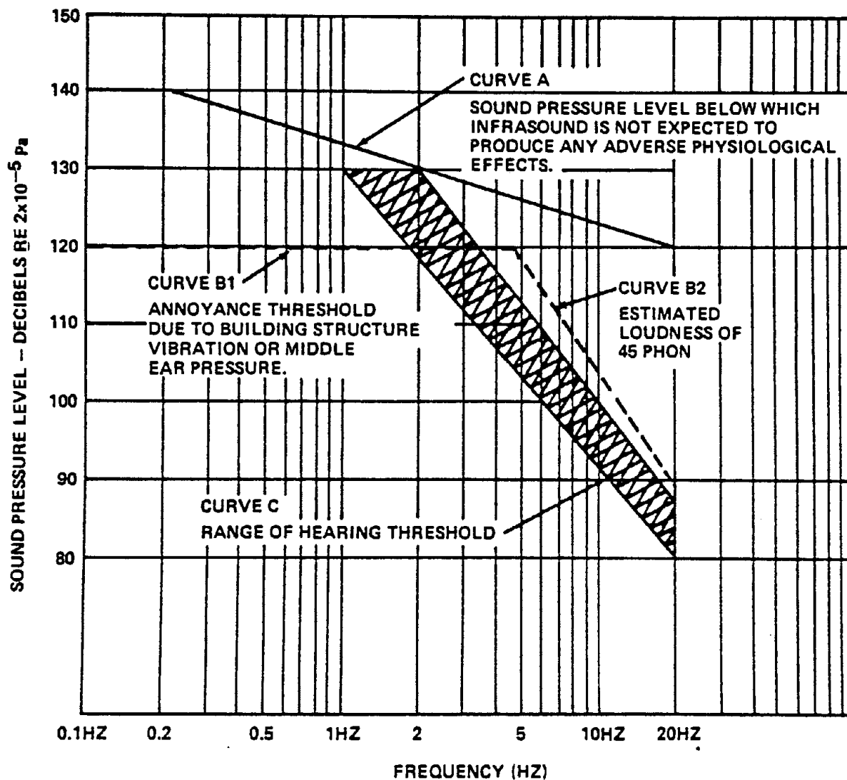
FIGURE 10. INFRASOUND CRITERIA
