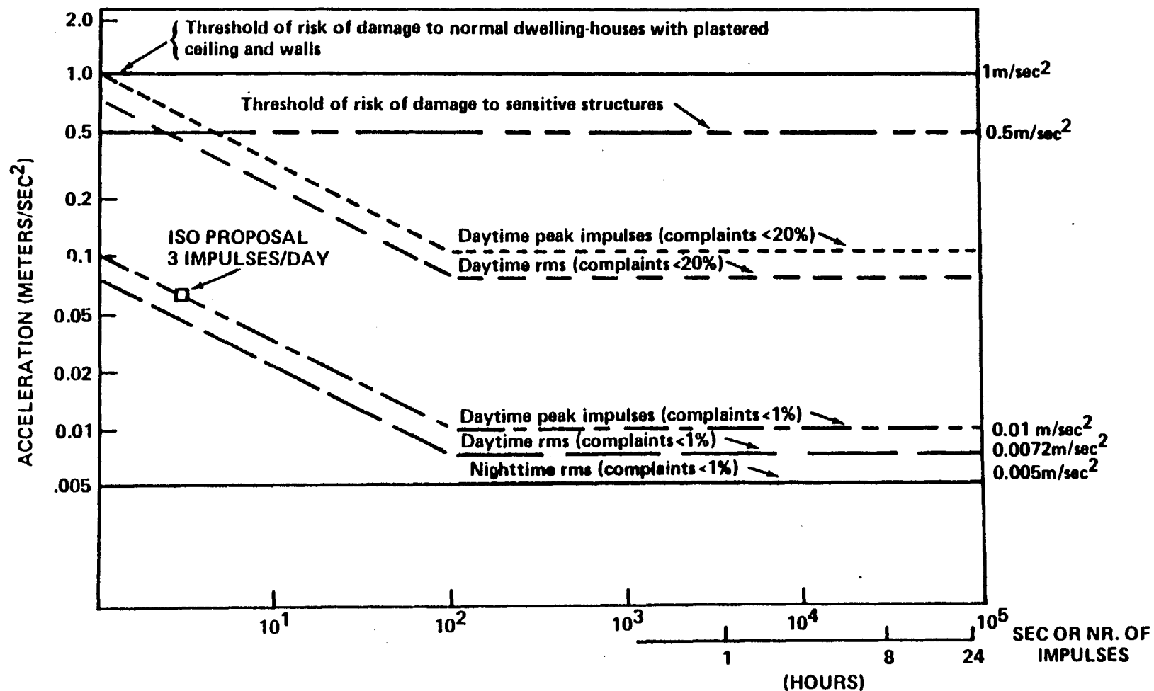
NUMBER OF IMPULSES PER DAY OR EXPOSURE TIME FIGURE 12. VIBRATION CRITERIA FOR RESIDENTIAL AREAS
