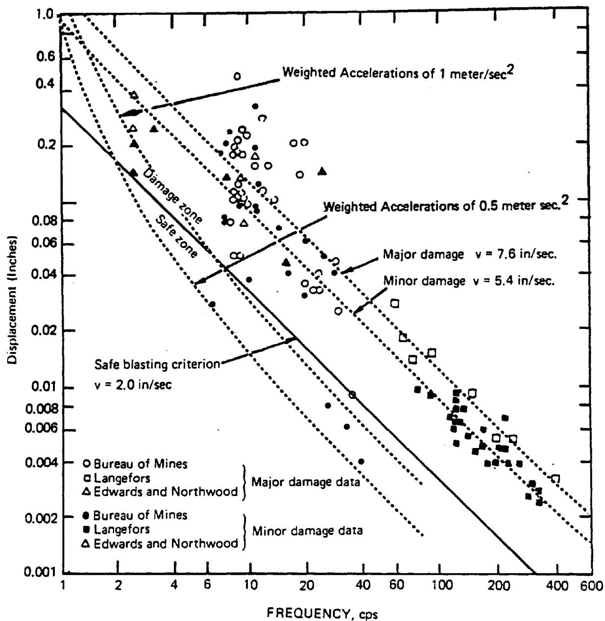
FIGURE D-4. Displacement versus frequency, combined data with recommended safe blasting criterion
