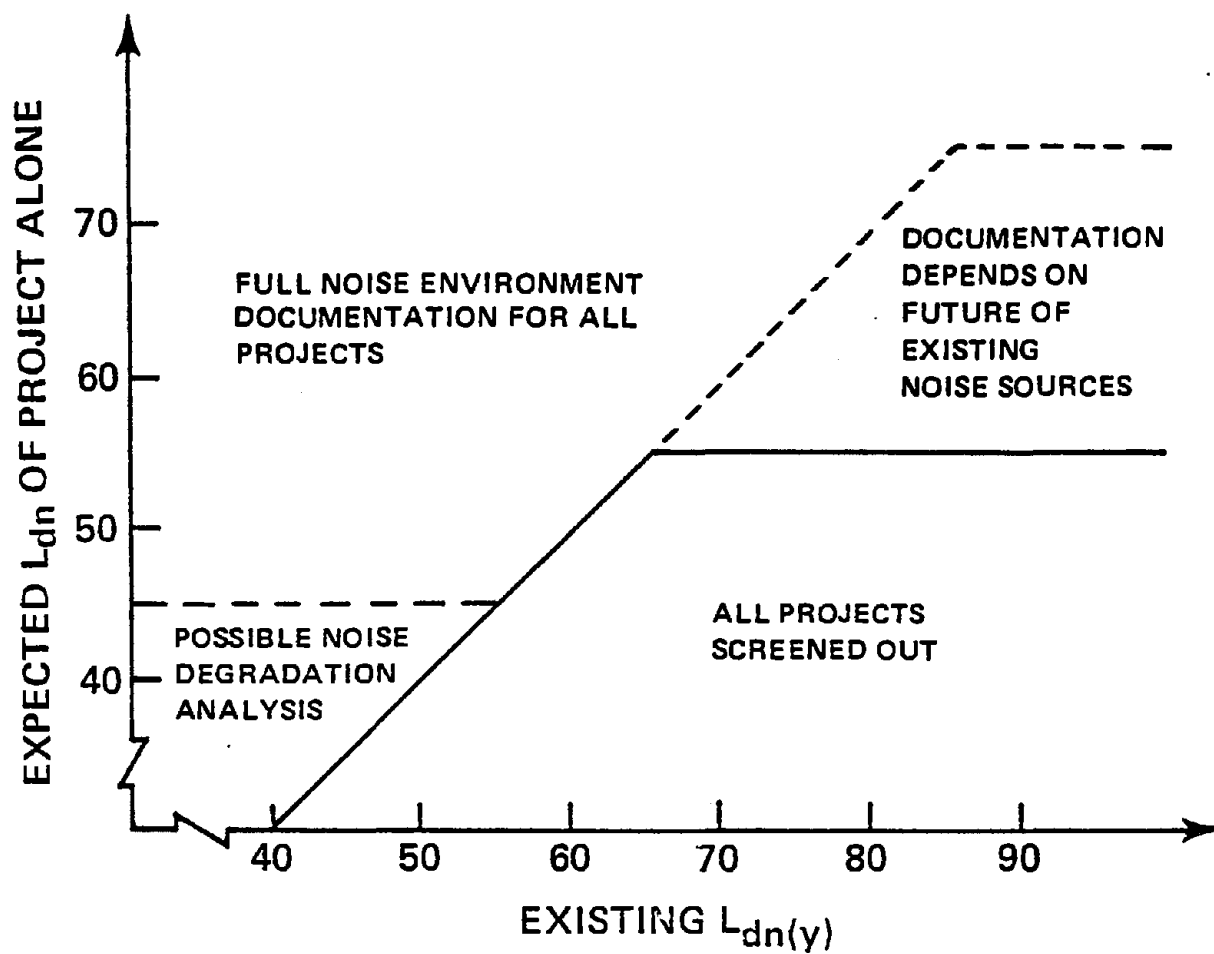
FIGURE 3. SCREENING DIAGRAM
