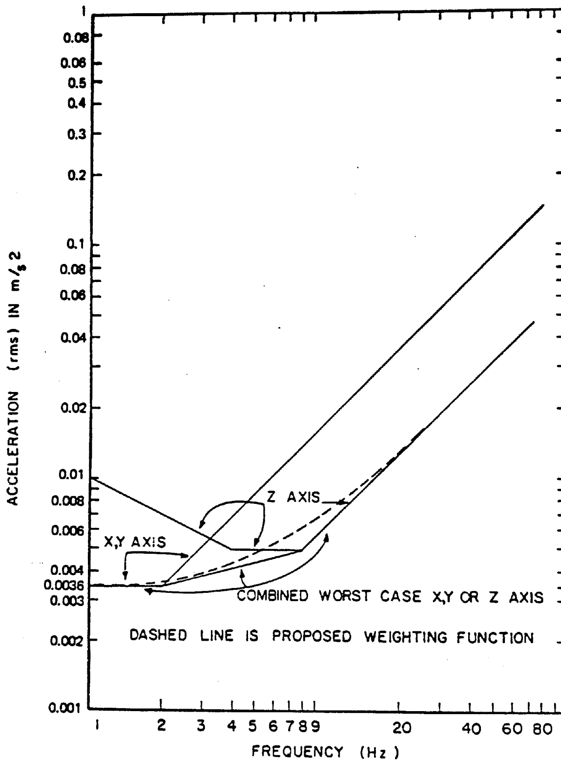
FIGURE D-2. Building vibration criteria for occupants in buildings. All curves are for hospital and critical working areas. See Table D-2 for proper scale factors.
