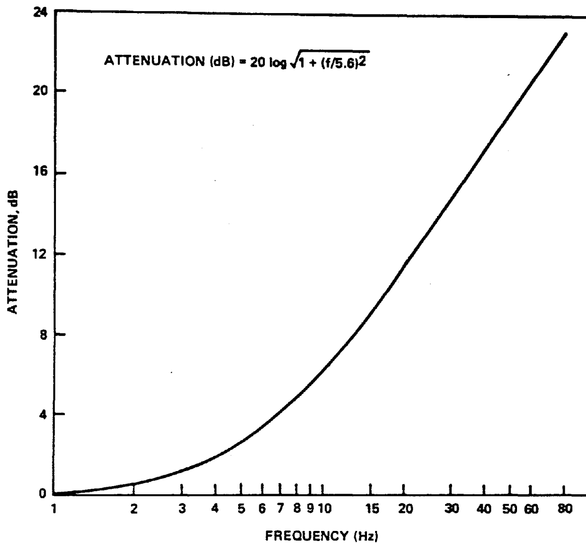
FIGURE 11. WEIGHTING CHARACTERISTIC FOR BUILDING VIBRATION IN TERMS OF HUMAN RESPONSE FOR THE FREQUENCY RANGE 1 TO 80 Hz.
