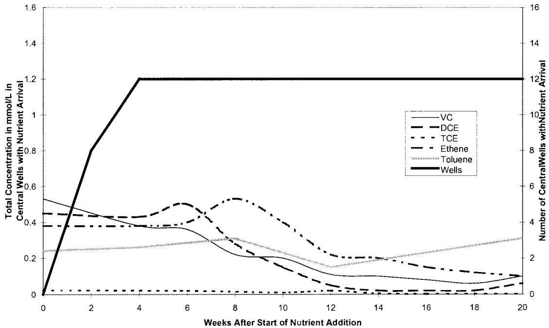
Figure 10. Contaminant monitoring data for Level C and D Wells.
