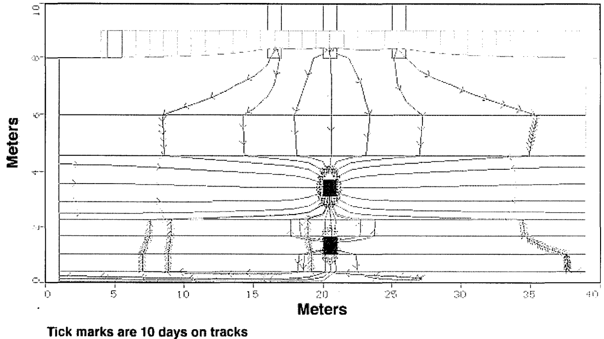
Figure 6. MODFLOW model of system ground water flow patterns and transit times.
