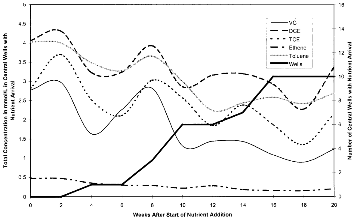
Figure 9. Contaminant monitoring data for Level A and B Wells.
