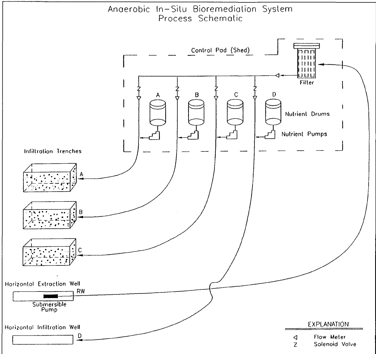
Figure 7. Bioremediation pilot system process diagram.
