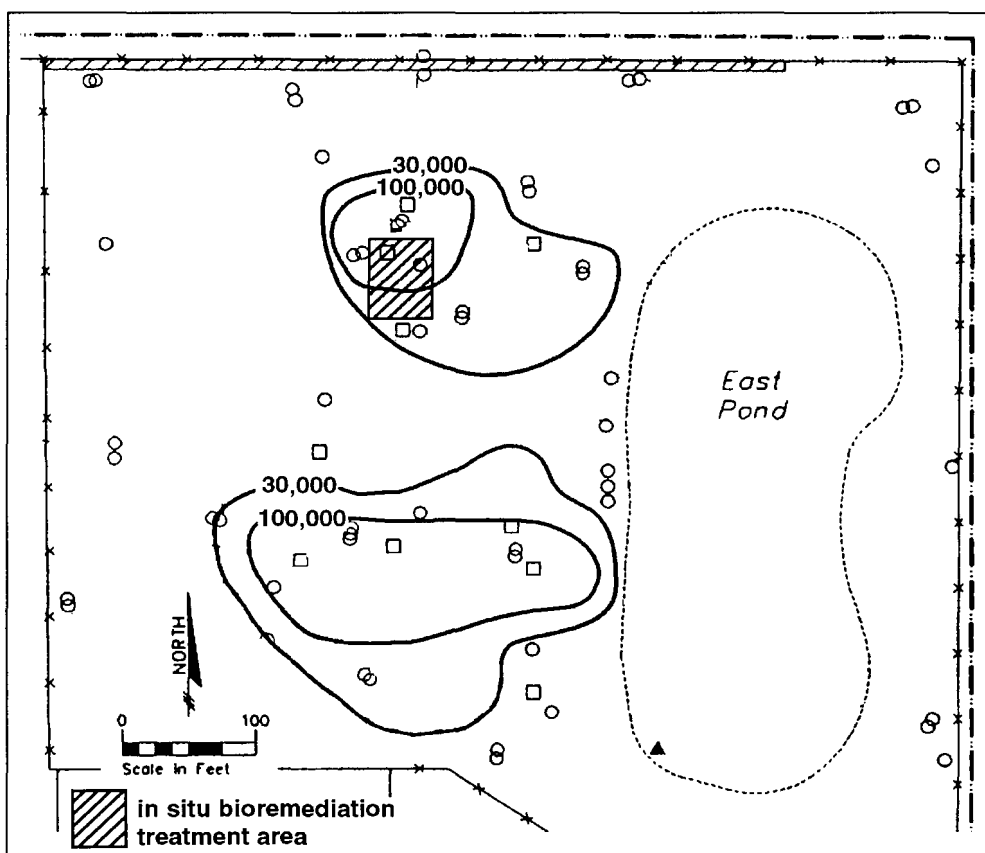
Figure 3. Total VOCs in ground water (in \mu\text{g/L} ).
