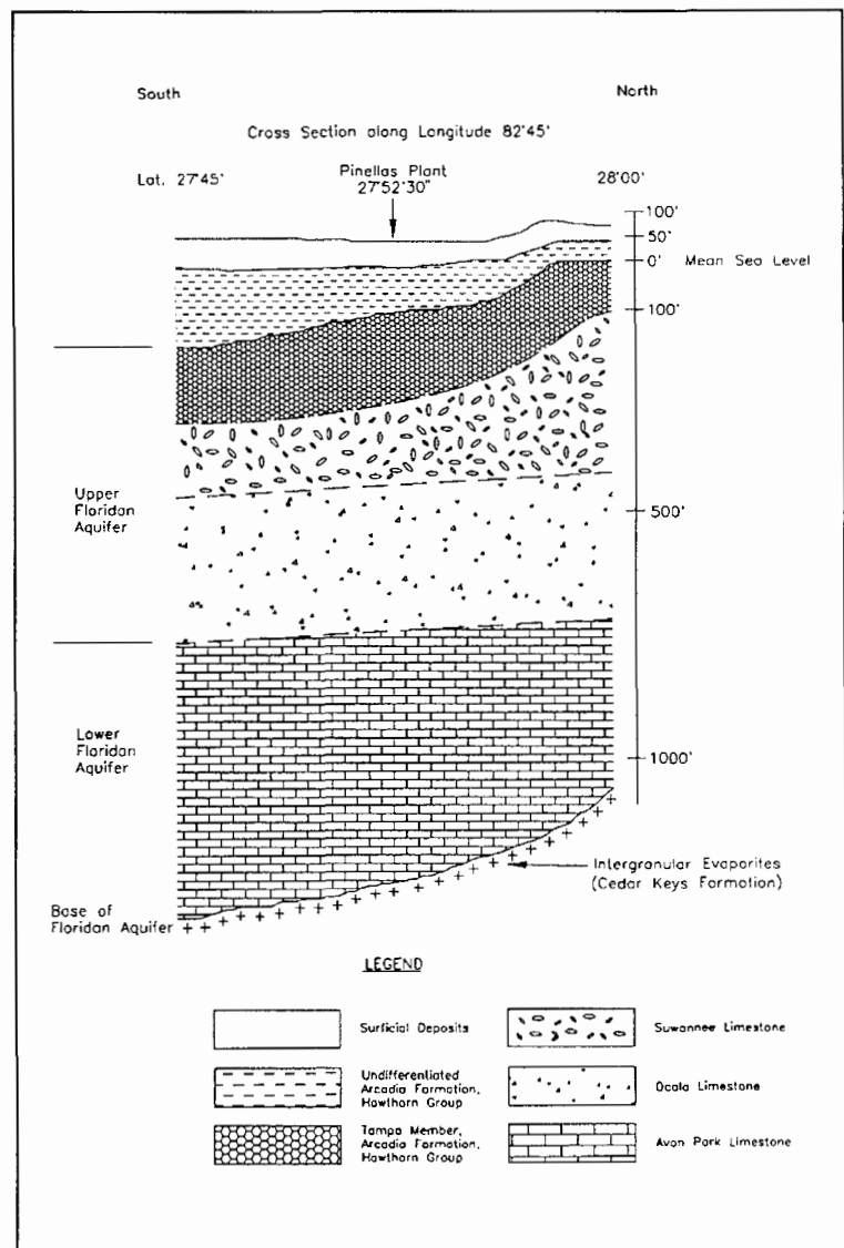
Figure 2. Geologic section at the Pinellas STAR Center.
