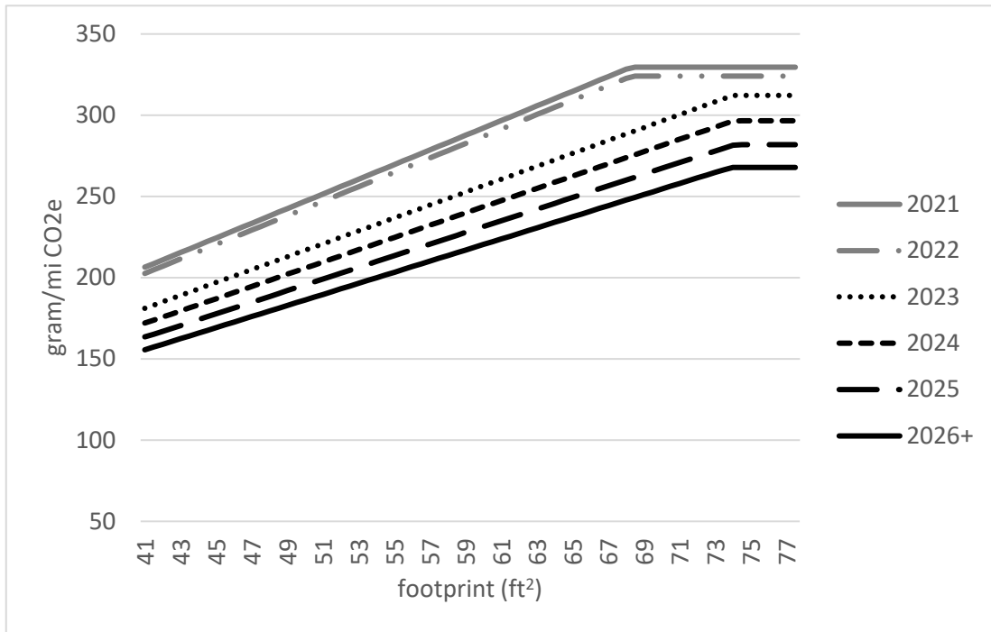
Figure 2-2: CO 2 vs Footprint Compliance Curves for Trucks
