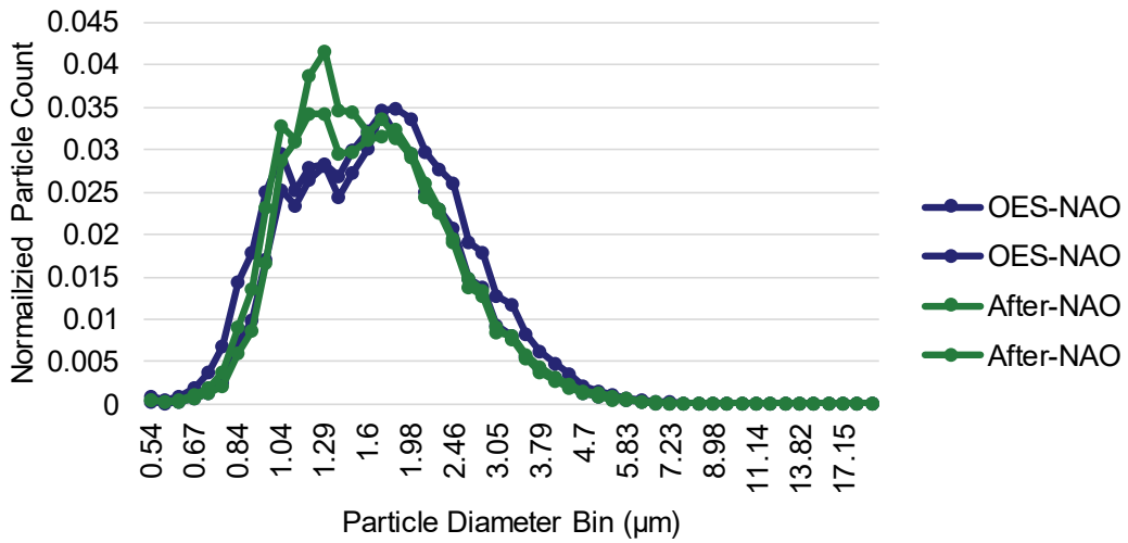
Figure 65. Size distribution of Prius front brake PM as measured by APS
