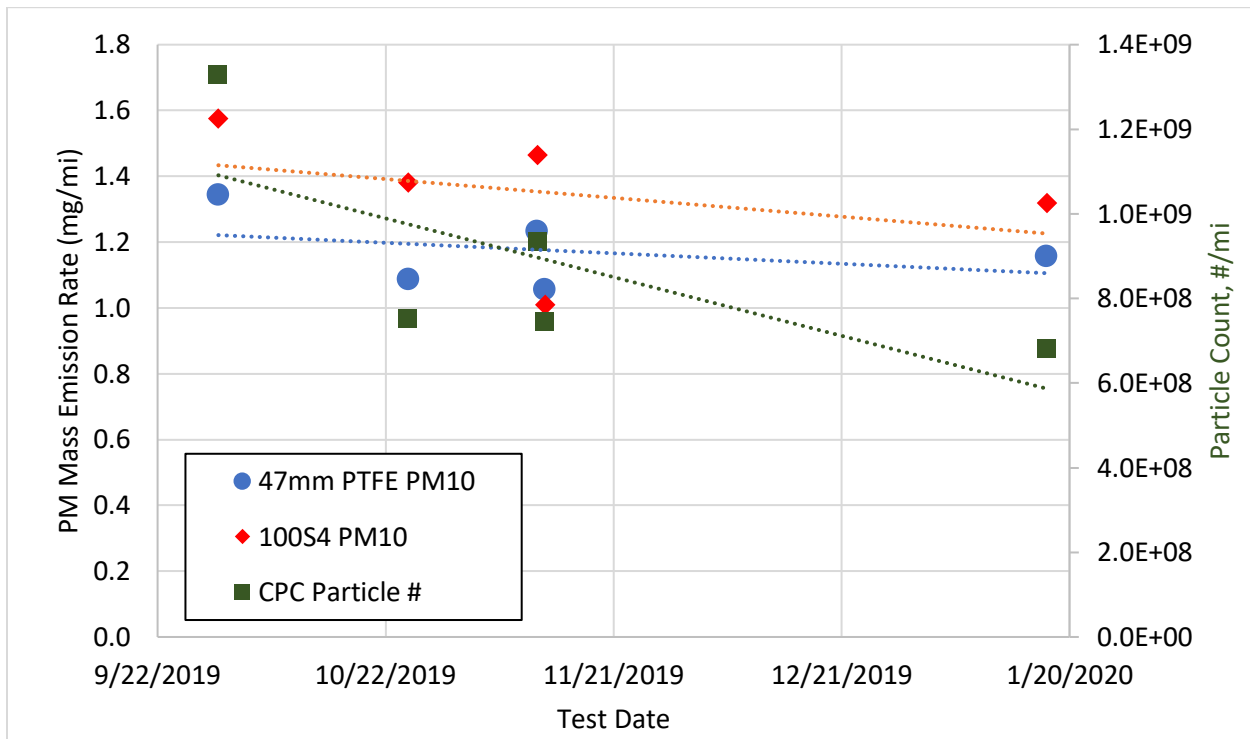
Figure 94. Reference trends by date for the 47mm PTFE and 100S4 PM10 mass measurements (left axis); and CPC particle count (right axis)
