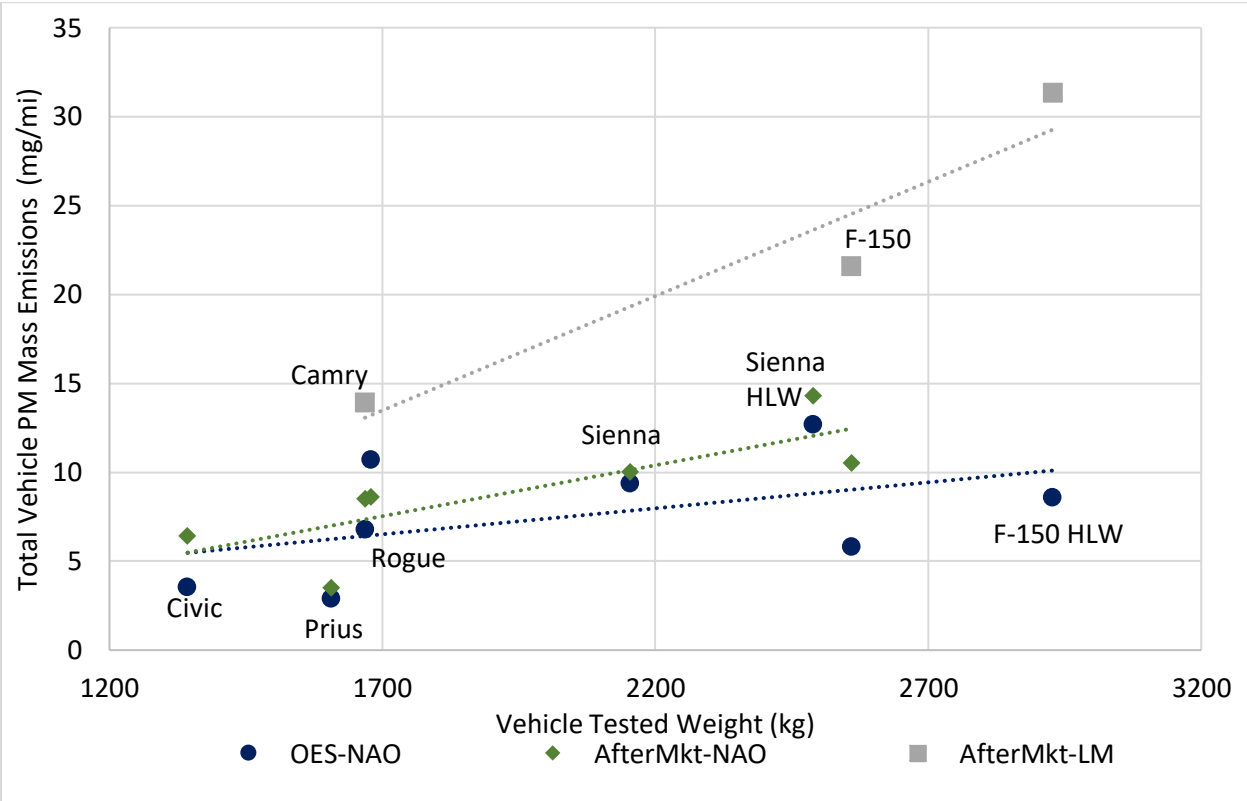
Figure 54. Total vehicle test cycle PM10 mass emissions vs simulated vehicle test weight, categorized by pad material.
