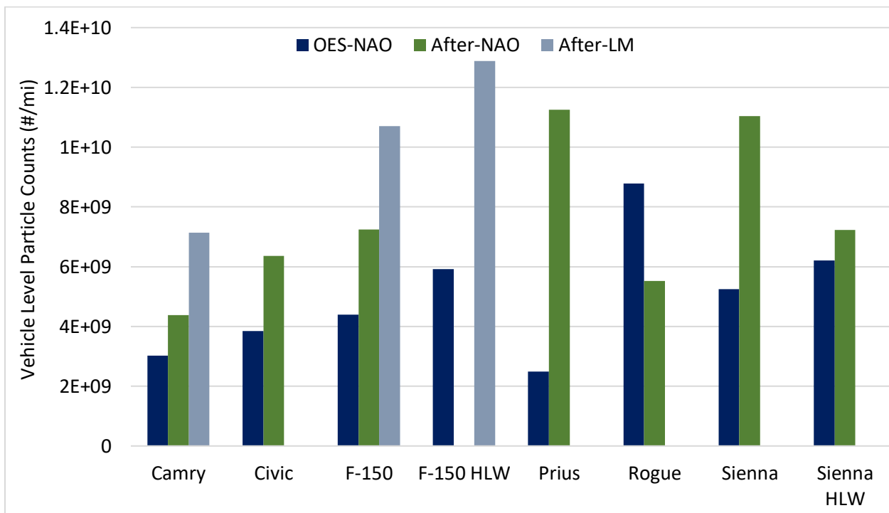
Figure 57. Vehicle-level particle number emission rates for each vehicle and friction material combination
