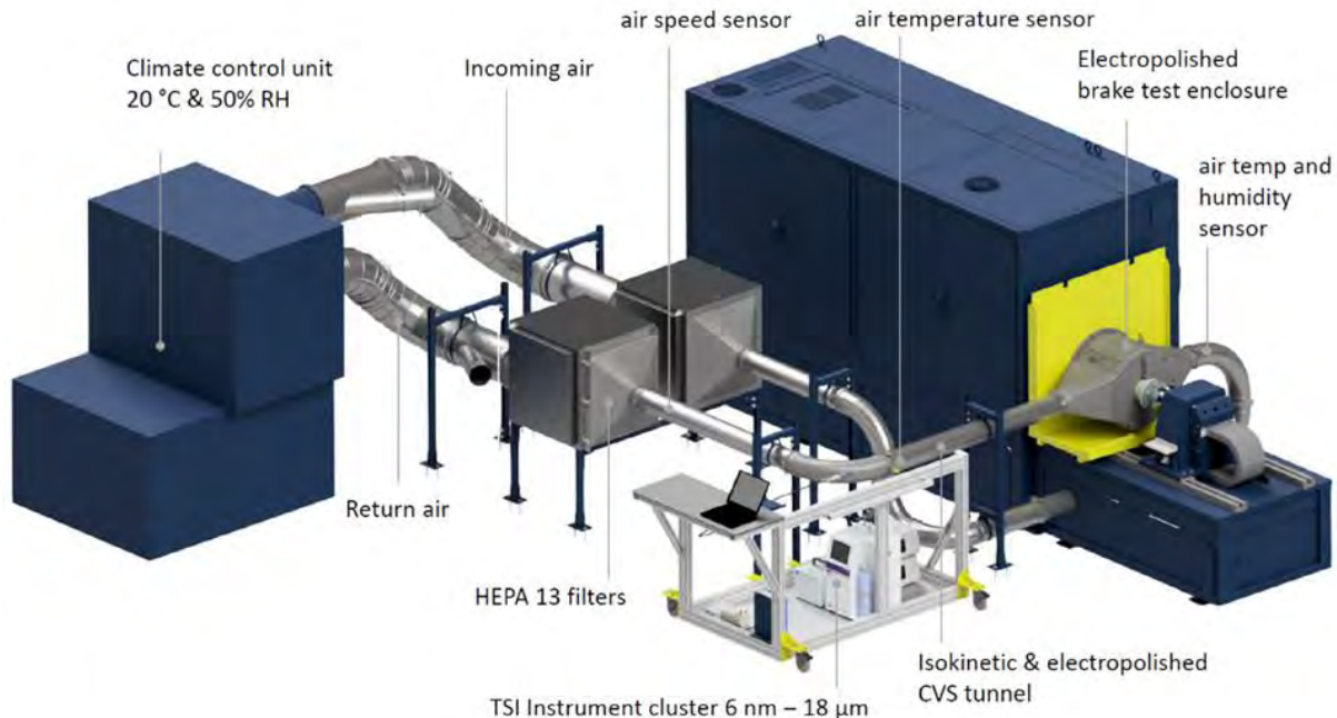
Figure 18. Schematic of LINK Laboratory Setup
