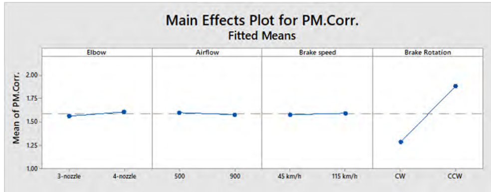
Figure 36. Graphical plot of the PM response to the parameters of the number of sampling nozzles, airflow rate, brake rotational speed, and brake rotational direction during the Arizona dust evaluation
